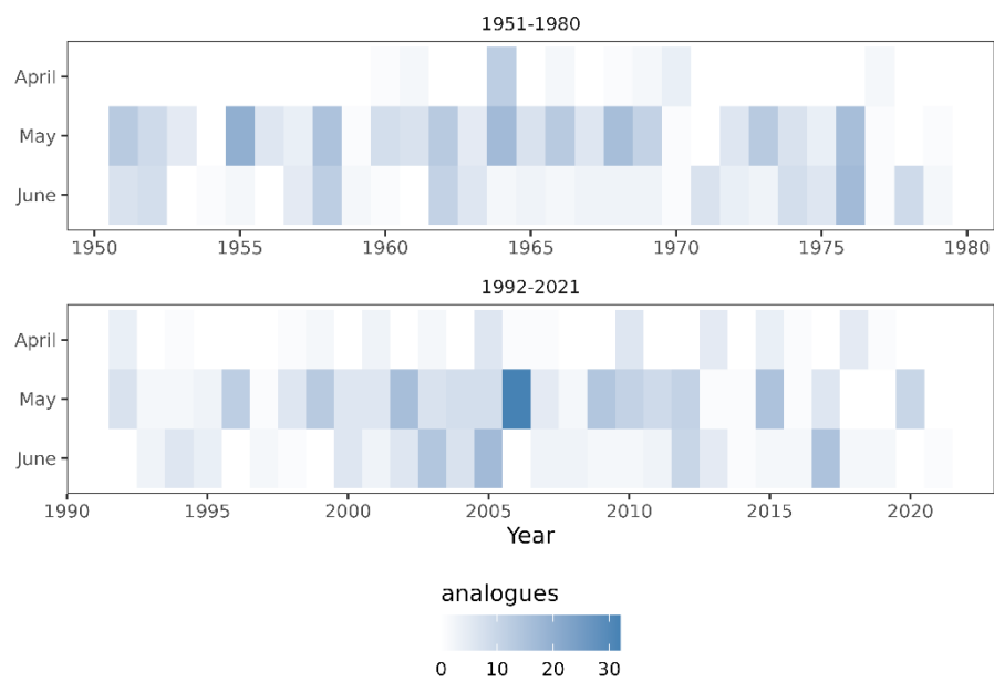
625 Figure A10. Number of analogues of the May 2022 event detected by year.
