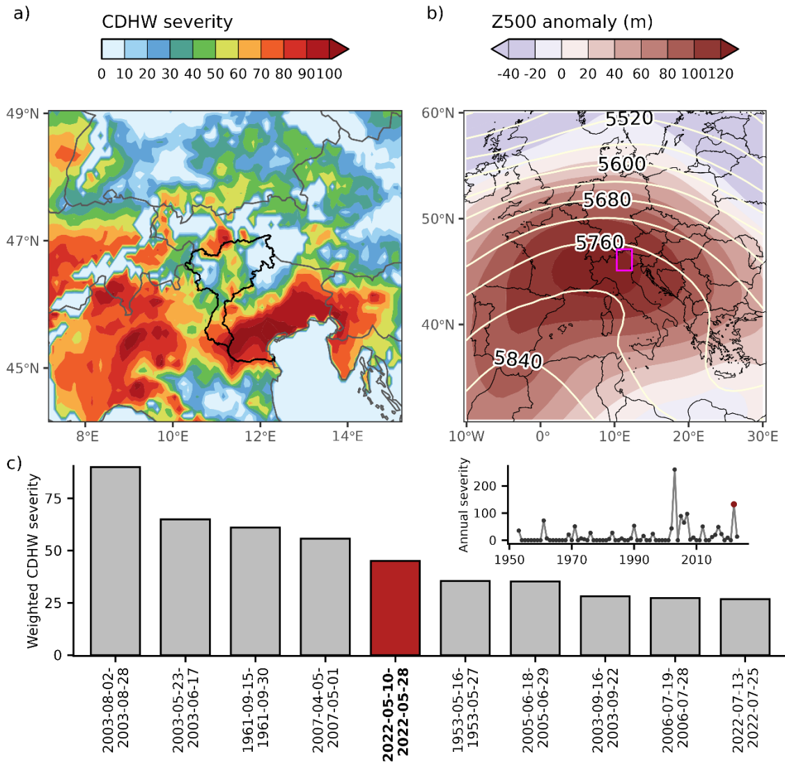
Figure 3. (a) Total severity values derived from the CDHWsev indicator and (b) 500-hPa geopotential height anomalies for the event from 10 to 28 May of 2022. c) Severity-area weighted ranked events for the Adige catchment from 1950 to 2023. The upper-right inset plot in c) shows the annual total severity-area weighted. Event and year 2022 are pointed out in red.
