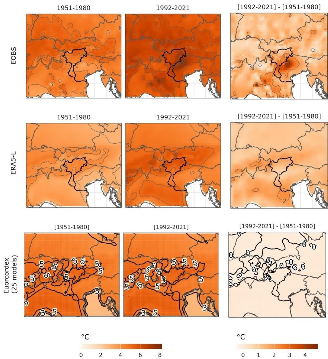
595 Figure A4. Spatial comparison of flow conditioned daily maximum temperature anomalies (TX) reconstructed for the periods 1951–1980 and 1992–2021, and the differences between these periods ([1992–2021] - [1951–1980]), based on three datasets: E-OBS (top row), ERA5-Land (middle row), and EURO-CORDEX ensemble mean (bottom row). The first two columns represent temperature anomalies for the two periods, while the third column shows the difference in anomalies.
