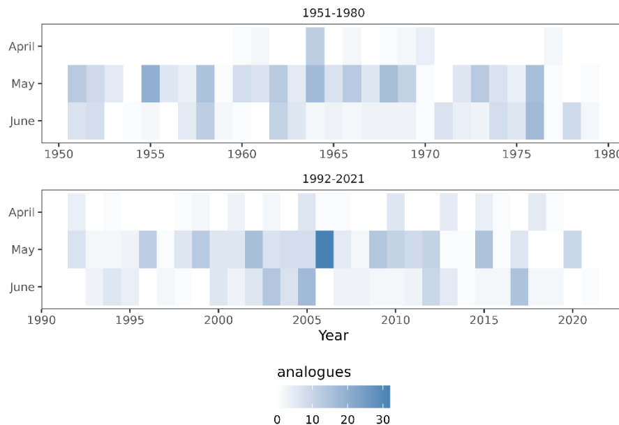
Fig R1. Number of analogues of the May 2022 event detected by year.
