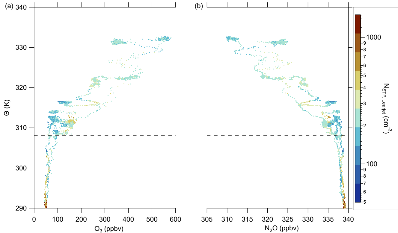
Figure A1. Vertical profiles of \text{O}_3 (a) and \text{N}_2\text{O} (b) for the complete F07, color-coded with the total aerosol number concentration measured by the UHSAS. The dashed lines visualize the chemical tropopause based on the vertical gradient and the mixing ratios of the individual species.
