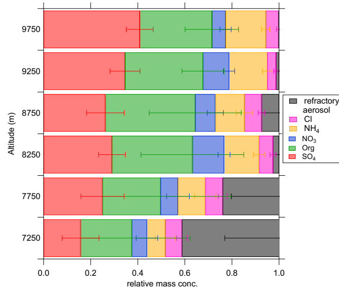
Figure 12. Relative mass concentration for the non-refractory aerosol species (chloride in pink, ammonium in orange, nitrate in blue, organics in green and sulfate in red) and estimated black carbon highest possible refractory aerosol (rA) (black) in 500 m vertical bins between 7 and 10 km. The error bars represent the standard deviation in the altitude bins.
