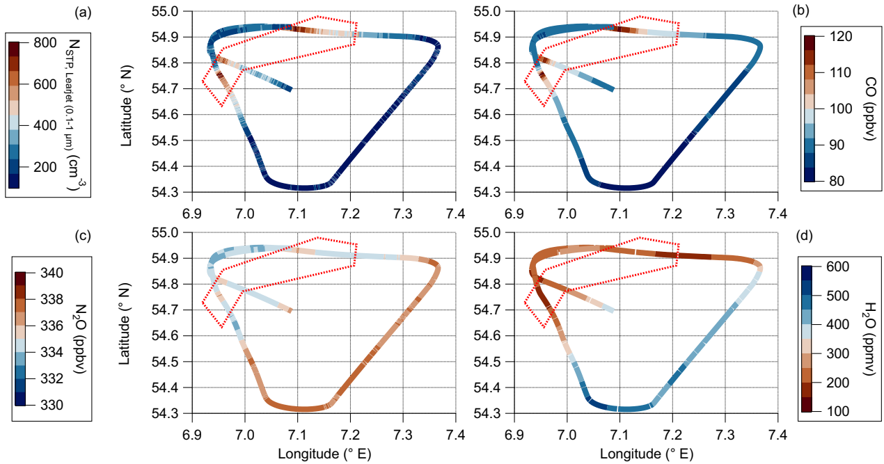
Figure 4. Flight track of the first complete triangular pattern with deployed TOSS-TPC-TOSS within the restricted air space. The pattern is flown at FL240 (approx. 7400m) between 07:24 and 07:47 UTC. The colorcode represents different in-situ measurements of onboard the Learjet : (a) total aerosol number concentration between 100-0.1 and 1 \mu\text{m} , (b) CO, (c) \text{N}_2\text{O} and (d) \text{H}_2\text{O} measurements. The red box surrounds the observed polluted air masses.
