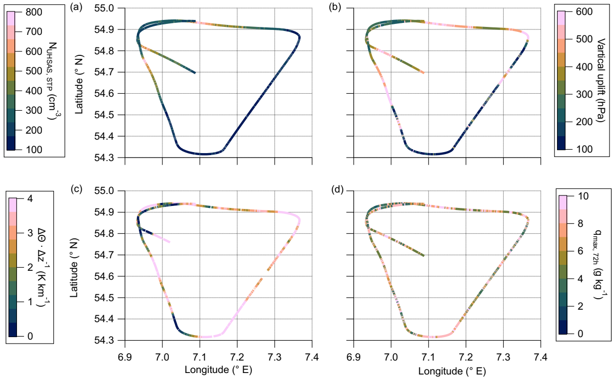
Figure 11. Top view of the first flight pattern within the restricted air space with deployed TOSS-TPC-TOSS during F07. Colorcoded are measured quantities, such as the total aerosol particle number concentration by the UHSAS (a) and the vertical gradient of potential temperature (c). Furthermore, we analyzed meteorological parameters along the trajectories, namely the range between maximum and minimum pressure (b) and the maximum specific humidity over the last 72 h before the measurements (d).
