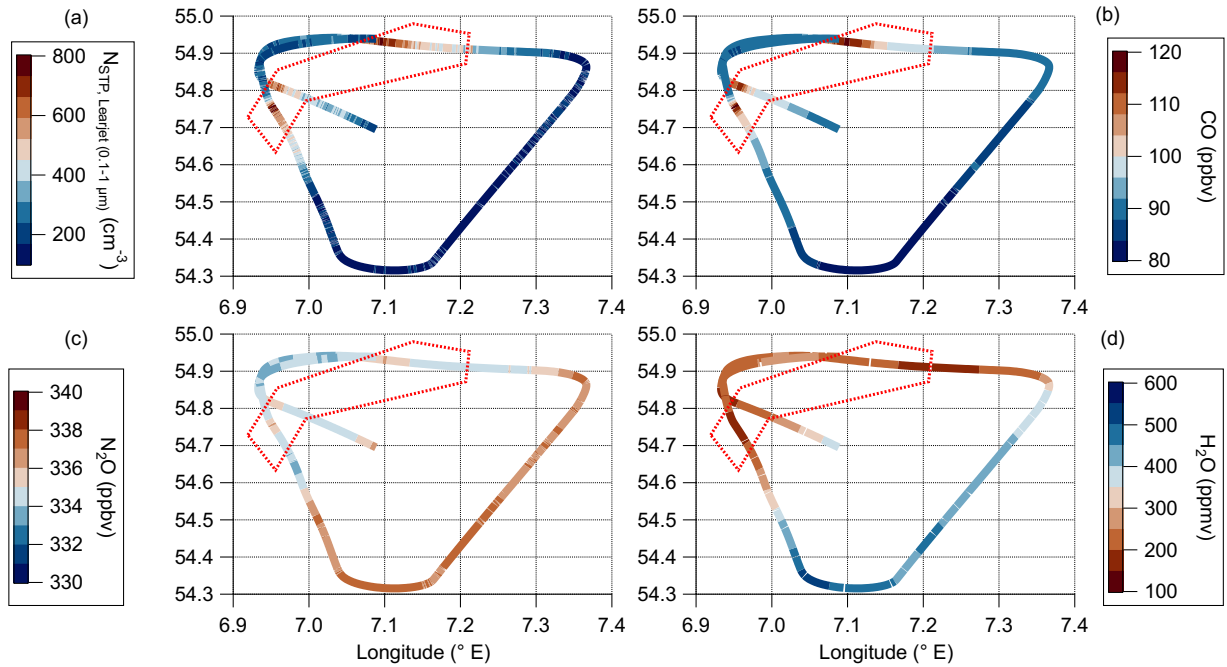
Figure 4. Flight track of the first complete triangular pattern with deployed TOSS-TPC-TOSS within the restricted air space. The pattern is flown at FL240 (approx. 7400m) between 07:24 and 07:47 UTC. The colorcode represents different in-situ measurements of onboard the Learjet : (a) total aerosol number concentration between 100-0.1 and 1 \mu\text{m} , (b) CO, (c) \text{N}_2\text{O} and (d) \text{H}_2\text{O} measurements. The red box surrounds the observed polluted air masses.
