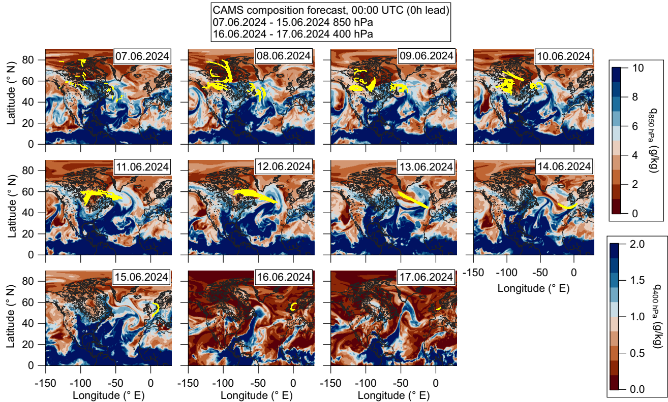
Figure F1. Combination of CAMS forecast data (colored background) and daily split trajectory data (red-yellow lines). All panels show the CAMS forecast with 0 h lead time for specific humidity ( q ) on 850 hPa (a-i) and 400 hPa (j-k). The trajectories are split for each 24 h interval to identify the large-scale context of the trajectories.
