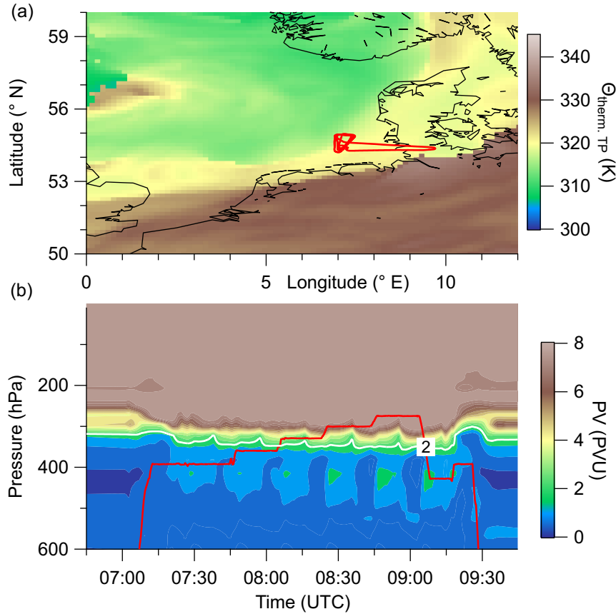
Figure 1. ECWMF forecast data for 17 June 2024, 06 UTC (F07). The potential temperature along the thermal WMO tropopause and the flight path of F07 ( black-red solid line) are shown in panel (a). Panel (b) shows a vertical cross-section of potential vorticity (PV) along the flightpath ( black-red solid line) with the 2 PVU surface as marker for the dynamical tropopause in the model (white solid line).
