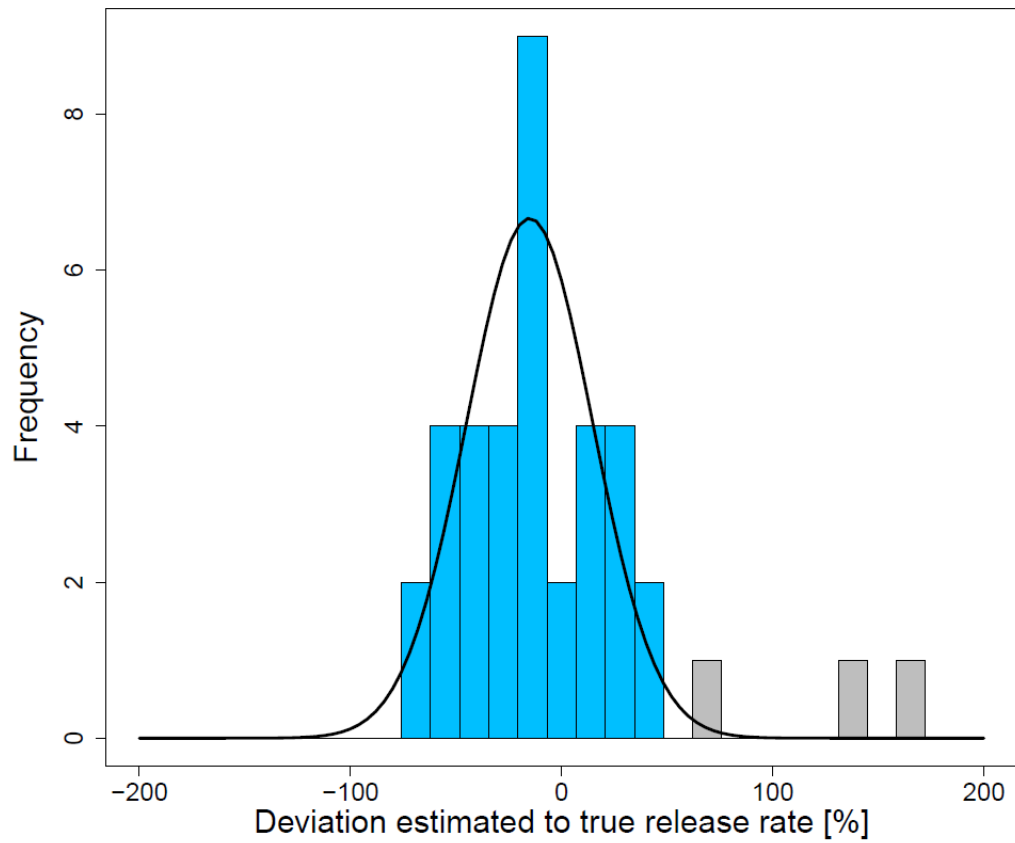
Figure S12. Histogram illustrating the distribution of mean estimated emission rates relative to the actual release rate across all six controlled release experiments conducted between 2018 and 2023. The black curve represents the normal distribution of the data, calculated using the mean and standard deviation. Grey data represent measurements at a distance of 14 m between air inlet and release source and are excluded from the normal distribution.
