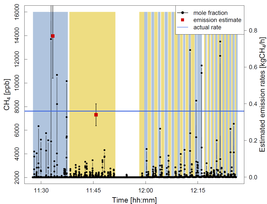
Figure S8. Controlled release experiment MA3 time series with CH 4 mole fraction measured at different distances highlighted (blue =14 m, yellow =36 m) and determined emission rates in comparison to actual release rate for the different distances.
