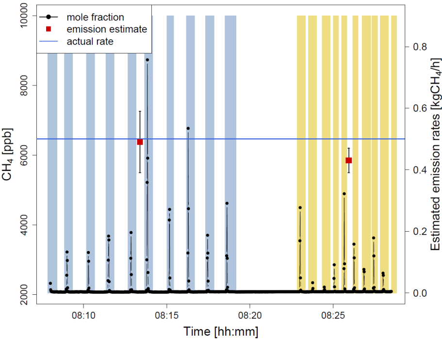
Figure S5. Time series with CH 4 mole fraction measured at different vehicle speeds highlighted (blue= 20 km h -1 ; yellow= 50 km h -1 ) with estimated release rates for the both driving speeds.
