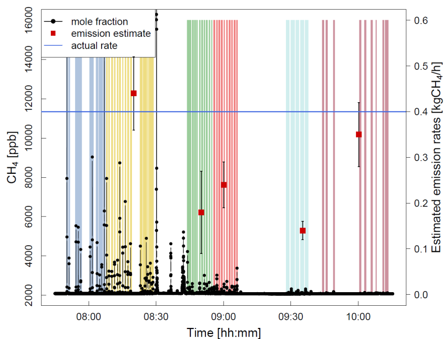
Figure S9. Controlled release experiment HD2 time series with CH 4 mole fraction measured at different distances highlighted blue (4 m), yellow (25 m), green (50 m), light red (70 m) light blue (120 m) and red (260 m) and determined emission rates in comparison to actual release rate for different distances.
