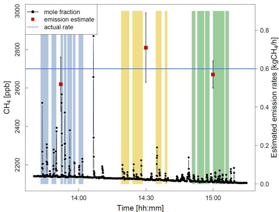
Figure S7. Time series with CH 4 mole fraction measured at different distances highlighted (blue = 100 m, yellow = 250 m, green = 310 m) and determined emission rates in comparison to actual release rate for the three different distances.
