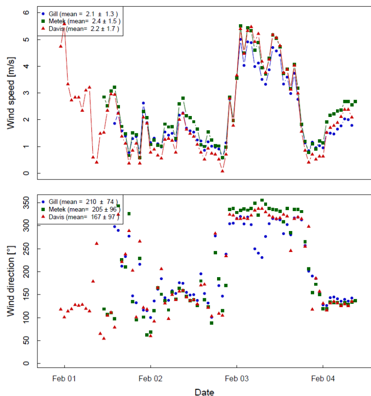
Figure S10. Wind speed (top) and wind direction (bottom) measured with the Gill (blue), Metek (green) and Davis (red) instruments installed stationary on the institute roof averaged hourly (February 2019).
