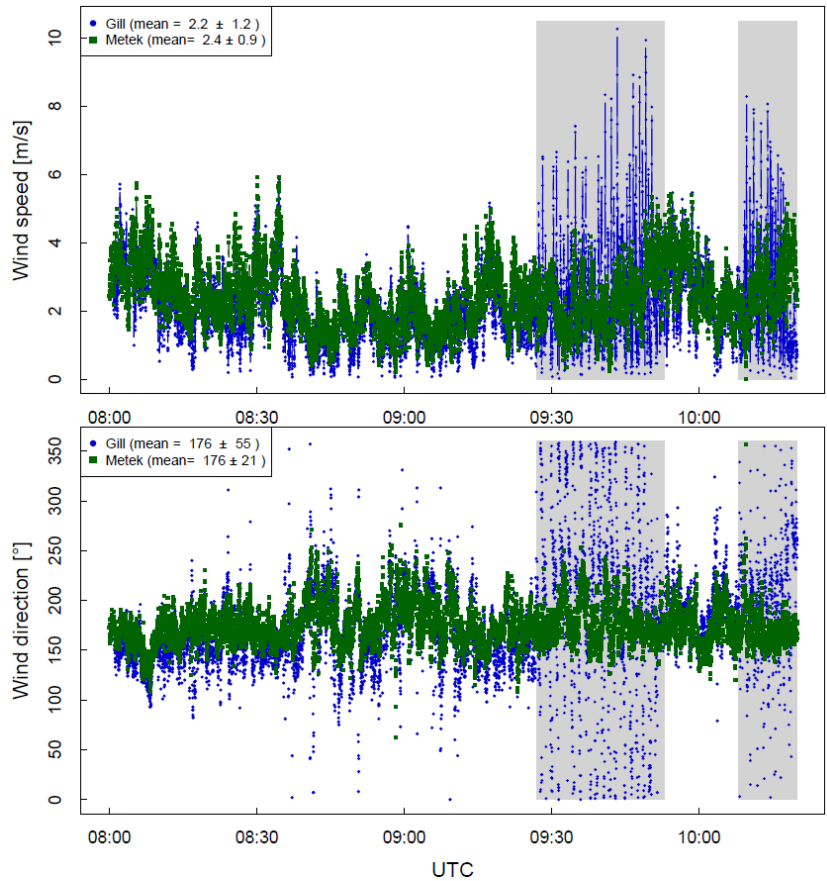
Figure 5. Wind speed (top) and wind direction (bottom) measured with the mobile (Gill) and stationary (Metek) instruments during the HD3 release experiment (October 2023). The grey areas highlight the periods when the car was driving.
