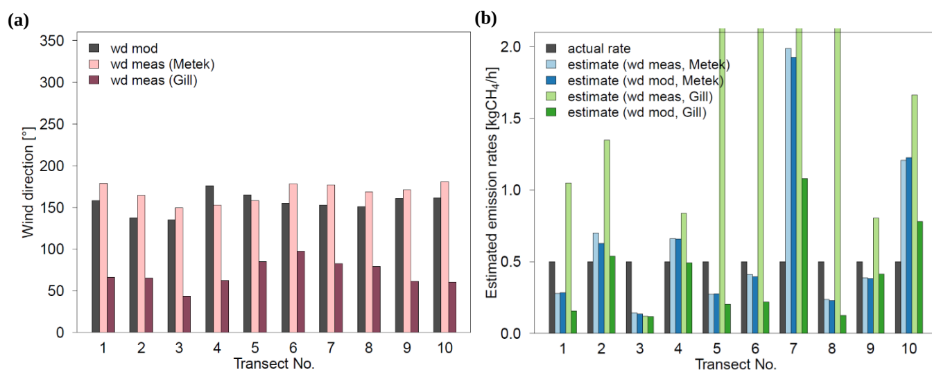
Figure 6. (a) Measured wind direction for the Metek (pink) and Gill (purple) instruments in comparison with the modelled wind direction shown in grey for 10 transects during the HD1 release experiment. (b) Bar plot showing the corresponding emission rates calculated via the measured and modelled wind directions for the Metek and Gill instruments, respectively, compared with the actual release rates.
