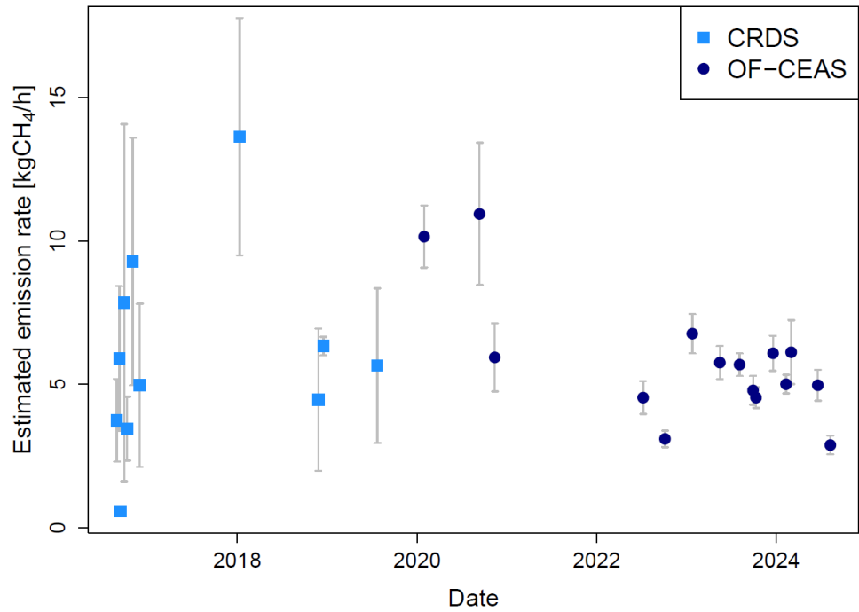
440 Figure 8. Harmonized dataset of the estimated mean CH 4 emission rates at a biogas plant for each measurement day between 2016 and 2024, calculated using the GPM. Emission rate values before 2020 in light blue are based on measurements performed with a CRDS trace gas analyser, and measurements after 2020 were performed via an OF-CEAS instrument with an adapted driving strategy. Note: The error bar for one CRDS-based CH 4 emission estimate is present but very small, making it difficult to distinguish visually in the figure.
