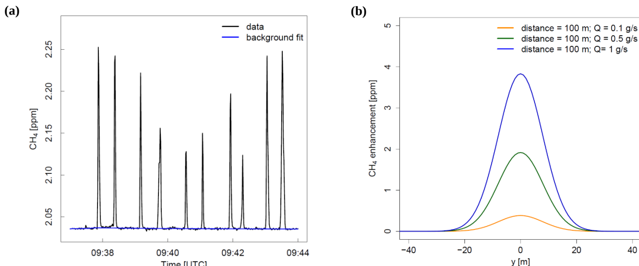
Figure 2. (a) Measured CH 4 mole fraction (ppm) against time (hh:mm) during emission plume crossings recorded with the LI-7810 trace gas analyser. The calculated background mole fraction is highlighted in blue. (b) Model cross sections of the GPM during CH 4 plume crossing downwind of the source at a distance of x = 100 m with different input emission rates (blue, Q = 1 \text{ g CH}_4 \text{ s}^{-1} ; green, Q = 0.5 \text{ g CH}_4 \text{ s}^{-1} ; yellow, Q = 0.1 \text{ g CH}_4 \text{ s}^{-1} ).
