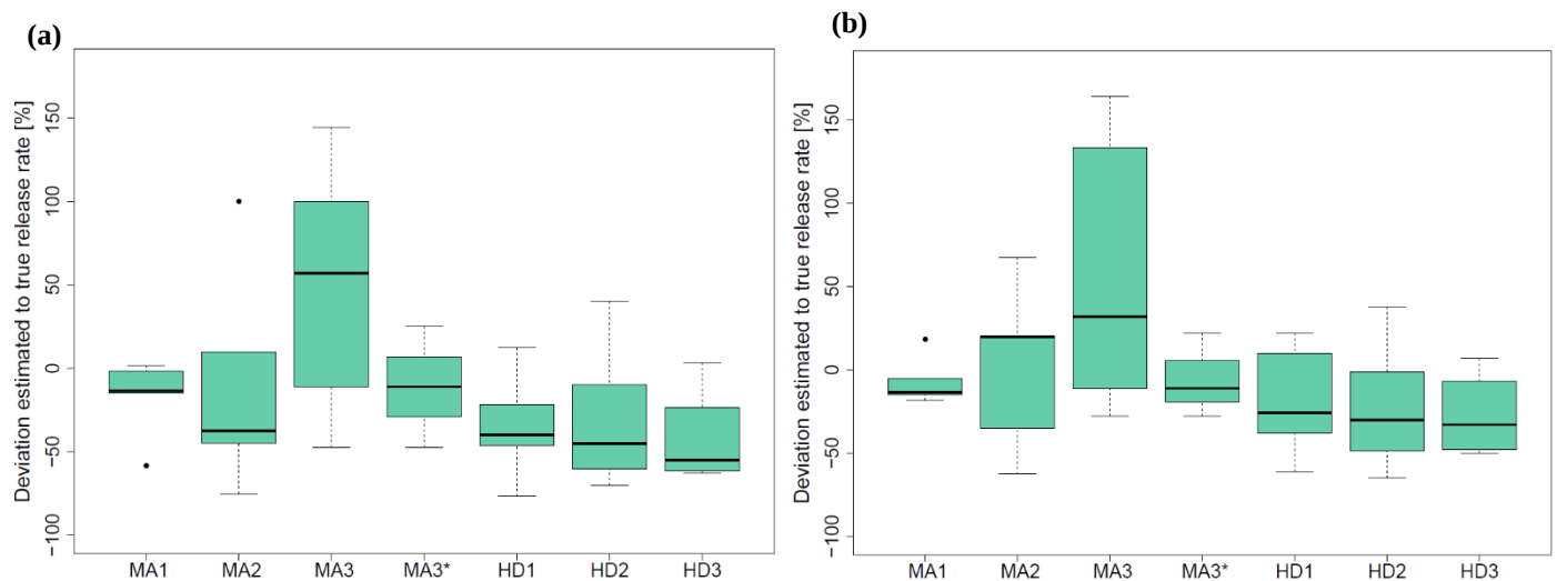
Figure 4: Boxplot for the comparison of the determined methane emission rates during the different release experiments to the actual release rates for (a) median and (b) mean values. The boxplots show the first and third quartiles of the data, whereas the whiskers extend to the largest value that remains within 1.5 times the interquartile range. Release experiment MA3 is split into MA3, which includes all release processes, and MA3*, which excludes release processes at a 14-m distance.
