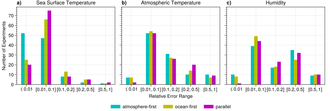
Figure 8. Weighted error e_j/e_{\max} for the two-day TOP experiments where SWR terminated, grouped by coupling scheme.
