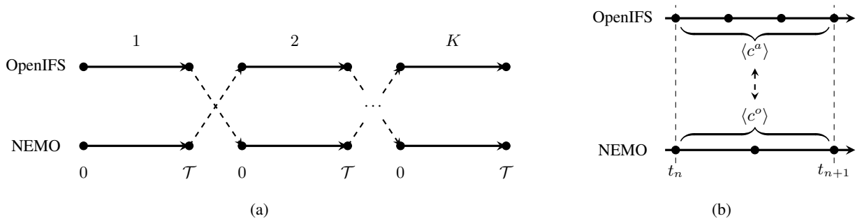
Figure 3. SWR for two subdomains depicted by the data dependency across iterations (a) and in the converged limit (b). Solid arrows depict integration in time. Dashed arrows represent communication of information between iterations.
