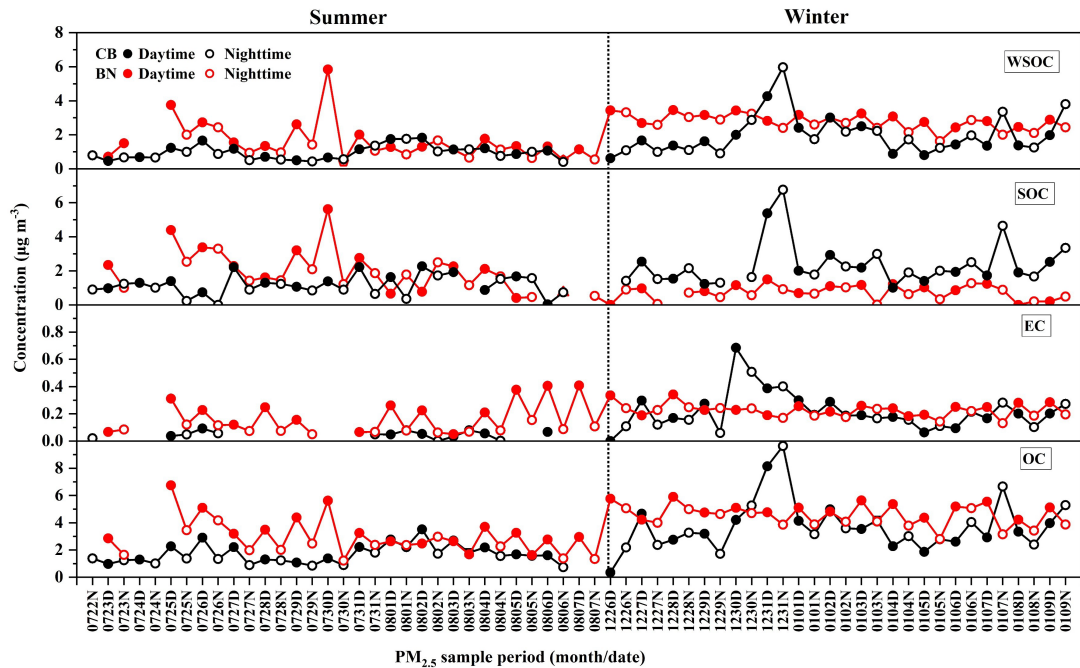
Figure 7: Temporal variations in the concentrations of OC, EC, WSOC, and SOC in \text{PM}_{2.5} collected from CB and BN, China during 2023-24.
