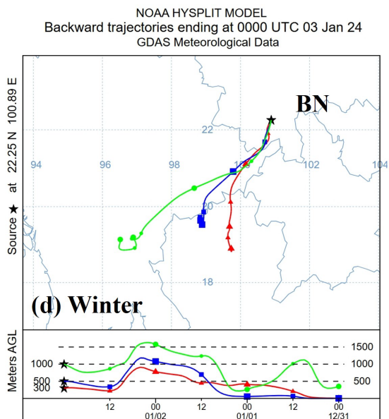
Figure 1: Clustered 72-hour backward airmass trajectories plots (above the ground level: 300 m, 500 m, and 1000 m) at CB and BN, China during 2023-24.
