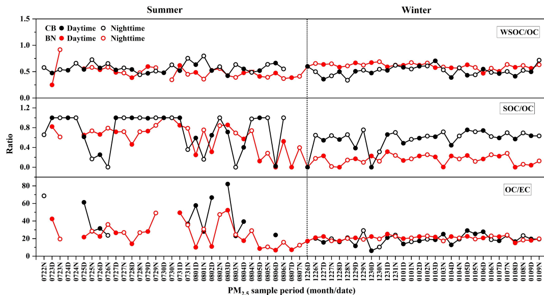
360 Figure 13: Temporal variations of OC/EC, WSOC/OC and SOC/OC in PM 2.5 collected from CB and BN, China during 2023-24.
