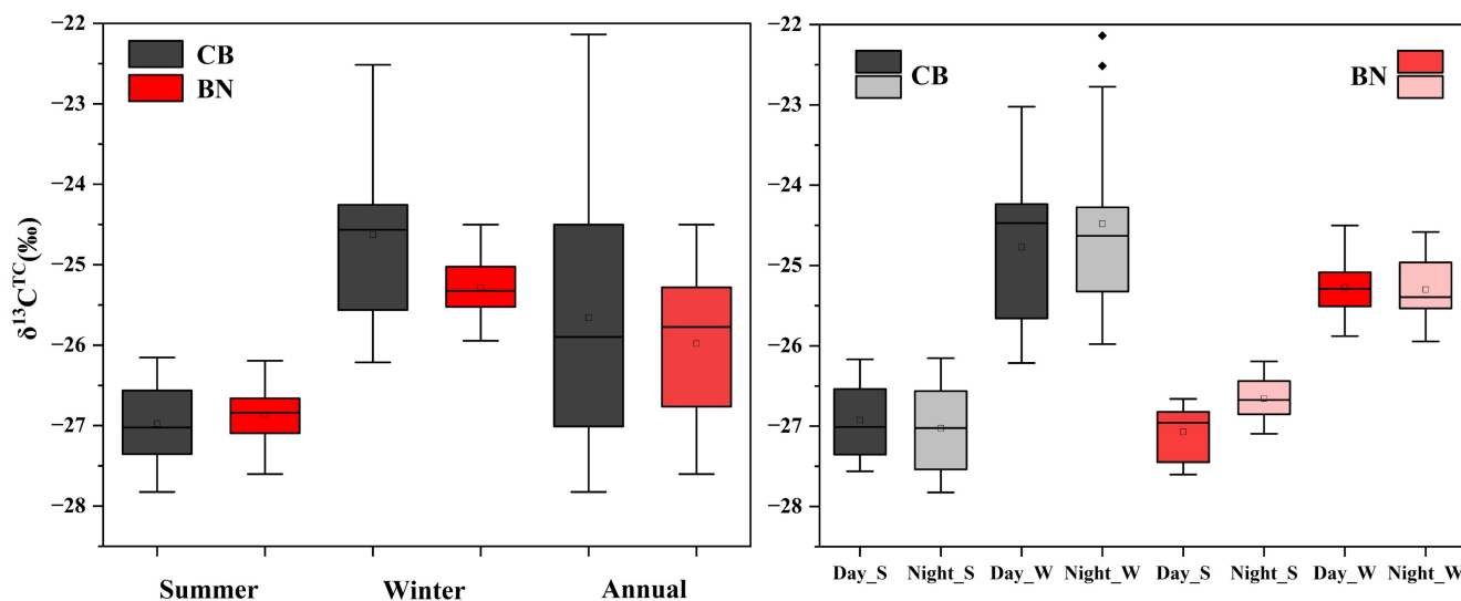
260 Figure 9: Seasonal and diurnal variations of \delta^{13}\text{C}_{\text{TC}} collected from CB and BN during the campaign. The S and W represent summer and winter, respectively.
