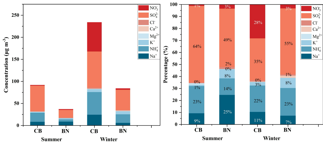
215 Figure 5: Concentrations and percentages of WSII in total ions.
