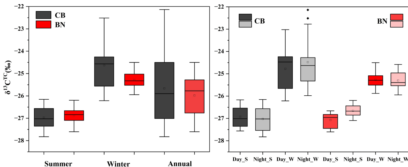
Figure 10: Seasonal and diurnal variations of \delta^{13}C_{TC} collected from CB and BN during the campaign. The S and W represent summer and winter, respectively.
