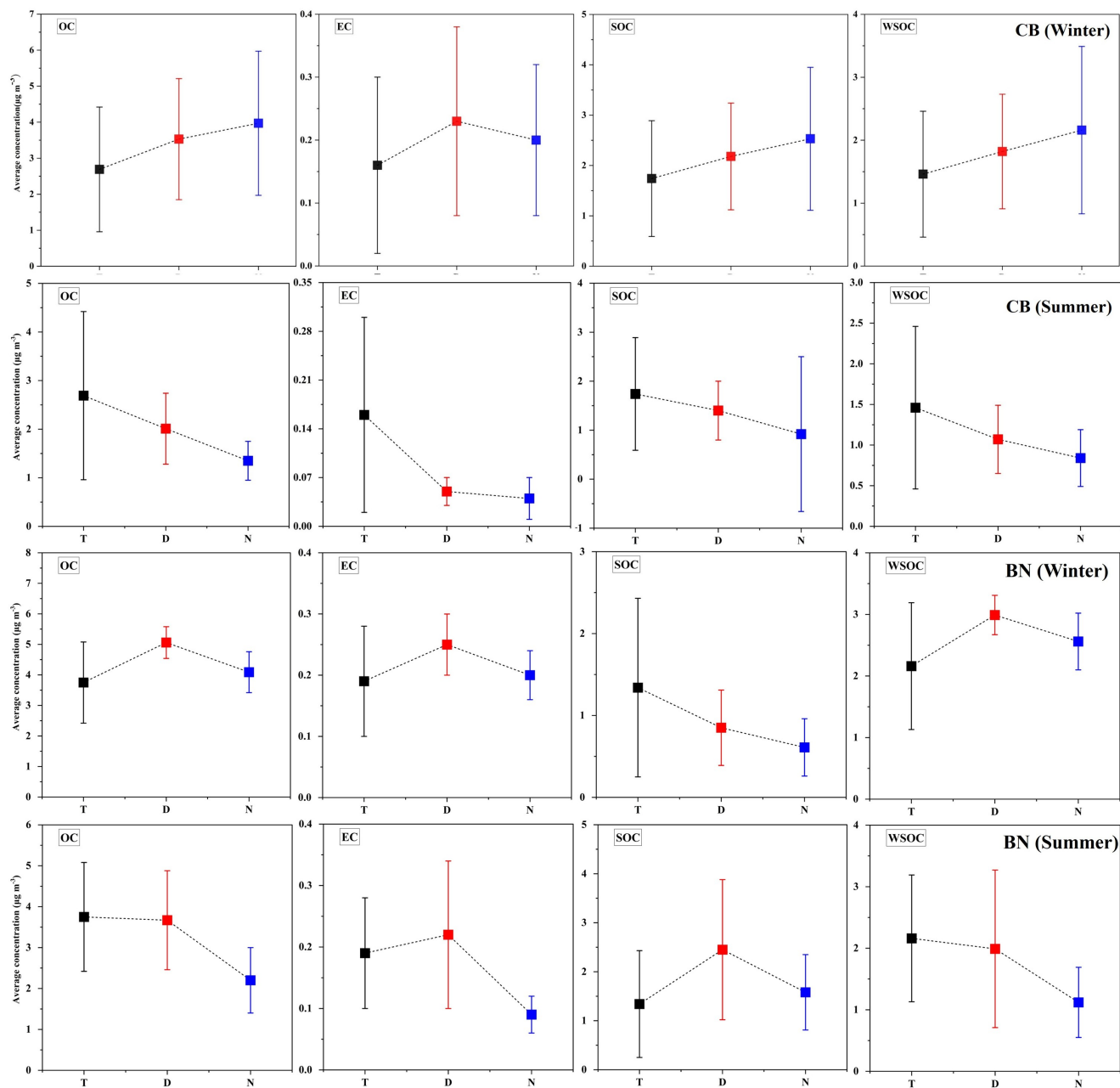
260 Figure 9: Diurnal variations in carbonaceous components in summer and winter forest aerosol samples collected from CB and BN, China during 2023-24. The black, red and blue squares represent the average concentrations of total (T), daytime (D) and nighttime (N).
