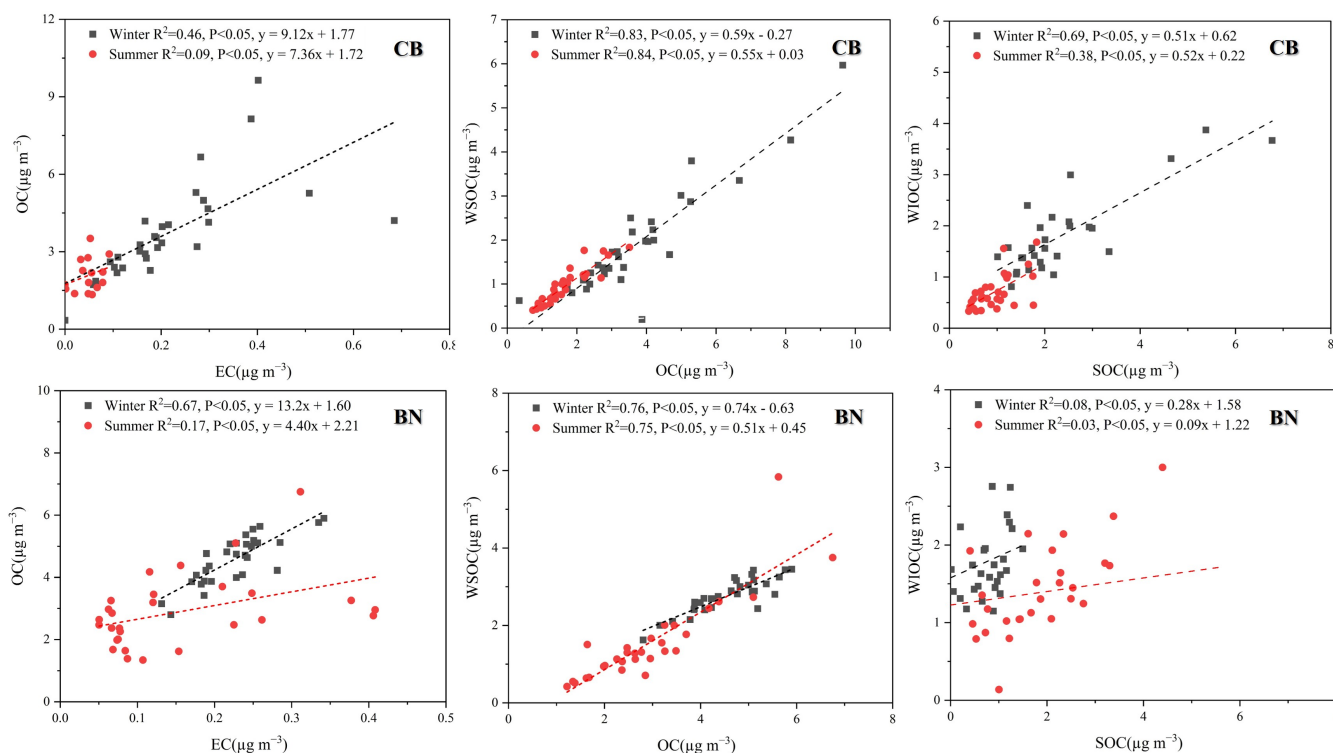
Figure 13: Correlations of certain carbonaceous components in PM 2.5 collected from CB and BN, China during 2023-24.
