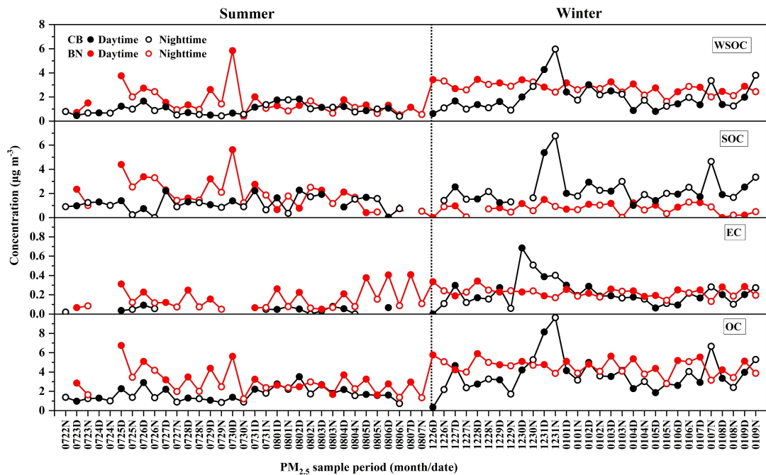
Figure 8: Temporal variations in the concentrations of OC, EC, WSOC, and SOC in \text{PM}_{2.5} collected from CB and BN, China during 2023-24.
