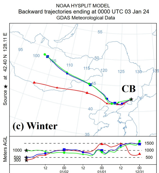
Figure 2: Clustered 72-hour backward airmass trajectories plots (above the ground level: 300 m, 500 m, and 1000 m) at CB and BN, China during 2023-24.
