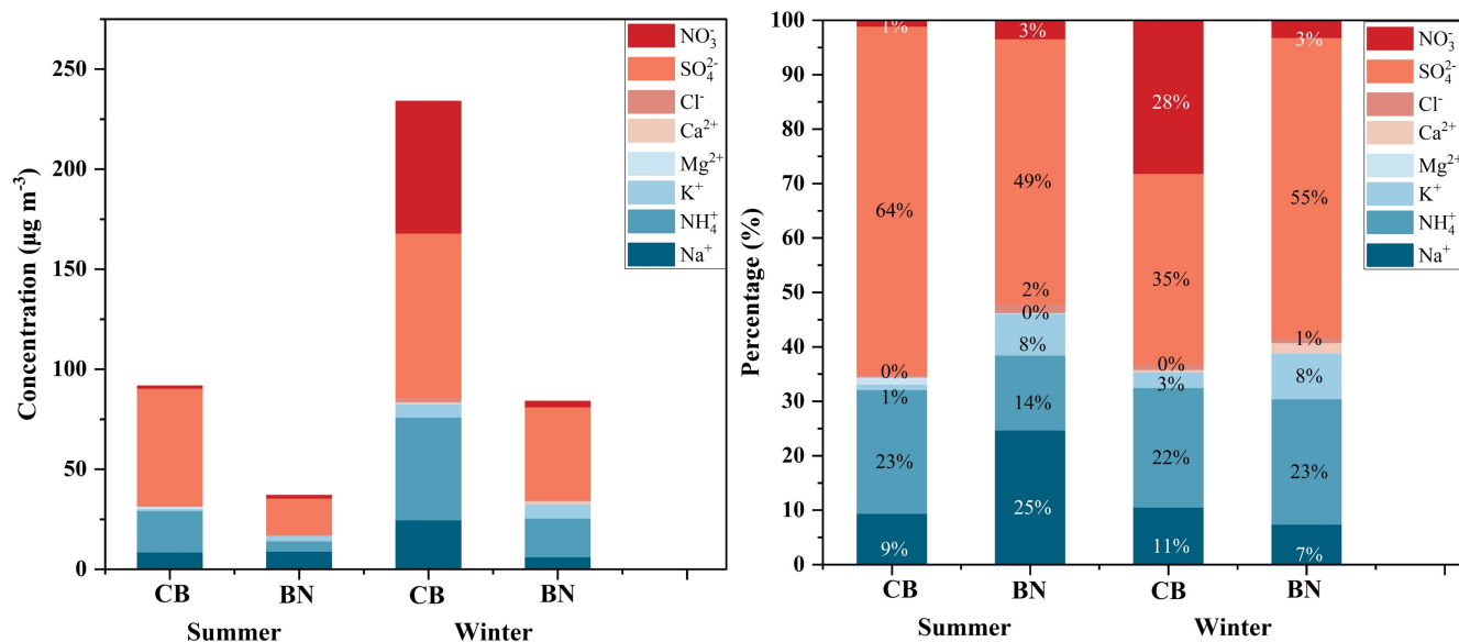
Figure 6: Concentrations and percentages of WSII in total ions.
