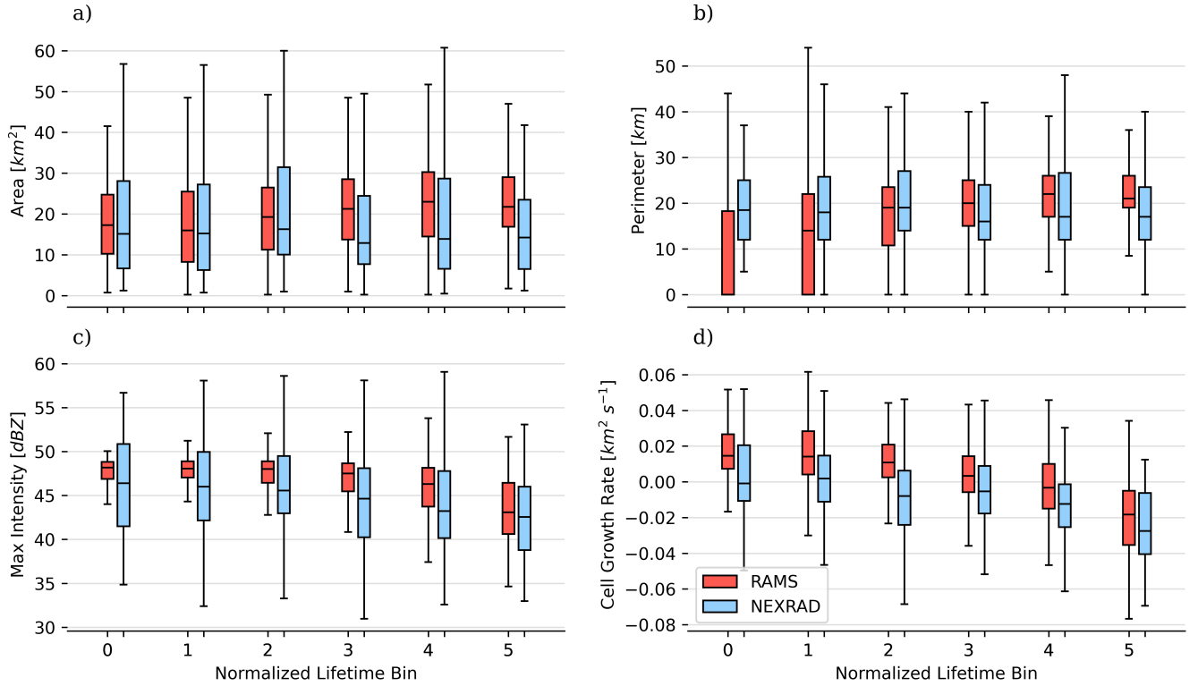
Figure 8. Box-whisker plot of tracked cell properties (both observed [NEXRAD] and simulated [RAMS]) as a function of the normalized lifetime bin. Only cells that last longer than 40 minutes and do not experience merging during their lifetime are included. 0 represents the first identification of the cell, and 5 indicates the termination of the tracked cell. Note that the unit of lifetime is in time units of minutes. The normalized lifetime is a unitless measurement.
