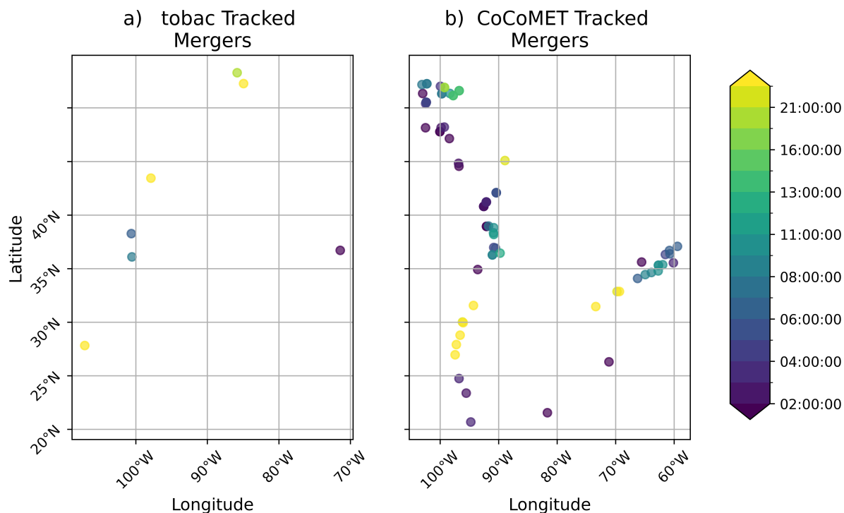
Figure C2. Same as Figure C1, but For CoCoMET: touching_threshold = 0.15, score_weight_1 = 1, overlap_threshold = 0.2. For tobac: merge_dist = 25 (100 km), frame_len = 3 (3 hours).
