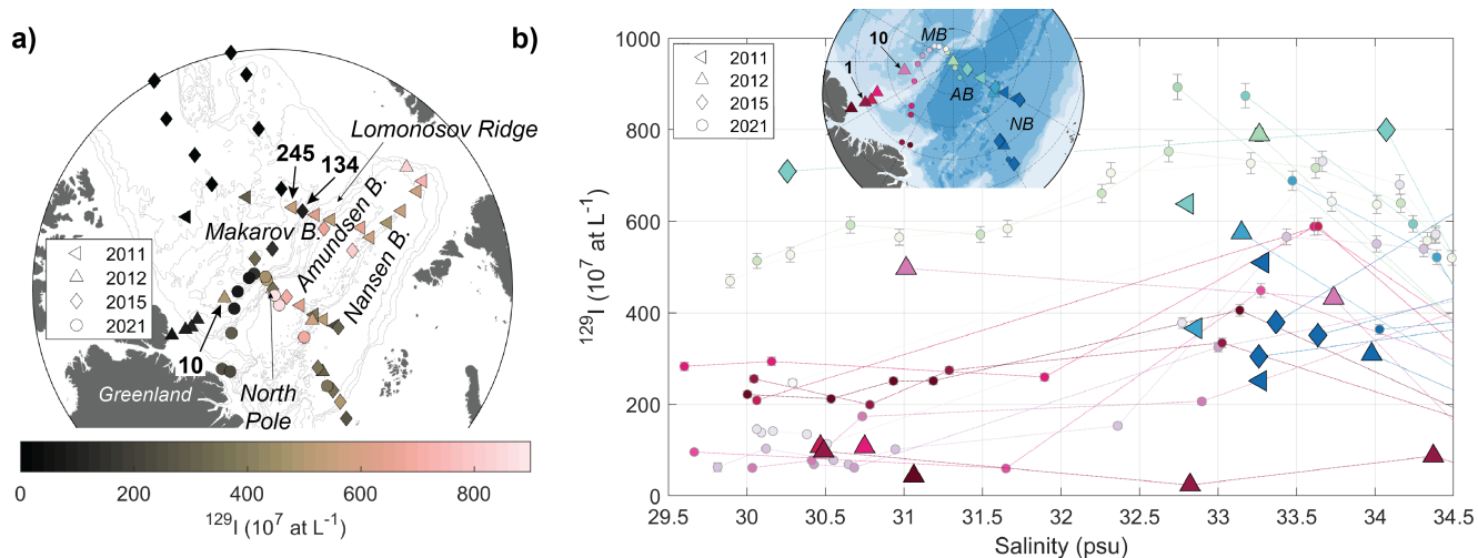
Figure 6. (a) Isosurface map of ^{129}\text{I} concentrations in the surface ( < 15 m depth for 2011, 2015, 2021; 25 m depth for 2012 due to sampling depth resolution). (b) Plot of ^{129}\text{I} concentration against practical salinity for available stations from 2011, 2012, 2015, 2021. The 2021 data is the same as in Fig. 5c. Stations are color-coded by region, following the color-coding for SAS2021 stations.
