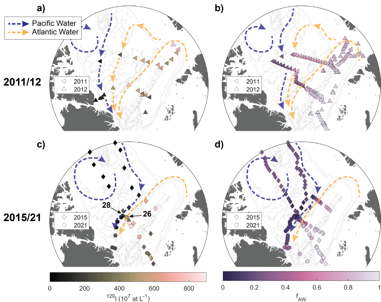
Figure 11. (a) Isosurface map of ^{129}\text{I} concentrations in the surface in 2011 and 2012 (< 15 m depth for 2011 25 m depth for 2012 due to sampling depth resolution). (b) Isosurface map of Atlantic Water fractions ( f_{\text{AW}} ) derived from salinity and N:P ratios, for all available data from the surface layer from the same expeditions as in (a). (c) Isosurface map of ^{129}\text{I} concentrations in the surface in 2015/2021 (< 15 m depth). Stations 26 and 28 from SAS2021 are highlighted. (d) Isosurface map of Atlantic Water fractions ( f_{\text{AW}} ) derived from salinity and N:P ratios, for all available data from the surface layer from the same expeditions as in (c). In all panels, the circulation of Atlantic- and Pacific-derived surface waters (yellow and blue, respectively) is sketched based on the corresponding tracer distribution (a & c) or derived water mass fraction (b & d).
