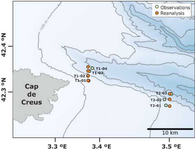
1043 Figure A1. Spatial distribution of CTD stations (green dots) across the Cap de Creus Canyon during the FARDWO-CCC1 1044 cruise where dense shelf waters were observed, and the corresponding MedSea reanalysis grid points (orange dots). Reanalysis 1045 data were obtained from the Mediterranean Sea Physics Reanalysis product (Escudier et al., 2020; 2021).
