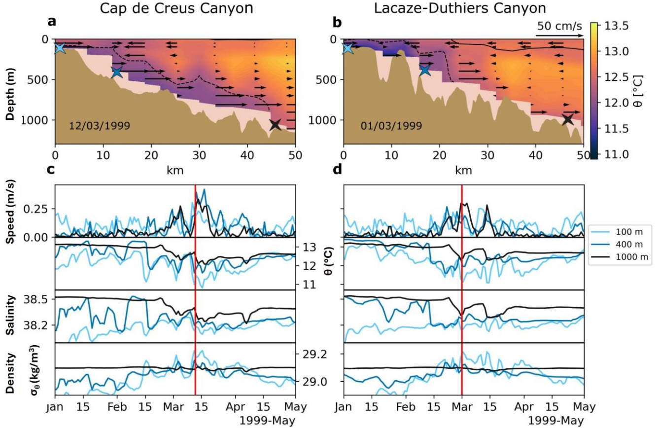
Figure 4. (a-b) IDSWC in 1999 in CCC and LDC from reanalysis. The black dashed line marks the 29.1 \text{ kg/m}^3 isopycnal, and the solid black line, the 29.0 \text{ kg/m}^3 isopycnal. Black vectors show downcanyon flow. Blue crosses mark the canyon bottom locations shown in c and d. The bathymetry corresponds to the reanalysis section represented with a grey line in Figure 1. (c-d) Time series of current speed, potential temperature, salinity and potential density. The red vertical line marks the date shown in a and b.
