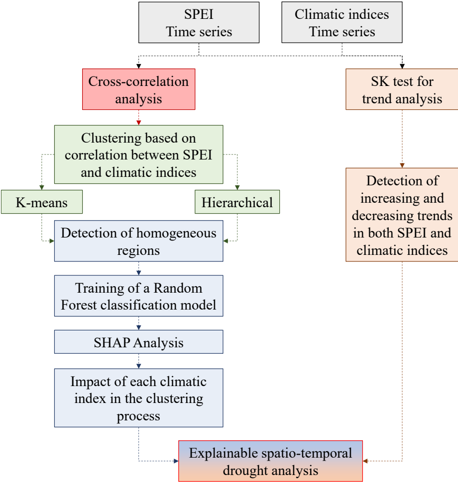
Figure 2: Modeling procedure.
