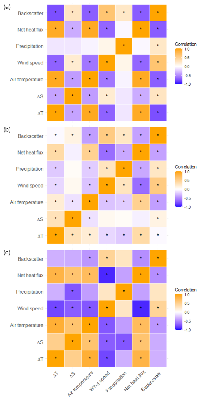
420 | Figure 7: Correlation heat map after the Pearson correlation analysis from (a) the harbour event on 14 March 2023, (b) the harbour events on 15 March 2023, and (c) the North Sea event on 10 October 2022. Each cell represents the correlation strength and direction between two variables, with different colours indicating the degree of correlation: warm colours (orange) for positive and cold colours (blue) for negative correlations. The colour intensity reflects the magnitude of the correlation, ranging from -1 (strong negative correlation) to +1 (strong positive correlation). Significant correlations ( p < 0.05 ) are annotated with an asterisk.
