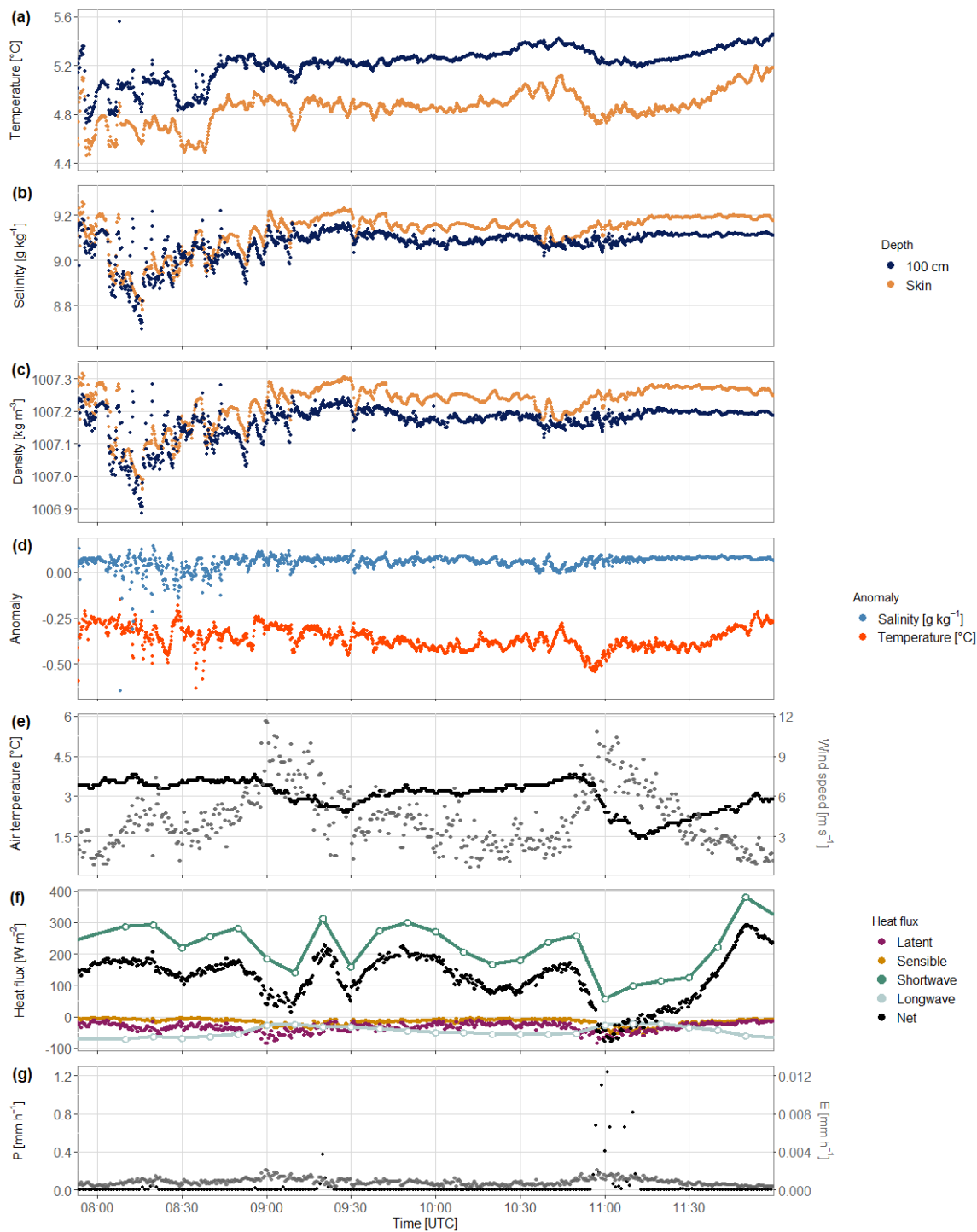
295 Figure 3: Time series of (a) sea surface temperature, (b) sea surface salinity, (c) sea surface density, (d) temperature and salinity anomaly, (e) air temperature and wind speed, (f) heat flux components, (g) precipitation (P) and evaporation (E) rates on 15 March 2023.
