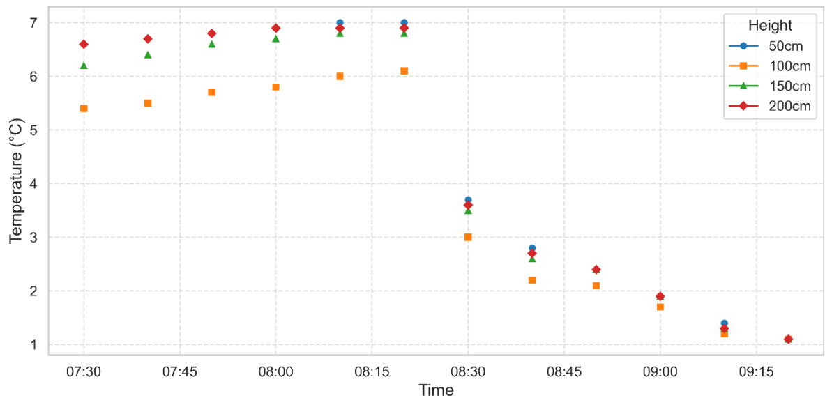
Dew temperature on 14.03.2023 at several heights above the sea surface.
