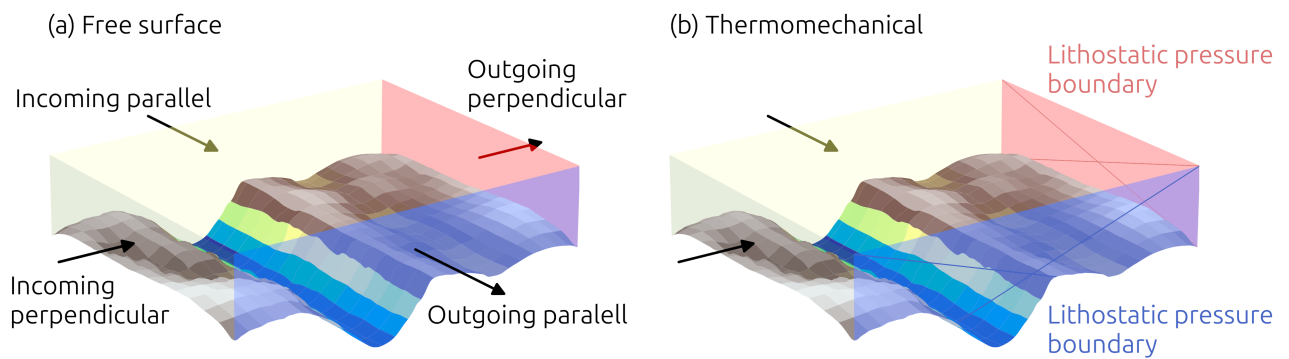
Figure A1. The incoming and outgoing boundaries for the two simulation steps (a) Free surface stage and (b) Thermomechanically coupled stage. Illustrated parallel flow direction and boundary does not represent simulated orientation.
