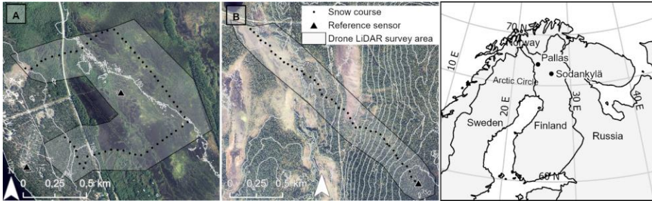
Figure 1. The location and maps of study sites (a) Sodankylä and (b) Pallas. The gray area represents UAV-flight areas, and the black points mark the manual snow sampling locations and of the snow courses. Orthophoto were obtained from the National Land Survey of Finland.
