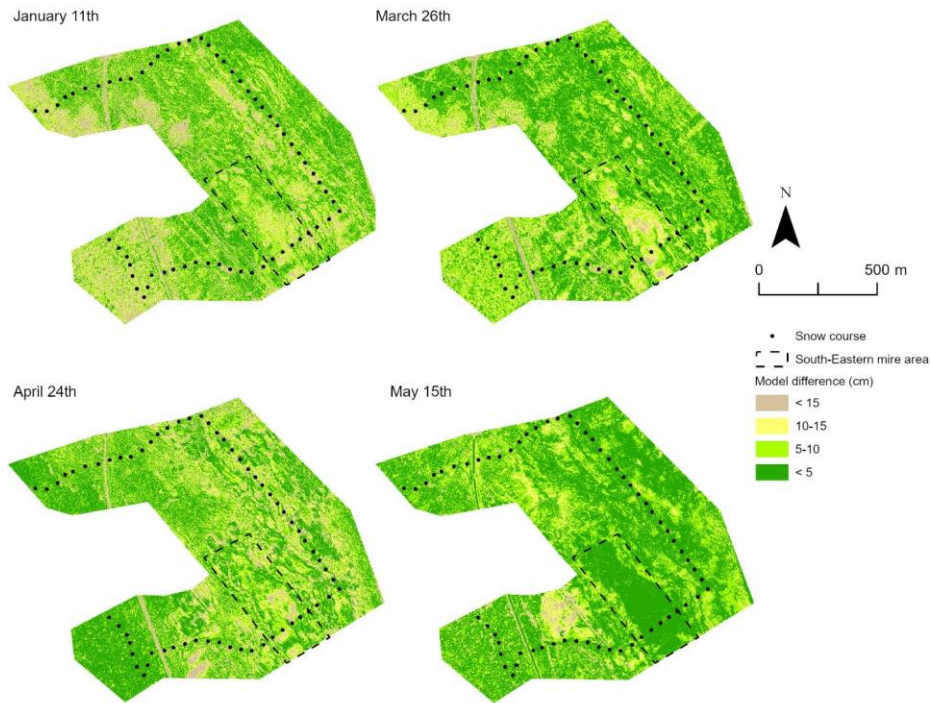
Figure 10. Sodankylä model performance from different UAV LiDAR UAV-campaigns. The values define the absolute difference between LiDAR based snow depth maps and the modelled snow depth maps.
