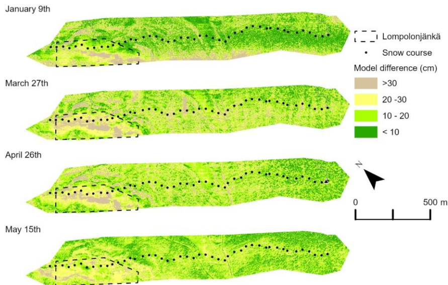
Figure 11 Pallas model performance from different UAV LiDAR UAV campaigns. The values define the absolute difference between UAV LiDAR snow depth maps and the model output.
