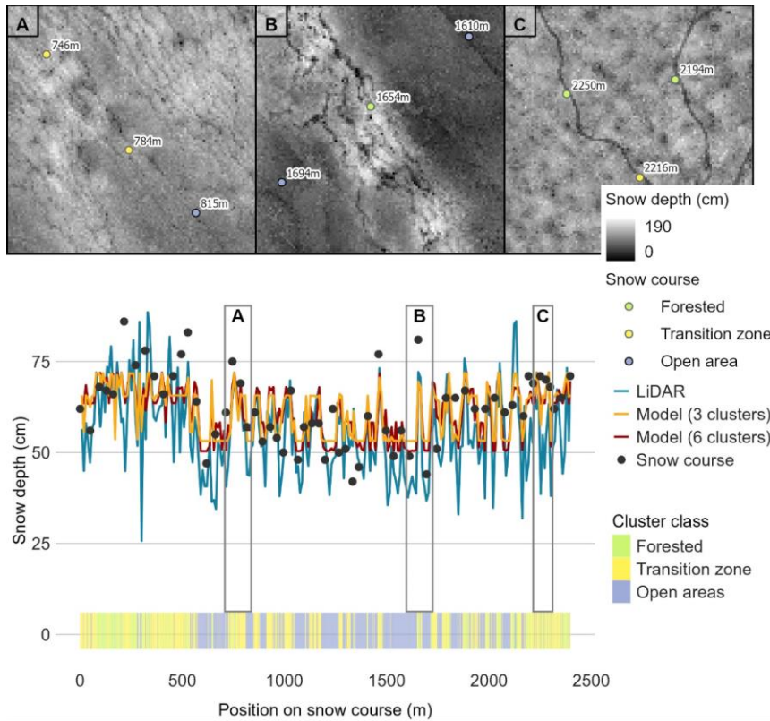
Figure 9. The transect from Sodankylä modelled snow depths, UAV-based UAV-LiDAR snow depths and snow course measurements and their representative clusters on 26.3.2024. The yellow line shows the model output of the model with the number of clusters set to three, as used in this study. For comparisons, The red line represents the model output with the numbers of 6 clusters set to six, allowing more detailed snow depth estimates.
