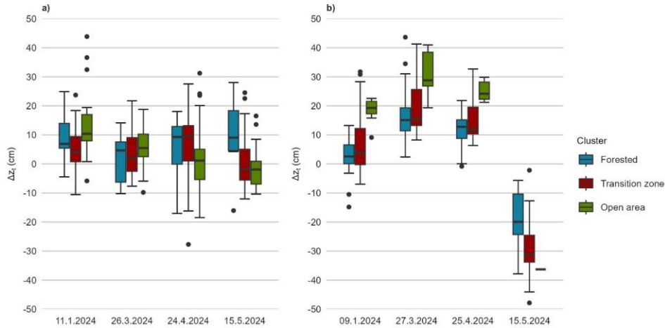
Figure 5. Differences in \Delta z_t (cm) between the UAV-based LiDAR UAV snow depths and snow course measurements by each campaign and representative cluster in (a) Sodankylä and (b) Pallas.
