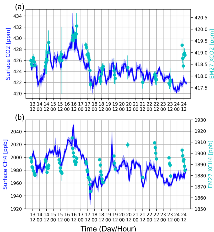
Figure 5. Similar to Figure 4, but adding the EM27/SUN FTIR XCO 2 and XCH 4 hourly means and stds (right y-axis) between 13 and 24 May 2022.
