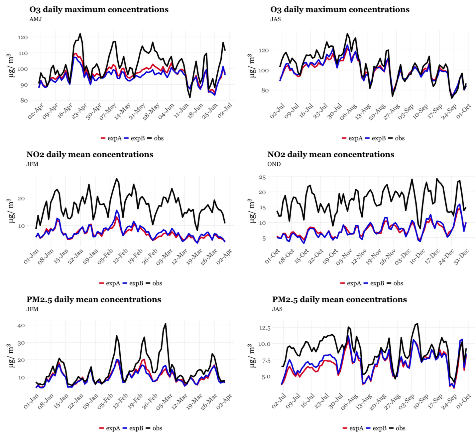
Figure 22 Spatial median of the observed (black) and modelled (red, expA; blue expB) daily maximum concentration of O 3 by the ENS during AMJ and JAS and daily mean concentration of NO 2 during JFM and OND and PM 2.5 during JFM and JAS for 2018.
