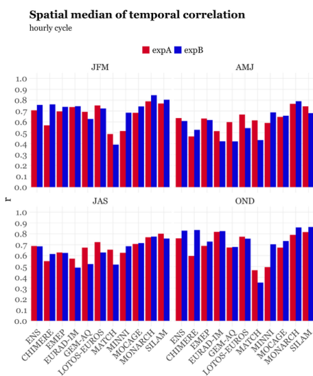
Figure 11 Comparison between the observed and modelled NO 2 diurnal cycle for the ENS (UTC time) for JAS and OND (left) and spatial median of the temporal correlations obtained for the ENS and each individual CAMS model per quarter in expA (red) and expB (blue).
