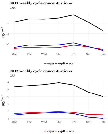
660 Figure 10 Comparison between the observed and modelled NO 2 weekly cycle for the ENS for JFM and JAS (left) and spatial median of the temporal correlations obtained for the ENS and each individual CAMS model per quarter in expA (red) and expB (blue).
