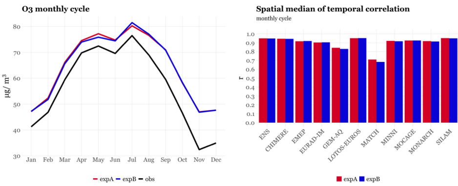
705 Figure 12 Comparison between the observed and modelled O 3 monthly cycle for the ENS (left) and spatial median of the temporal correlations obtained for the ENS and each individual CAMS model in expA (red) and expB (blue).
