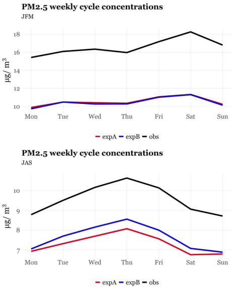
820 Figure 19 Comparison between the observed and modelled PM 2.5 weekly cycle for the ENS for JFM and JAS (left) and spatial median of the temporal correlations obtained for the ENS and each individual CAMS model per quarter in expA (red) and expB (blue). ▽
