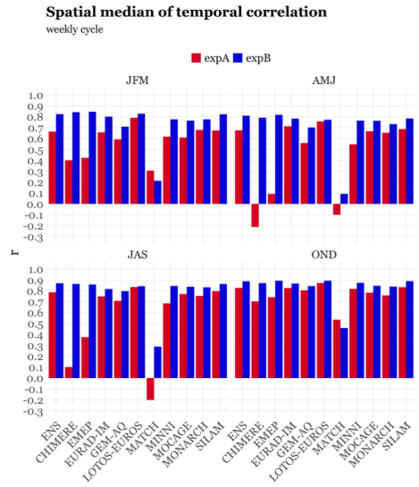
660 Figure 10 Comparison between the observed and modelled NO 2 weekly cycle for the ENS for JFM and JAS (left) and spatial median of the temporal correlations obtained for the ENS and each individual CAMS model per quarter in expA (red) and expB (blue).
