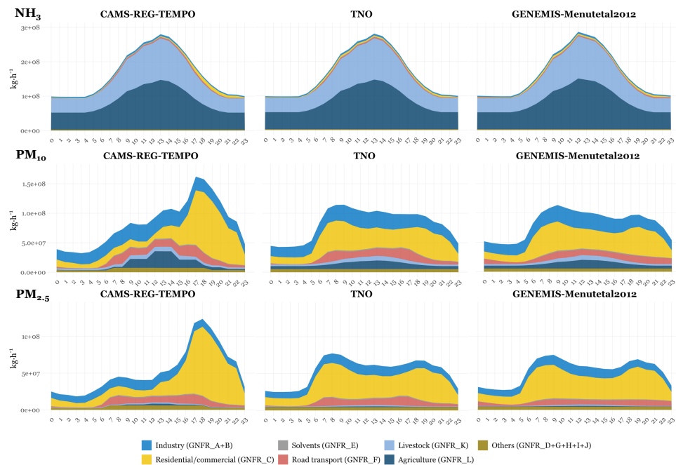
520 Figure 6 Same as Fig. 5 for NH 3 , PM 10 and PM 2.5
