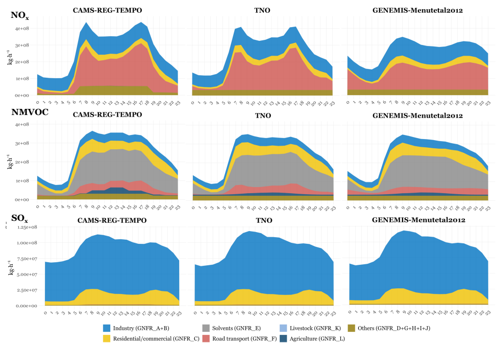
515 Figure 5 Diurnal NO x , NMVOC and SO x emission temporal distributions obtained per pollutant and sector at the EU27 plus UK and Norway level when using the CAMS-REG-TEMPO, TNO and GENEMIS-Menutetal2012 profiles, respectively.
