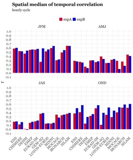
785 Figure 17 Comparison between the observed and modelled PM 10 diurnal cycle (UTC time) for the ENS for JFM and OND (left) and spatial median of the temporal correlations obtained for the ENS and each individual CAMS model per quarter in expA (red) and expB (blue).▼
