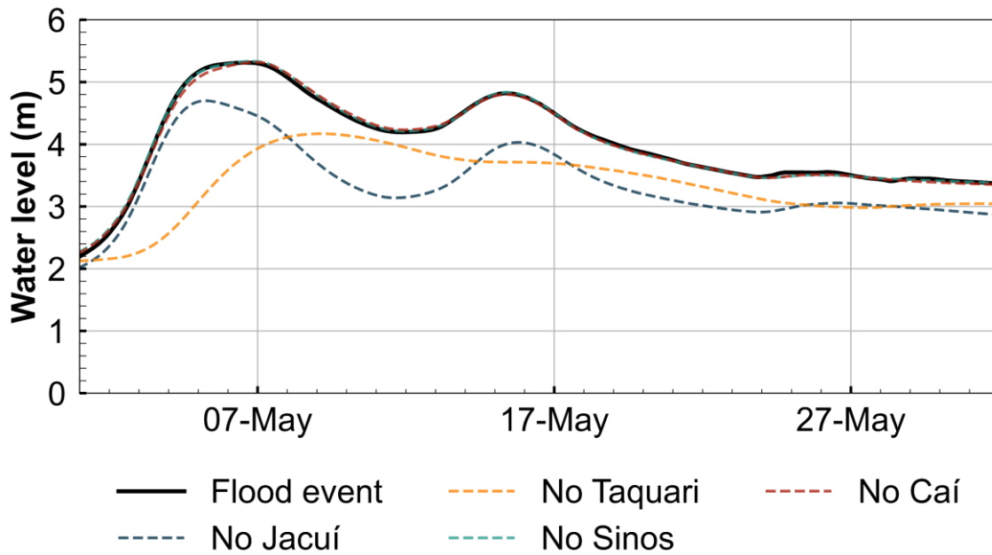
Figure 9. Impact of individual river contributions on RMPA flooding, based on scenarios where each river’s input was removed from the simulation (Taquari, Jacuí, Sinos, Gravataí, and Cai). The Jacuí and Taquari rivers are identified as the primary flood contributions. Excluding the Taquari River’s input would lower the peak flood level to 4.25 meters, while removing the Jacuí River’s contribution would lower the peak to 4.75 meters. In both scenarios, the peak flood level would still exceed the flood threshold for RMPA cities.
