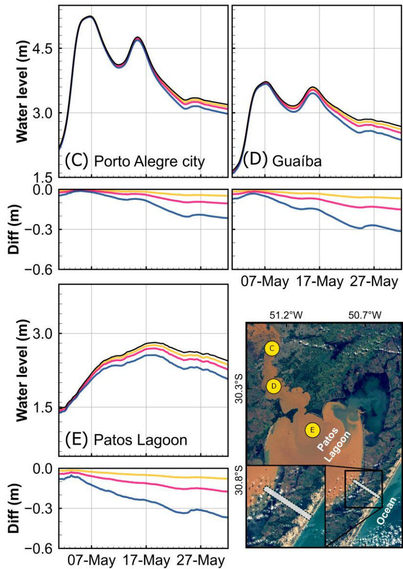
370 Figure 12. Second evaluated flood mitigation scenario for the RMPA considered the construction of a channel connecting the Patos Lagoon and the Atlantic Ocean in its northeastern portion. Points C, D and E illustrate the influence of the channel on reducing flooding in the region.
