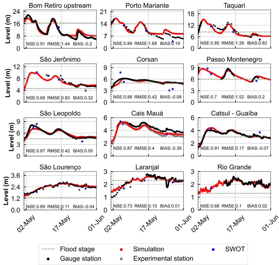
280 Figure 5: Water level simulations (red) compared to observations at twelve-gauge stations observations (black) located in the study area, alongside water surface elevation (WSE) data from the SWOT mission (blue). The grey line in the Cais Mauá plot corresponding to the experimental site data, and the dashed line indicates the flood stage at each station.
