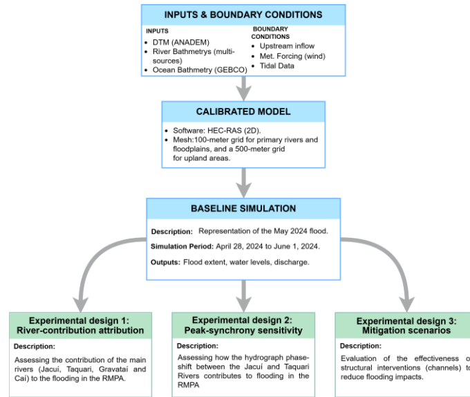
210 Figure 3. The workflow for this study proceeded by defining the input and boundary conditions for the May 2024 flood, followed by calibrating and validating a baseline model, which was then utilized to analyse multiple scenarios.
