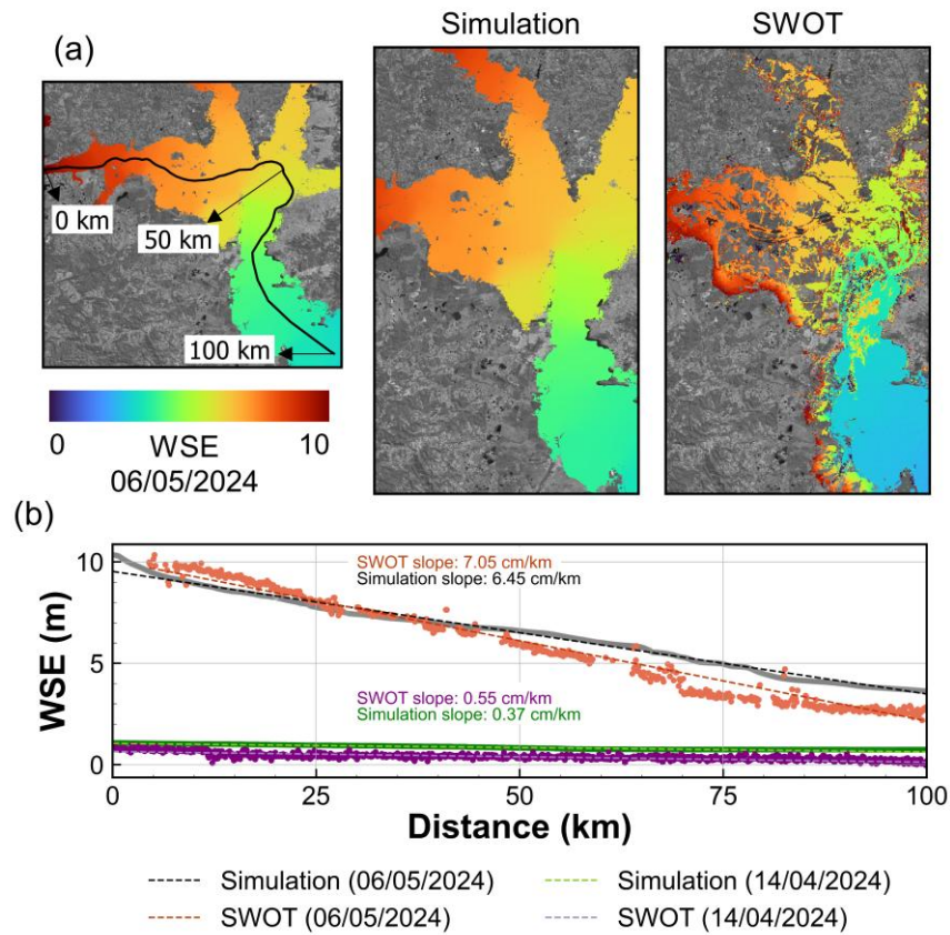
285 Figure 6: Water surface elevation slope from the 2D simulation (a) compared with SWOT data observation from May 6th. The profile line between Jacuí and Guaíba River (b) showed steep water slope changes (SWOT = 7.05 cm/km and Simulation = 6.45 cm/km) compared to low waters stable conditions (SWOT = 0.55 cm/km and Simulation = 0.37 cm/km).
