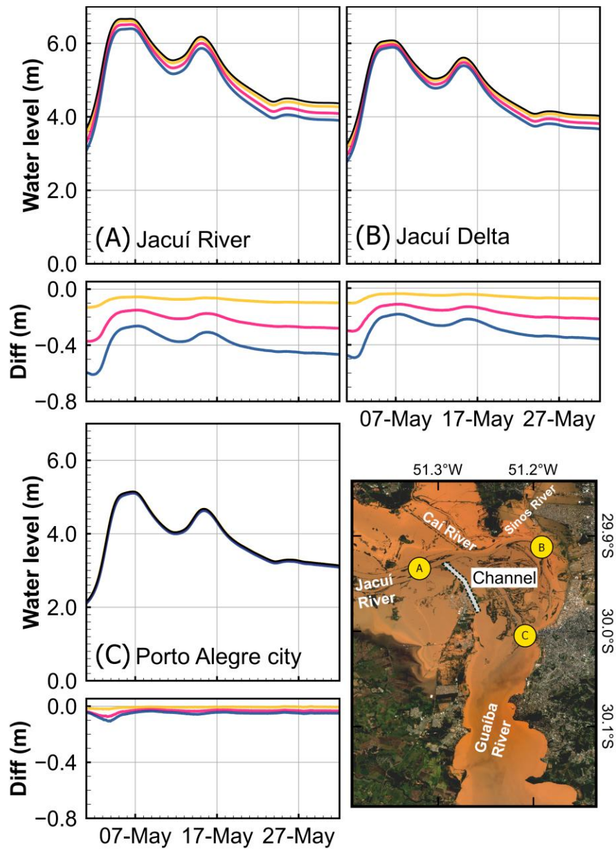
360 Figure 11. Evaluated scenario for mitigating flooding in the RMPA involved a channel connecting the Jacuí and Guaíba rivers. Points A, B, and C illustrate the channel's effectiveness in reducing water levels around the Jacuí Delta.
