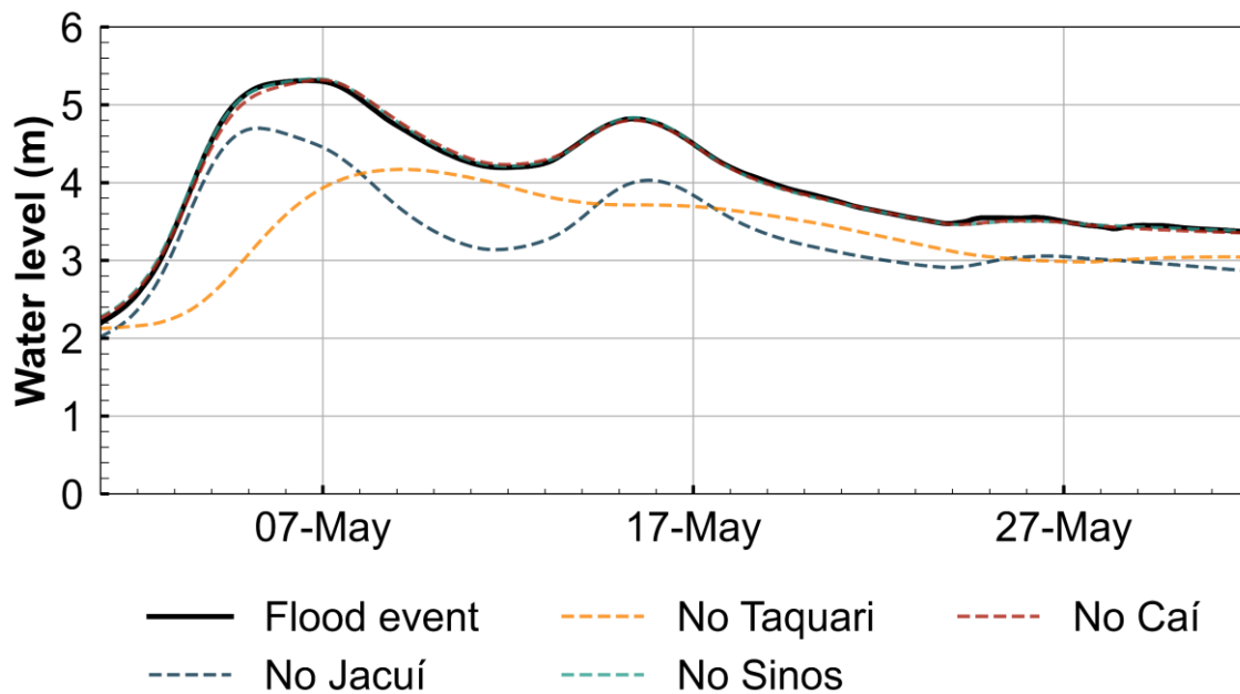
330 Figure 9: Impact of individual river contributions on RMPA flooding, based on scenarios where each river’s input was removed from the simulation (Taquari, Jacuí, Sinos, Gravataí, and Cai). The Jacuí and Taquari rivers are identified as the primary flood contributions. Excluding the Taquari River’s input would lower the peak flood level to 4.25 meters, while removing the Jacuí River’s contribution would lower the peak to 4.75 meters. In both scenarios, the peak flood level would still exceed the flood threshold for RMPA cities.
