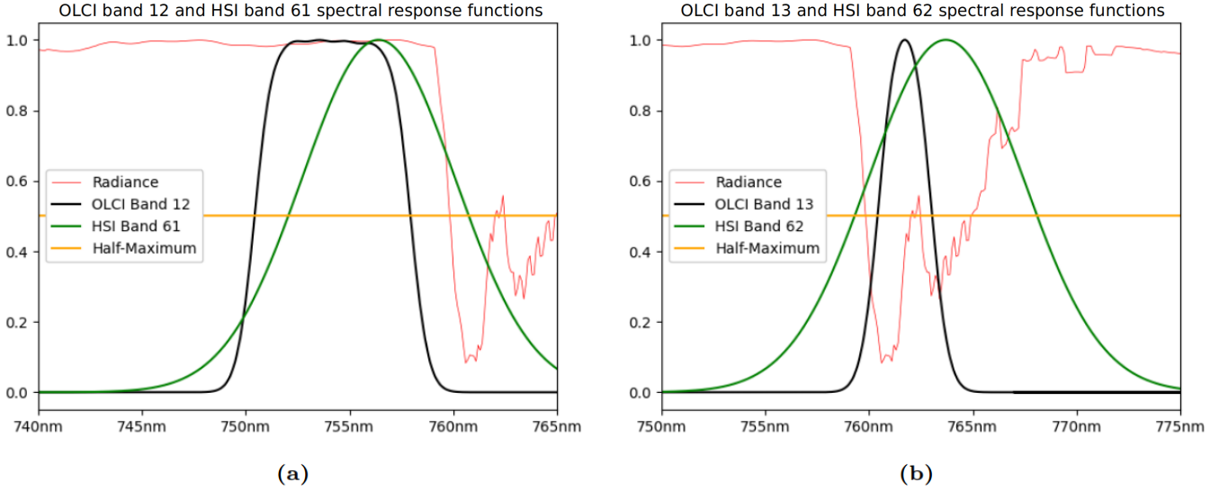
Figure 3. O 2 A-Band. The spectral response functions of (a) O_{12} and H_{61} and (b) O_{13} and H_{62} , overlain on a 1 nm rolling-average of radiances simulated using SCIATRAN (Rozanov et al., 2014) at 0.1 nm spectral resolution (red line). All curves are plotted relative to their maximum within the range. The orange line is intended as a visual aid to help identify the FWHM of the two spectral response functions.
