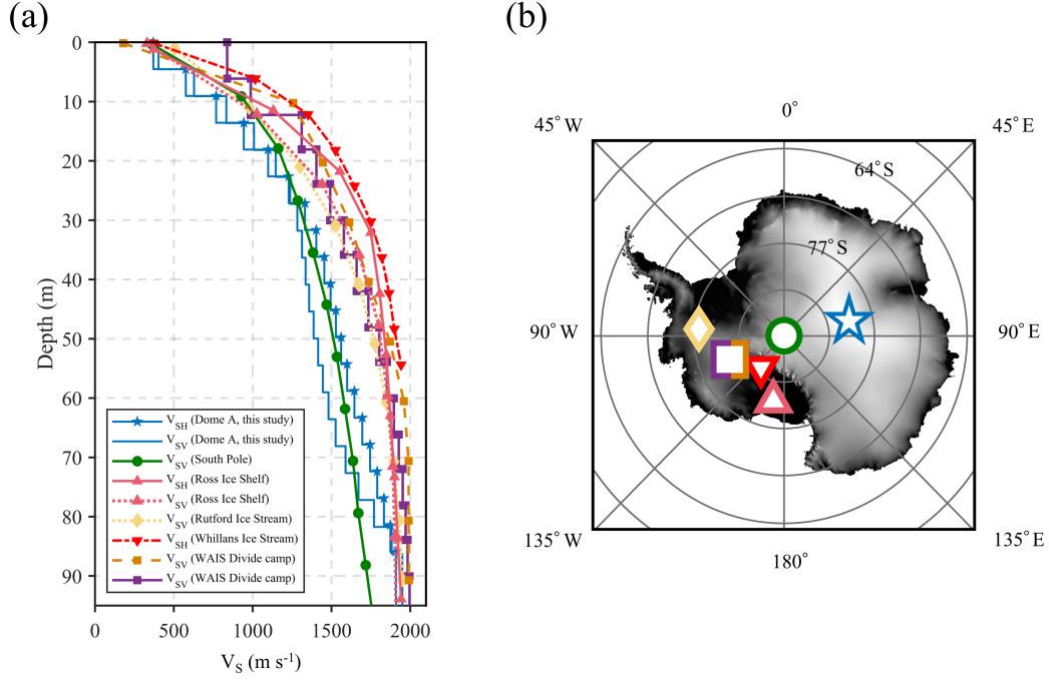
Figure 5. S-wave velocity from different areas in Antarctica. (a) V_{SH} , V_{SV} from this study (blue line with pentagrams and blue line), V_{SV} from South Pole (Yang et al., 2024; green curve with circles), V_{SH} and V_{SV} from Ross Ice Shelf (Diez et al., 2016; pink curve with triangles and pink dotted curve with triangles), V_{SV} from Rutford Ice Stream (Zhou et al., 2022; yellow dotted curve with diamonds), V_{SH} from Whillans Ice Stream (Picotti et al., 2024; red dash-dot curve with inverted triangles), V_{SH} and V_{SV} from WAIS Divide camp (Qin et al., 2024, Zhang et al., 2024; brown dashed curve with squares and purple line with squares). The markers in (b) corresponding to (a) represent the respective study areas from different research areas in Antarctica.
