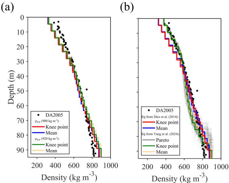
Figure A1. Density estimated by empirical relationship. (a) Using a relationship from Diez et al. (2014) with V_{SH} . The red and blue lines use an ice density of 900\text{ kg m}^{-3} , while the green and yellow lines use 920\text{ kg m}^{-3} . (b) Using the relationship from Yang, Zhan et al. (2024) with V_{SV} (grey, green and yellow lines). The filled circles show the ice core (DA2005) density near Dome A. The red and blue lines in (a) and (b) are consistent with Fig. 3c in the main text.
