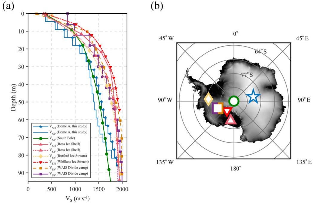
245 Figure 5. S-wave velocity from East and West different areas in Antarctica. (a) East Antarctica: V_{SH} , V_{SV} from this study (blue line with pentagons and blue line), and V_{SV} from South Pole (Yang et al., (2024); (green curve with circles), West Antarctica: V_{SH} and V_{SV} from Ross Ice Shelf (Diez et al., (2016); (pink curve with triangles and pink dotted curve with triangles), V_{SV} from Rutford Ice Stream (Zhou et al., (2022); (yellow dotted curve with diamonds), V_{SH} from Whillans Ice Stream (Picotti et al., (2024); (red dash-dot curve with inverted triangles), V_{SV} and V_{SV} from WAIS Divide camp (Qin et al., (2024), Zhang et al., 2024; (brown dashed curve with squares), and V_{SV} from Zhang et al. 2024 (purple line with squares). The markers in (b) corresponding to (a) represent the respective study areas from different 250 research-works areas in Antarctica.
