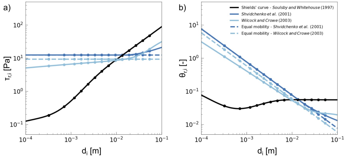
205 Figure 1: Comparison of the S2001 and WC2003 formalisms. a) Reference shear stress as a function of grain size. b) Reference Shields stress as a function of grain size. The Shields's curve is included as well as the curves corresponding to equal mobility conditions. Dots correspond to grain size classes of WC2003's dataset for the grain size distribution with the lowest sand fraction.
