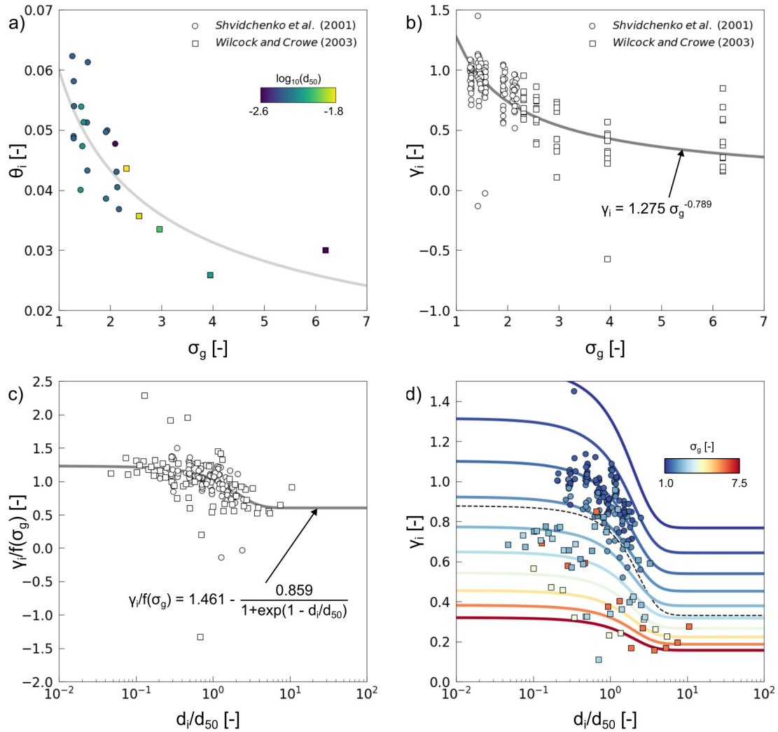
430 Figure 3: New formalism of reference shear stress for incipient motion of multiple-size sediments. a) Variations of reference Shields stress of the median size as a function of the final surface grain size sorting. The grey line corresponds to Eq. (22) ( R^2=0.69 ). Markers are colored according to the median grain size. b) Variations of exponent in hiding function as function of grain size sorting. c) Variations of exponent in hiding function without the effect of the grain size sorting as function of grain size to median grain size ratio. d) Variations of exponent in hiding function as a function of grain size to median size ratio. Markers are 435 colored according to the final surface grain size sorting. Equation (24) ( R^2=0.74 ) is plotted for ten values of final surface grain size sorting. The dashed line corresponds to the equation of Wilcock and Crowe (2003).
