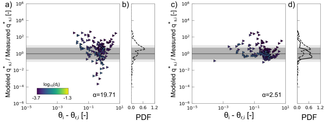
Figure 8: Effects of standardized incipient motion and adjusted transport height on predictions of total load transport rates at equilibrium for Engelund and Hansen (1967). a-b) Predictions with the same critical shear stress values as of Le Minor et al. (2022) and the original parameterization of LM2022's model ( \alpha=19.71 ). c-d) Predictions with the LM2022's model adjusted with the bed roughness length as reference height across all grain sizes, a bed roughness of 3d_{90}/30 (no bed forms) and the standardized reference shear stress values after re-calibration ( \alpha=2.51 ). The ratio of model predictions to flume observations is plotted against the dimensionless excess of shear stress (Shields stress) along with the probability density function (PDF) of the residuals. For the PDF, the dashed line corresponds to predictions with the original LM2022's model. The solid line in d) corresponds to predictions with the adjusted model. The dark and light gray areas correspond to measured values that are predicted within a factor of 5 and 10, respectively. 675
