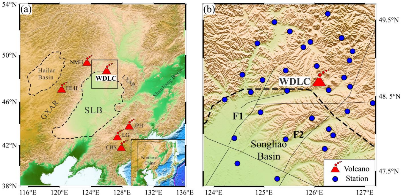
Figure 1: Map view of the surface topography and major tectonic settings of the Wudalianchi (WDLC) volcanic field. The blue circles denote seismic stations used in this study. The dashed line and thin black lines mark the outlines of the basins and major faults, respectively. CBS, Changbaishan; HLH, Halaha; LG, Longgang; JPH, Jingpohu; NMH, Nuominhe; SLB, Songliao Basin; GXAR, Great Xing'an range; LXAR, Lesser Xing'an range; F1, Nenjiang fault; F2, Hailun-Renmin fault.
