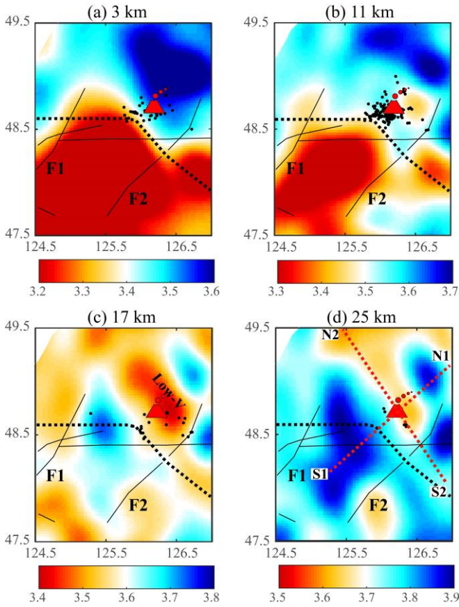
Figure 6: Shear-wave velocity structures at multiple depths. The red dashed lines in (d) mark the profile locations in Figure 7. The black dashed lines mark the outlines of the Songliao Basin. The black dots represent the earthquakes beneath the WDLV volcano. Other labels are the same as those in Figure 1.
