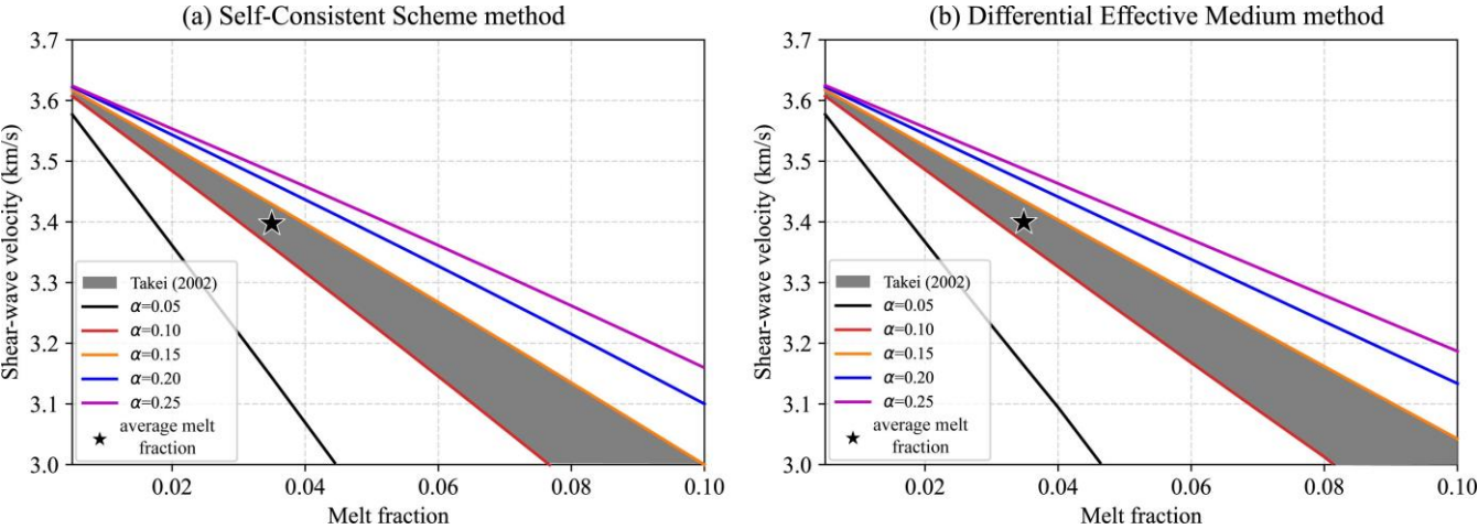
Figure 9: Estimation of the melt fraction for the middle-lower crustal magma reservoir beneath the WDLC volcano. The black star is the average melt fraction for the middle-lower crustal magma reservoir using the aspect ratio suggested by Takei (2002).
