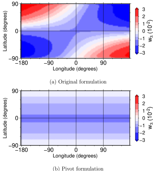
Figure 1. Demonstration of the remapping weight computation. (a) w_{3nk} using the J99 original algorithm (Eq. 14) (b) w_{3nk} by Eq. (21).
