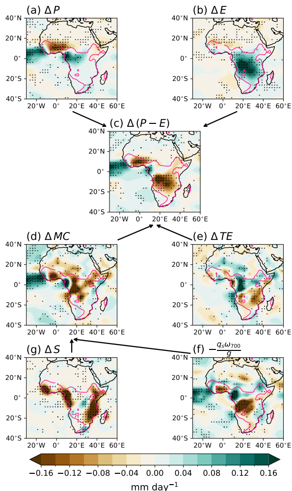
Figure 3. Spatial maps of MJJAS changes in (a) precipitation \Delta P , (b) evapotranspiration \Delta E , (c) net precipitation \Delta(P - E) , (d) mean-circulation mean-circulation moisture flux term \Delta MC , (e) transient eddy term \Delta TE , (f) omega scaling and (g) surface term \Delta S over Africa in AFFOREST. Pink contours enclose the regions where there are is at least 5% of afforestation. Stippling shows where 6 out of 7 ESMs agree on the sign of change. Arrows show the relationship between the different variables.
