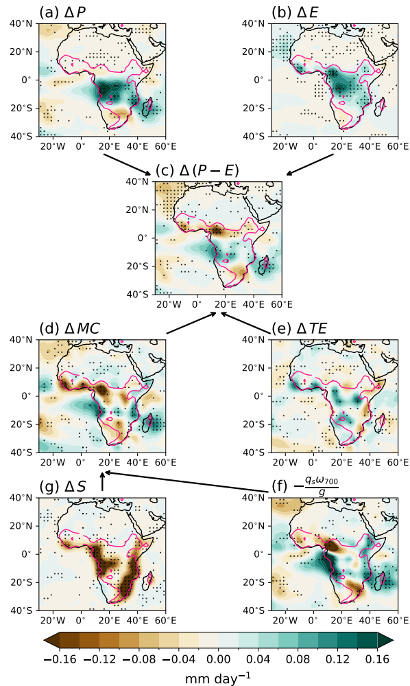
Figure 4. Spatial maps of Same as Figure 3 but for ND-JFM changes in (a) precipitation \Delta P , (b) evapotranspiration \Delta E , (c) net precipitation \Delta(P - E) , (d) mean-circulation mean-circulation moisture flux term \Delta MC , (e) transient eddy term \Delta TE , (f) omega scaling and (g) surface term \Delta S over Africa in AFFOREST. Pink contours enclose the regions where there are is at least 5% of afforestation. Stippling shows where 6 out of 7 ESMs agree on the sign of change. Arrows show the relationship between the different variables.
