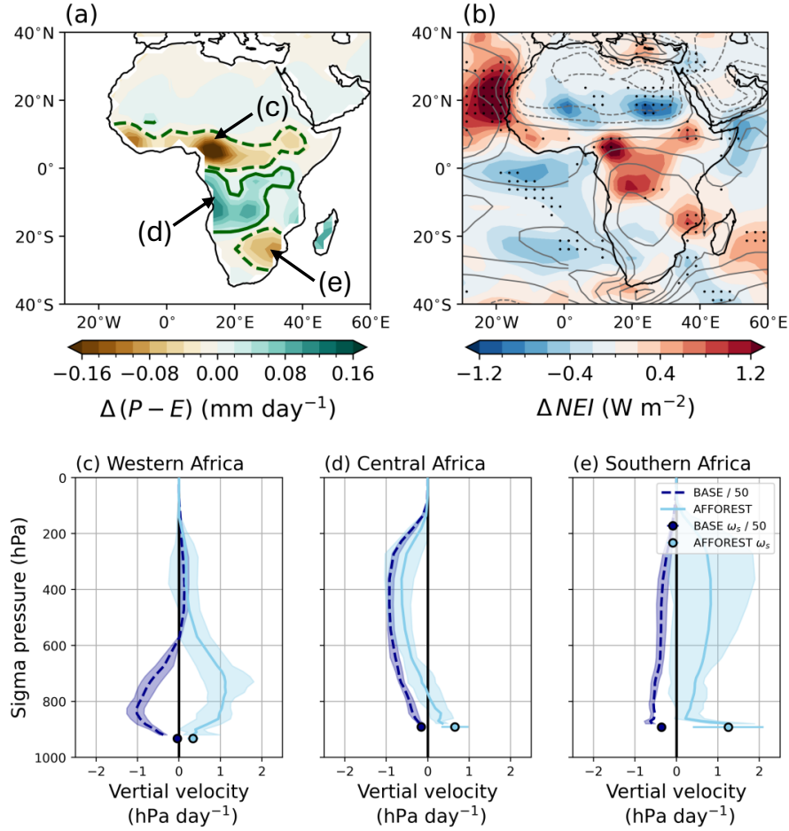
Figure 7. Spatial maps of Same as Figure 6 but for NDJFM changes in (a) net precipitation \Delta(P - E) and (b) net energy input \Delta NEI over Africa in AFFOREST. In (b), contours show BASE values of NEI with a spacing of 20 \text{ W m}^{-2} . (c-e) Vertical profile of BASE values (dark blue) and changes following AFFOREST (light blue) in vertical-velocity \omega averaged over the western, central and southern African regions indicated in (a). The dark blue dot shows the BASE value and light blue one the AFFOREST value of vertical-velocity at the surface \omega_s with error bars showing the 25-75 th percentile. Note that BASE values have been divided by 50 to display them on the same axes and the profiles are interpolated to sigma coordinates. The sigma coordinates are calculated as pressure divided by the grid-cell surface pressure in BASE and multiplied by the area-averaged surface pressure in BASE to get sigma coordinates in pressure units. The surface values (dots) are positioned at the average surface pressure in BASE over the relevant region. Also note that the regions marked as western western, central and southern Africa are not the same as in Fig. 6.
