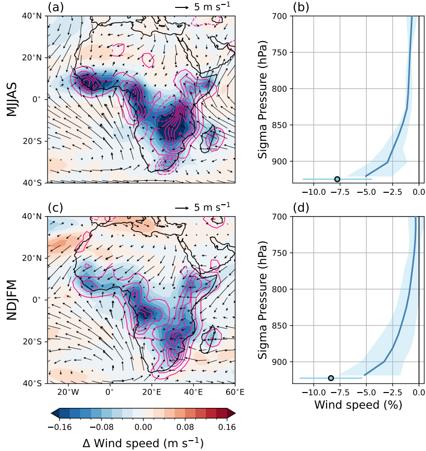
Figure 5. (a, c) Spatial maps of changes in surface-near-surface wind speed (filled contours) over Africa for AFFOREST in MJJAS (upper row) and NDJFM (lower row). Pink contours show changes in surface-near-surface pressure vertical velocity \omega_s with solid (dashed) contours indicating positive (negative) values. Vectors show BASE surface winds. (b, d) Vertical profile of percentage changes in wind speed over Africa (land region of 37°S-15°N, 20°W-50°E) interpolated to sigma coordinates. The sigma coordinates are calculated as pressure divided by the grid-cell surface pressure in BASE and multiplied by the area-averaged surface pressure in BASE to get sigma coordinates in pressure units. The envelope shows the 25 th to 75 th percentile model spread. The light blue dot shows the percentage changes in surface wind speed (positioned at the average surface pressure in BASE) with the error bar showing the 25 th -75 th percentile model spread.
