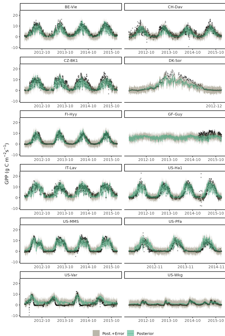
Figure D5. Time series plot of observed (black crosses) and modelled daily gross primary production (GPP) for setup h-S6 for years 2012 to 2015 of the training data set. Model output is computed with parametric uncertainty (green shaded area, based on 20 samples from the posterior) and structural uncertainty (grey shaded area, based on 3 samples from error model).
