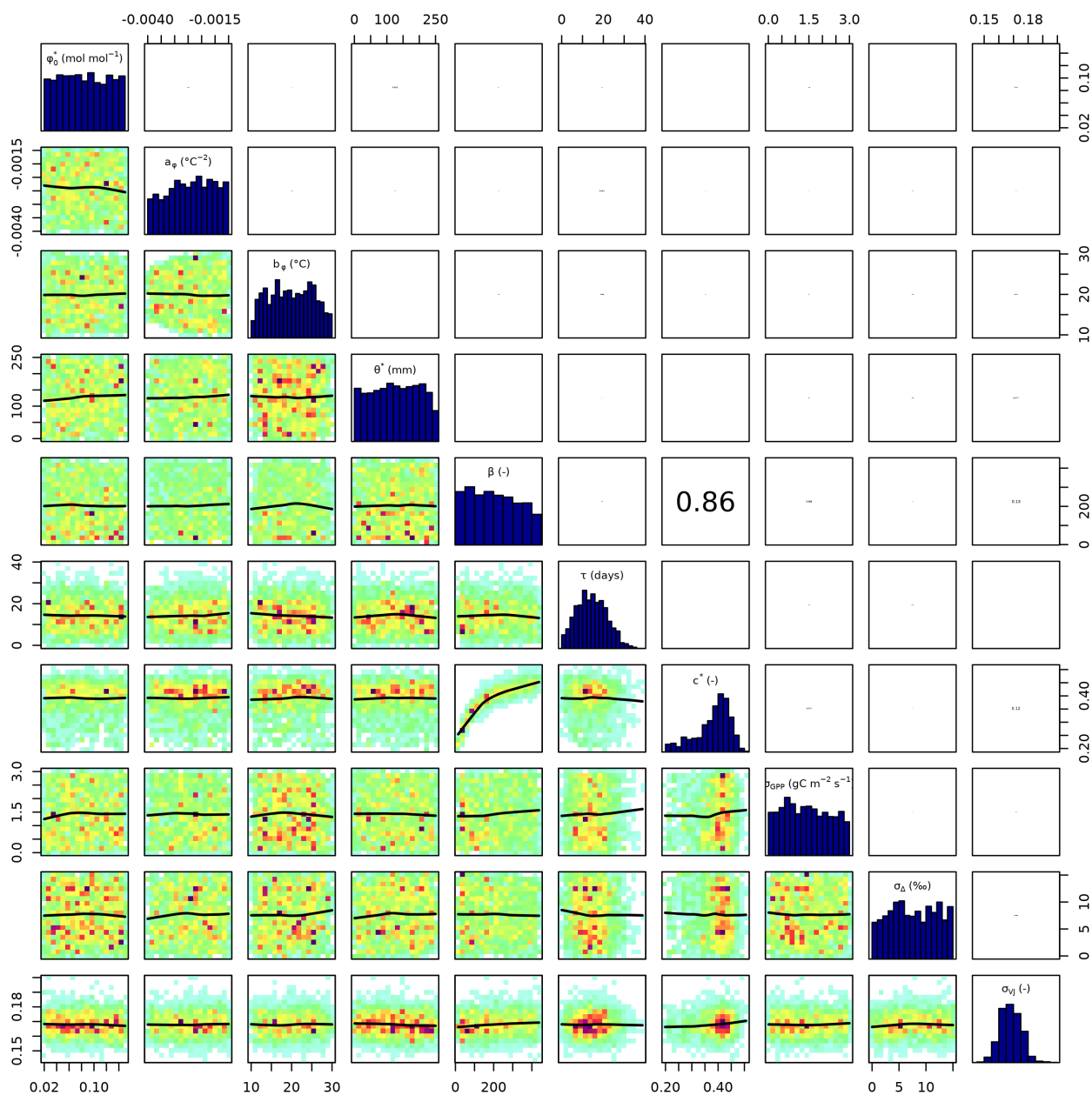
Figure D2. Parameter correlation of posterior parameters in setup b - S2 with 100'000 iterations and 30'000 burnin - in .
