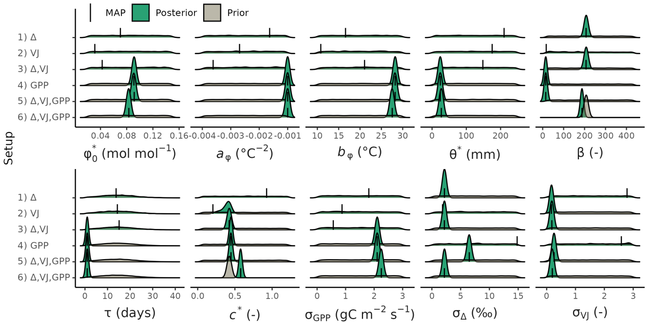
Figure 3. Prior and posterior distributions of the calibrated model parameters and error model terms in the for different setups. The maximum a posteriori (MAP) estimates are indicated with a dashed line and fixed parameters with solid lines line. For parameter description and units refer to See Table 2 for parameter descriptions .
