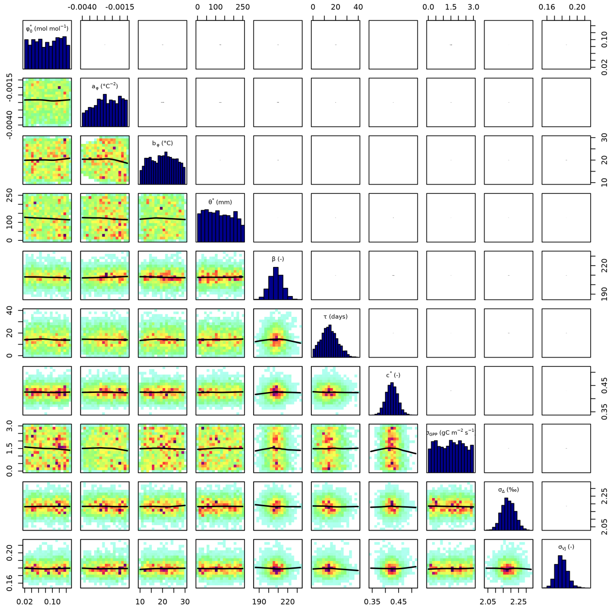
Figure D3. Parameter correlation of posterior parameters in setup \text{e} \rightarrow \text{S3} with 100'000 iterations and 30'000 burn-in.
