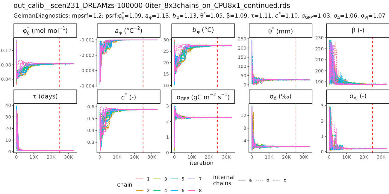
Figure D1. Trace plot of MCMC sampling of all parameters in setup h)S6 .
