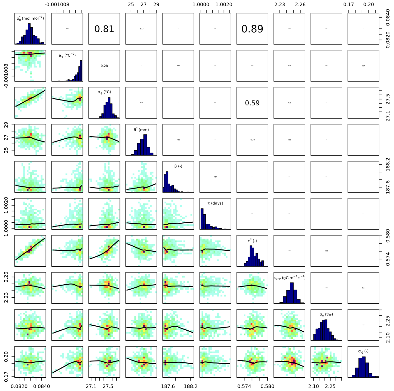
Figure D4. Parameter correlation of posterior parameters in setup \text{h}\text{S6} with 100'000 iterations and 30'000 burn-in.
