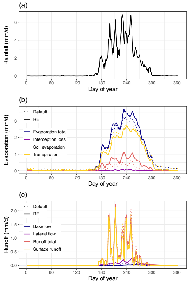
Figure 2. Average yearly cycle of simulated hydrology at the Dahra site in Senegal for 2002-2022, comparing the default LPJ- GUESS v4.1 multilayer soil hydrology (Default; dotted line) with the updated soil hydrology based on Richards equations 430 with the “free drainage” bottom boundary condition (RE; solid line). Figures show 5-day moving averages of (a) in-situ measured daily rainfall for reference, (b) simulated daily evaporation components, and (c) simulated daily runoff components.
