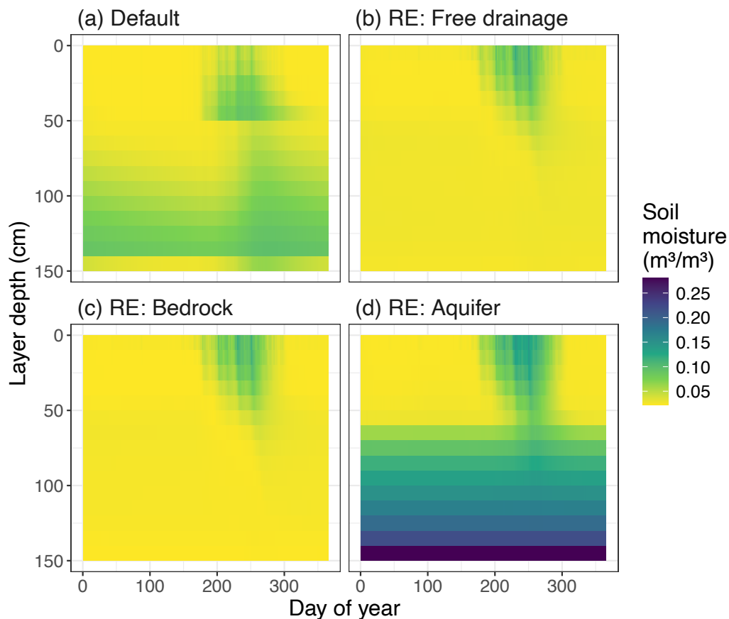
435 Figure 3. Average yearly cycle of soil moisture ( \text{m}^3/\text{m}^3 ) for the Dahra fluxtower site, as simulated by the different soil hydrology modules in (a) the default version of LPJ-GUESS v4.1 and (b-d) the updated version based on Richards equation with the available bottom boundary conditions. Boundary conditions include (b) free drainage (the default used for model evaluations), (c) impermeable bedrock, and (d) a permanent aquifer below the bottom layer.
