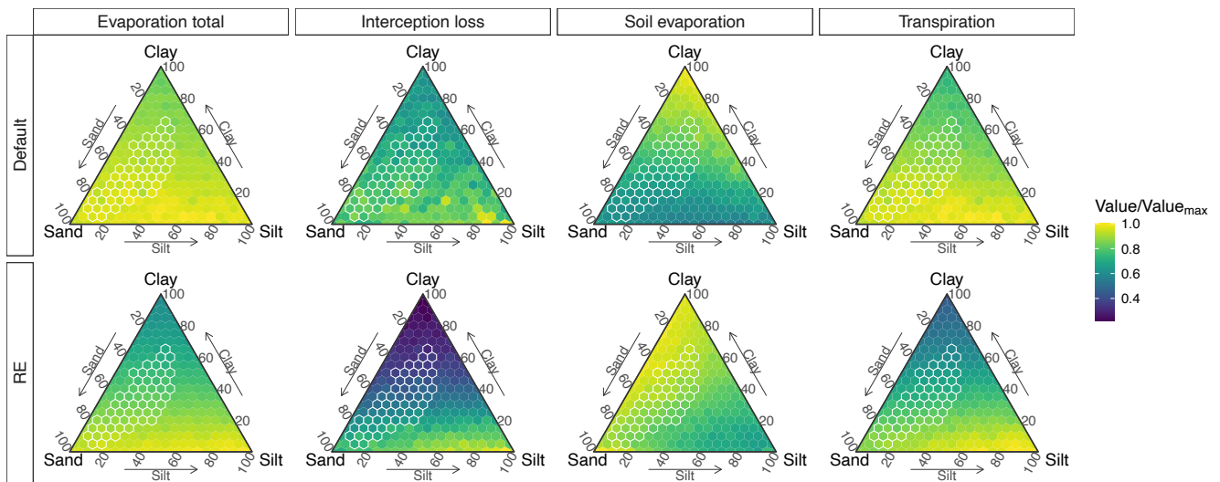
Figure 11. Simulated sensitivity of evaporation components (columns) to soil texture for both model versions (rows), based on the Dahra meteorological drivers. Sensitivities represented by ternary plots of time-series average evaporation component values for each soil type. Values are divided by maximum evaporation value over all soil types ( Value_{max} ), calculated for each model version and each evaporation component separately. Soil textures found in the Sudan-Sahel region are marked in white.
