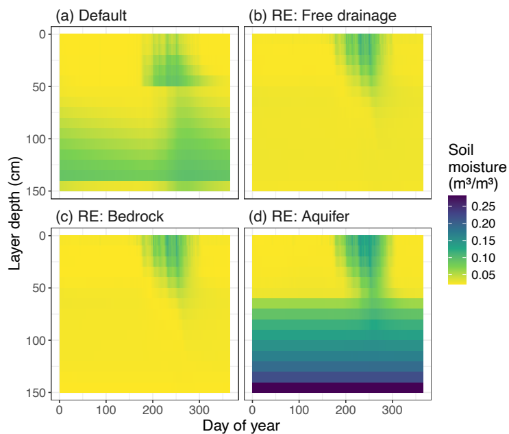
505 Figure 3. Average yearly cycle of soil moisture ( \text{m}^3/\text{m}^3 ) for the Dahra fluxtower site, as simulated by the different soil hydrology modules in (a) the default version of LPJ-GUESS v4.1 and (b-d) the updated version based on Richards equation with the available bottom boundary conditions. Boundary conditions include (b) free drainage (the default used for model evaluations), (c) impermeable bedrock, and (d) a permanent aquifer below the bottom layer.
