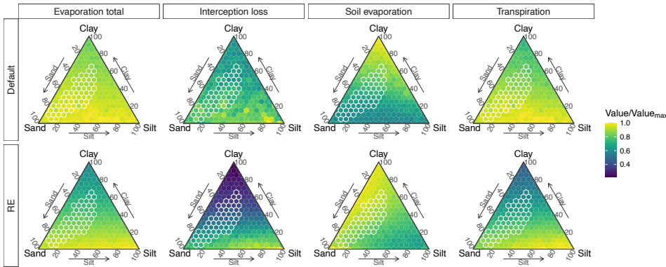
Figure 11. Simulated sensitivity of evaporation components (columns) to soil texture for both model versions (rows), based on the Dahra meteorological drivers. Sensivities represented by ternary plots of time-series average evaporation component values for each soil type. Values are divided by maximum evaporation value over all soil types ( Value_{max} ), calculated for each model version and each evaporation component separately. Soil textures found in the Sudan-Sahel region are marked in white.
