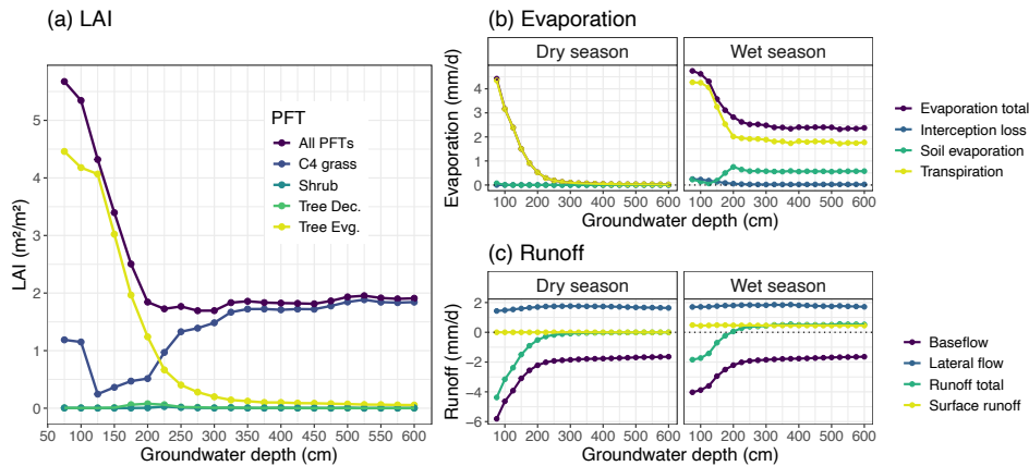
Figure 13. Influence of groundwater depth on simulated vegetation cover and surface hydrology at the Dahra flux tower site.
