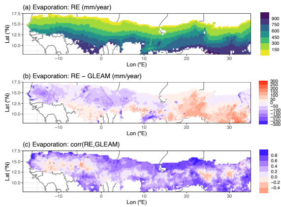
600 Figure 6. Regional simulation of yearly total evaporation by the updated LPJ-GUESS v4.1 model for the period 1980–2022. (a) Multiyear model averages over this time period, (b) difference between multiyear averaged model and GLEAM data, (c) Pearson correlation between model and GLEAM for yearly totals over 1980–2022. For panel (b) all outlier values saturate at \pm 300 mm/year to avoid distorting the colour scale.
