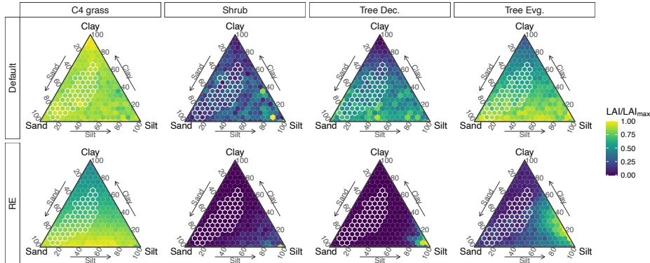
Figure 12. Simulated sensitivity of the different dryland PFTs (columns) to soil texture for both model versions (rows), based on the Dahra meteorological drivers. Sensivities represented by ternary plots of time-series average LAI for each soil type. Values are divided by the maximum LAI value over all soil types ( LAI_{max} ), calculated for each model version and each PFT separately. Soil textures found in the Sudan-Sahel region are marked in white.
