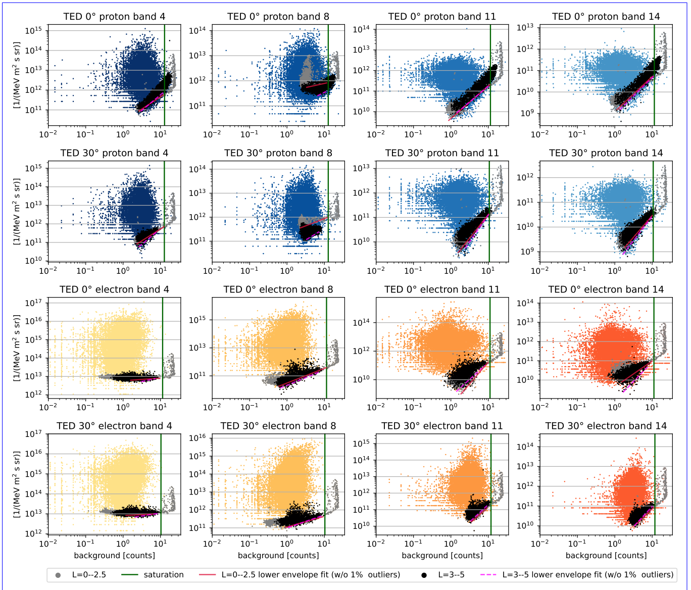
Figure 8. Correlation of TED channels and of NOAA15 plotted against their individual background channel.
