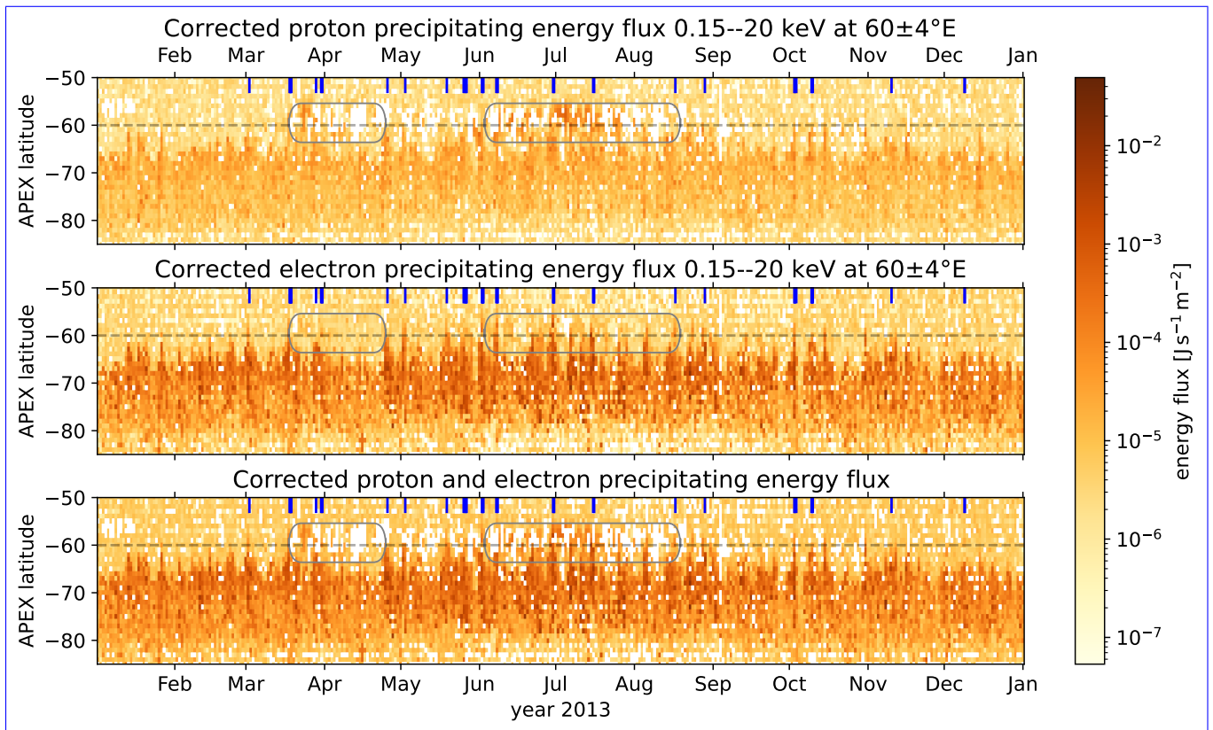
Figure 11. Similar plot as Fig. ?? 6 but with corrected fluxes, two Kp levels and for 60°E APEX only. Note: Dots are uncorrected fluxes that the third panel (protons + electrons) contains data only in case that it is available for both particle species.
