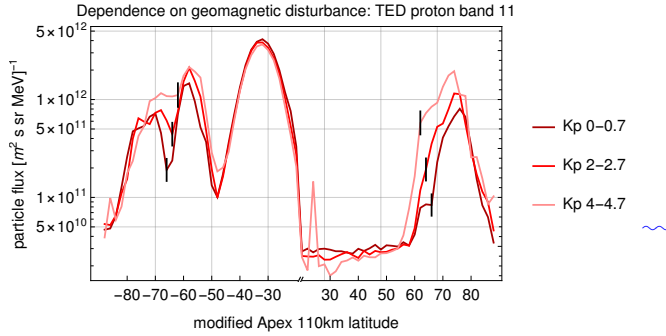
Figure 2. Cross-section at 60°E APEX for TED 0° proton band 11 during varying levels of geomagnetic disturbance. The vertical lines indicate the minimum between the auroral and subauroral peaks. Note that the latitude axis is stitched together, as modified APEX latitudes at 110 km altitude are constrained to values greater than 18°.
