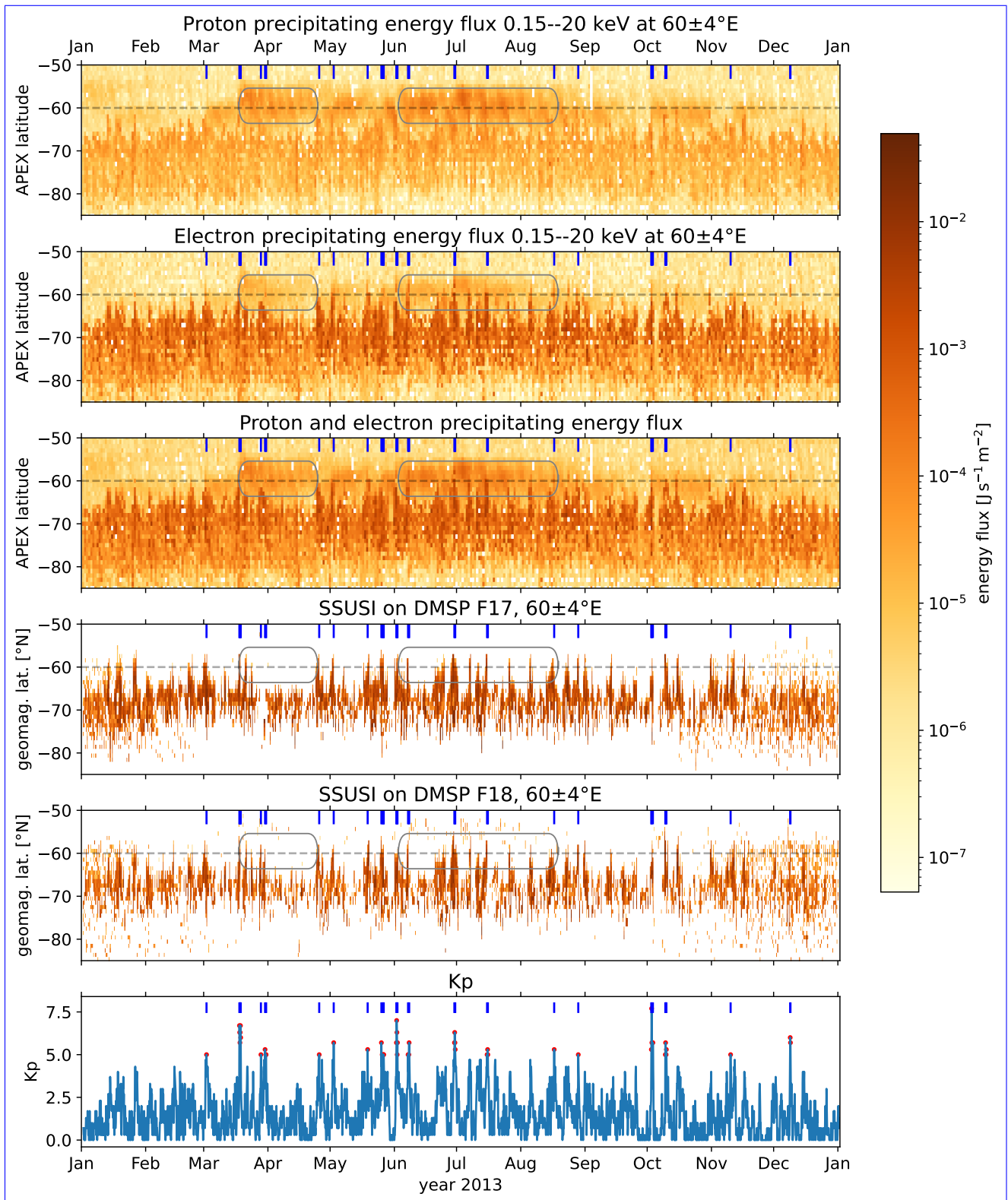
Figure 6. Temporal evolution of electron energy flux, proton energy flux, and their combined flux, compared to the energy flux derived from SSUSI auroral UV radiation from SSUSI as observed by two satellites, and the geomagnetic activity represented by Kp for the year 2013.
