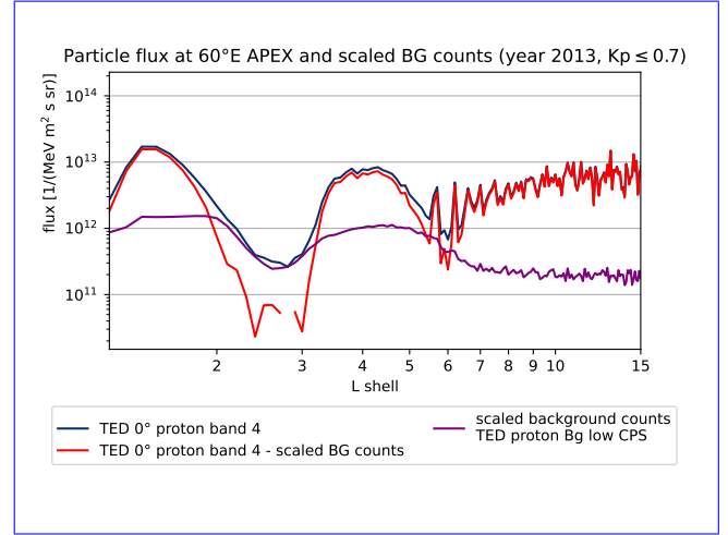
Figure 3. The subauroral peak of the TED channels cannot be adequately corrected based on scaled background counts. Either it creates strong negative fluxes around the peak or the correction does not noteworthy change the fluxes.
