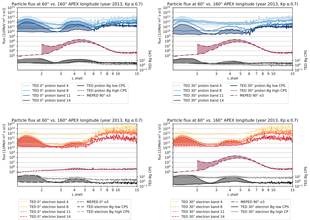
Figure 4. Particle fluxes and background sensor counts for the TED 0° TED and MEPED detectors (left panels) and the TED 30° /MEPED 90° detectors (right panels) in addition to the MEPED 0° or 90° e3 channel. The difference between 60°E and 160°E APEX is highlighted by the shaded area. Below L=6, the higher counts (or fluxes) consistently correspond to 60°E APEX longitude, while the lower values correspond to 160°E APEX. Elevated background counts in the L≤2 (SAA) region and in the L=3–6=3–6 range (subauroral peak) coincide with intense particle counts in TED proton channels and certain the MEPED channels 90° e3 channel.
