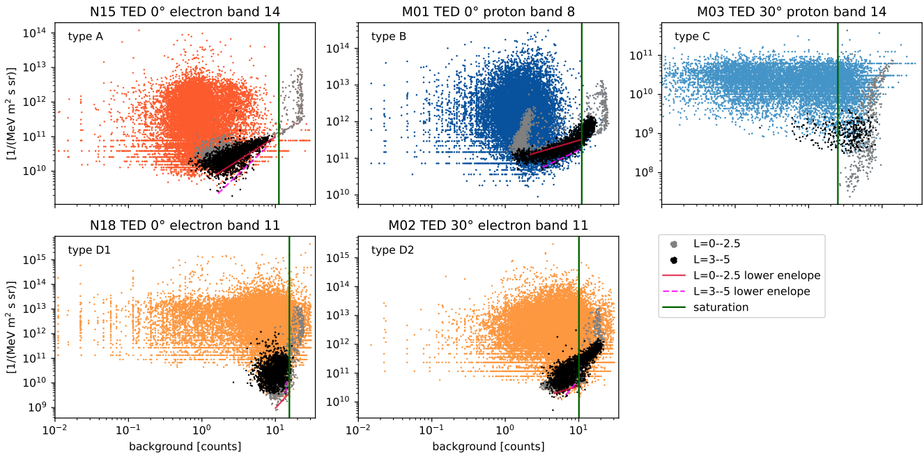
Figure 9. Different types of problematic contamination (see text for details).
