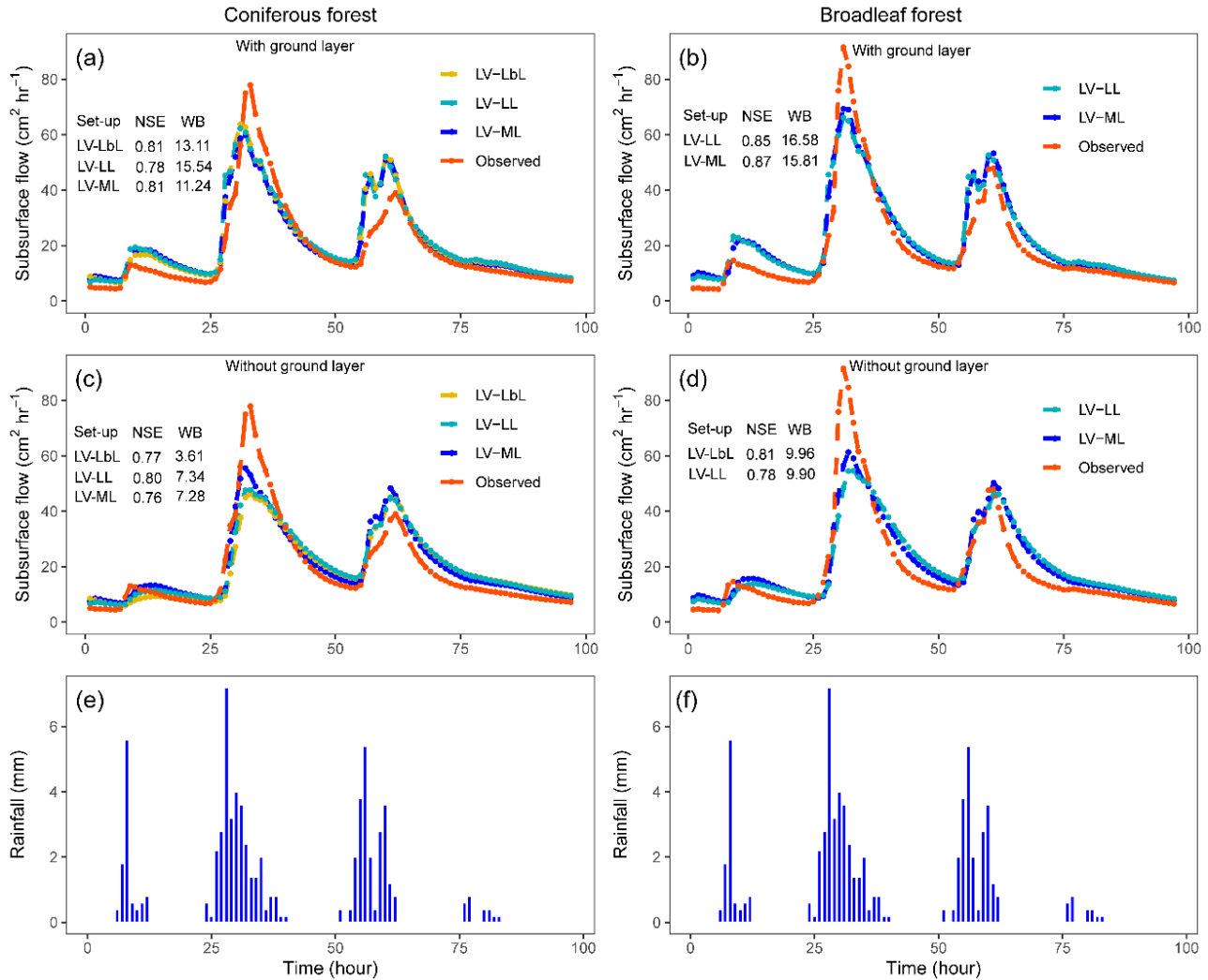
Figure 3: Observed and simulated hydrographs of the acceptable set-ups and their counterparts with a ground layer in the coniferous forest (a, c) and broadleaf forest (b, d) at event scale (e, f).
