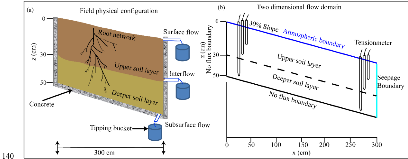
Figure 1: Artificial field configurations (a) and flow domain with boundary conditions in the numerical model (b).
