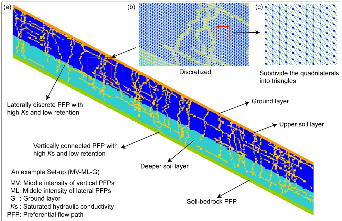
Figure 2: A set-up of hillslope structure with explicit structures (a) and discretization of the flow domain (b, c) in the numerical model.
