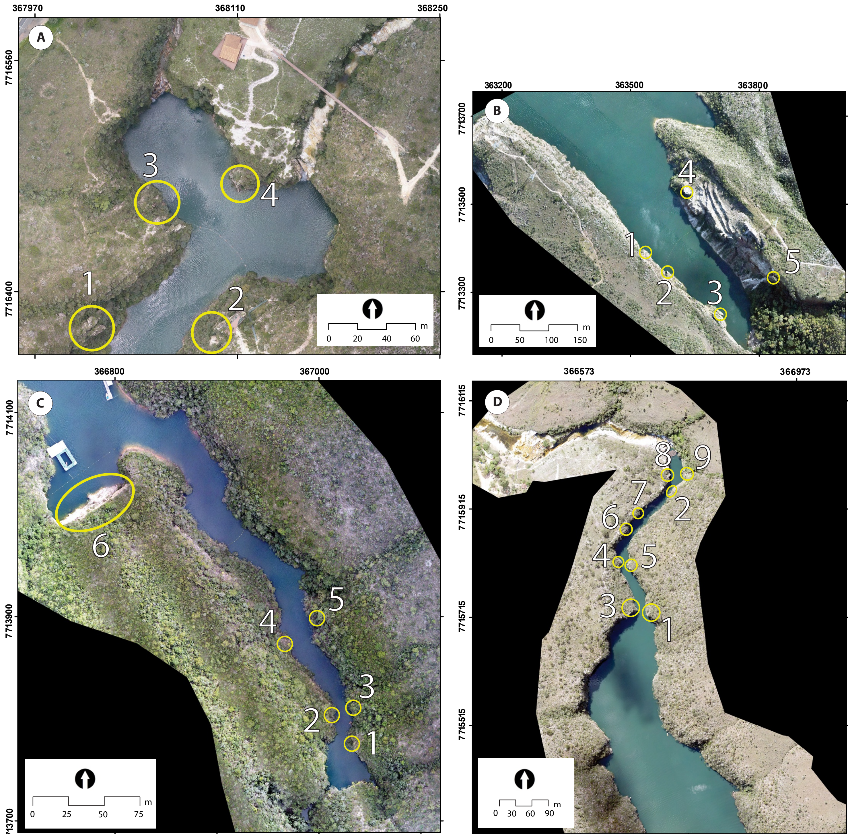
Figure S1: The yellow circles represent the sites where retention structures or removal/destruction of rock blocks should be considered. Numbers represent priority.
