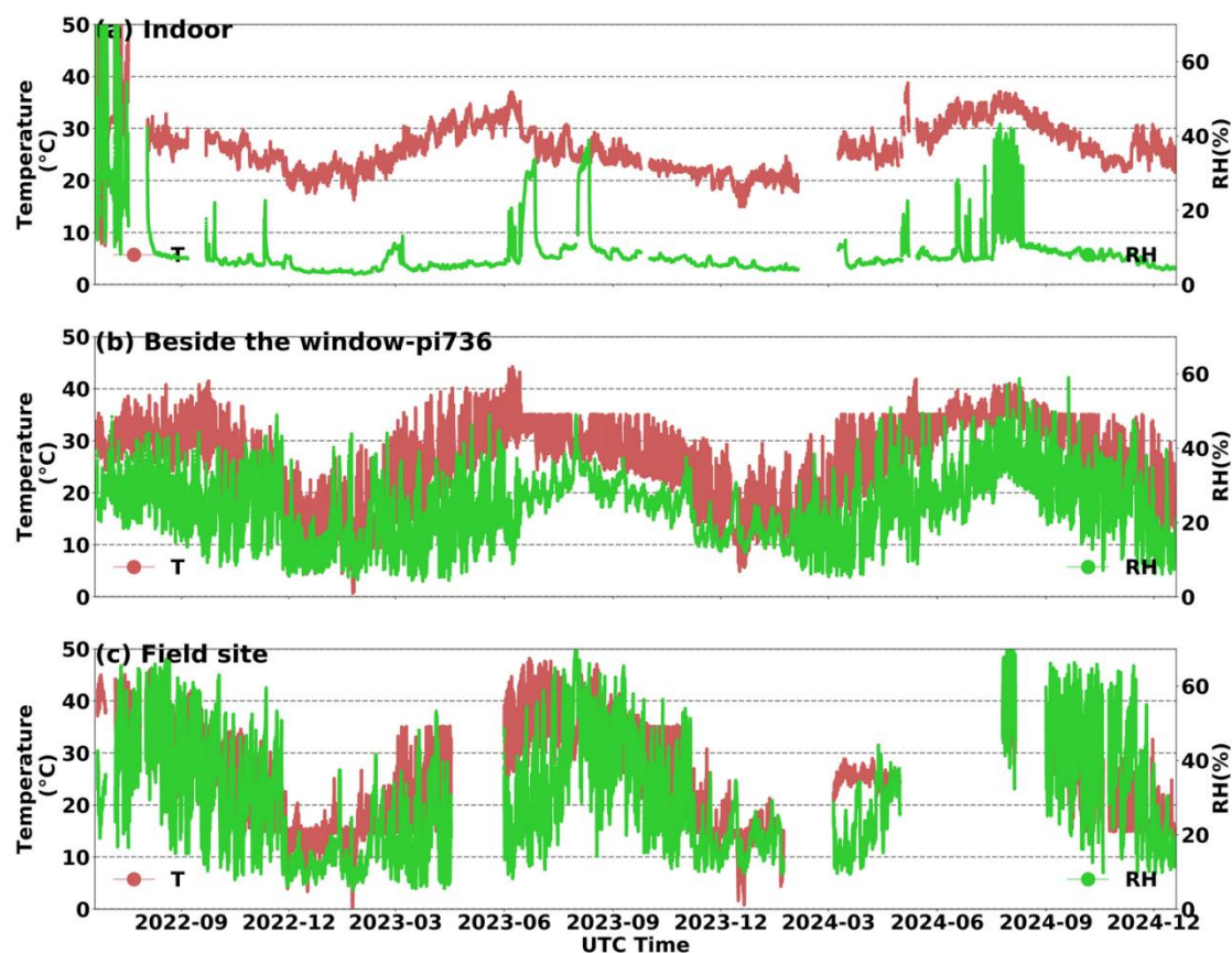
Figure 1. The temperature and humidity variation of LCS instruments under (a) indoor, (b) beside the window, and (c) field conditions during the experimental period.
