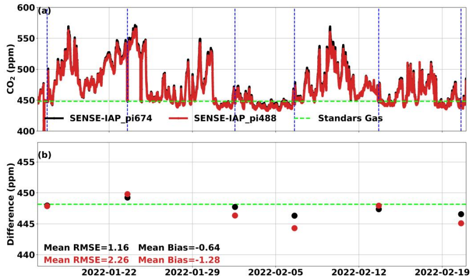
Figure 2: Comparison of CO 2 concentrations measured by SENSE-IAP and the CO 2 concentrations of standard gas at Beijing-CNEMC site in January and February 2022. (a) The time series of CO 2 per minute in the whole measurement period; the blue dashed lines mark one hour of the standard gas measurement per week, and the green dashed lines mark the concentration of standard gas. (b) The points are the hourly means of values during one hour of standard gas measurement per week, with mean biases -1.28 ~ -0.64 ppm and RMSE 1.16 ~ 2.26 ppm.
