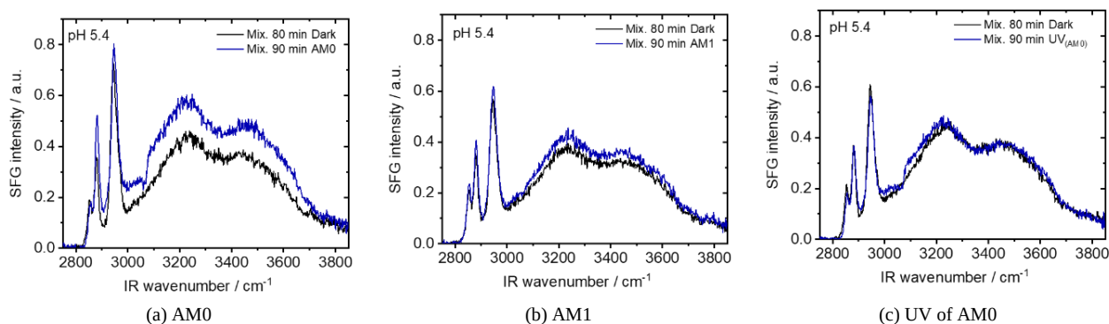
8 Figure 5: SFG spectra at air–water interface of 2 mM NA aqueous mixtures with 0.2 mM 4-BBA at a pH of 5.4, before and 9 after irradiation with (a) AM0, (b) AM1 and (c) UV portion of AM0.
