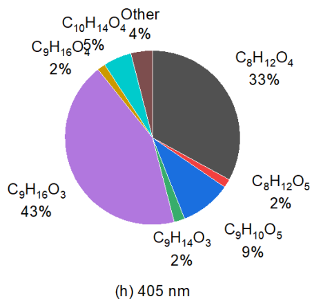
Figure 13: Fractions of products in total liquid-phase C x H y O z under different irradiation conditions. All panels represent experiments conducted in air, except panel (c), which corresponds to an experiment performed in pure nitrogen.
