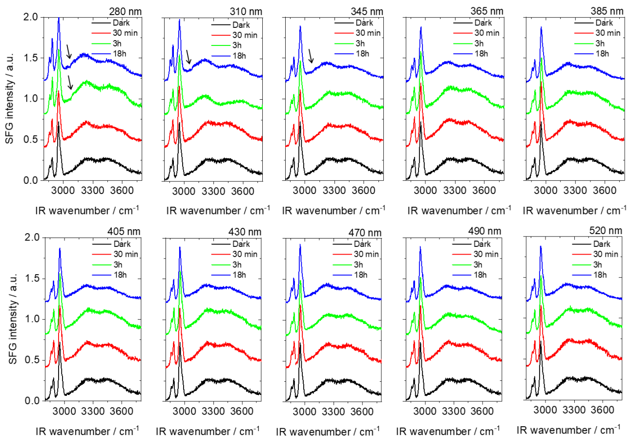
7 8 Figure 6: SFG spectra at air–water interfaces of (2 mM NA + 0.2 mM 4-BBA) mixtures at pH 5.6 after different times of 9 irradiation with different wavelengths. Note that the spectra have a constant with offset.
