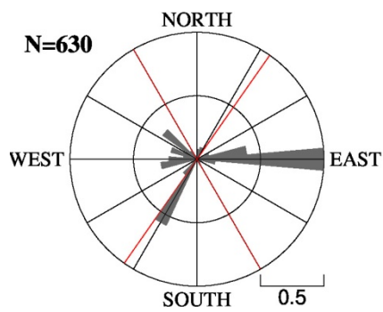
Figure 5: Rose plots of back-azimuths for (a) null and (b) non-null measurements, binned in 10° sectors. Red lines indicate the fast axis orientations of anisotropy in northern and southern Iraq. N denotes the number of measurements used to plot the rose diagrams.
