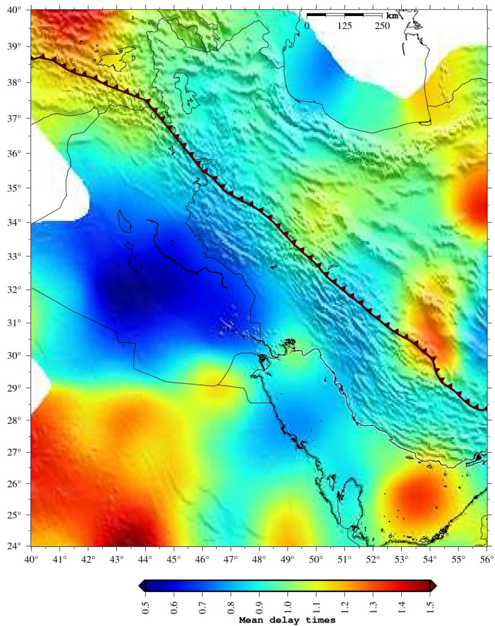
545 Figure 6: Spatial distribution of SKS splitting times across the Zagros foredeep and 546 surrounding regions, based on data from this study and previous works. The map is generated 547 by resampling the splitting times at regularly spaced 1° grid points, averaging over the 548 Fresnel zone around each point, and linearly interpolating between the grid points.
