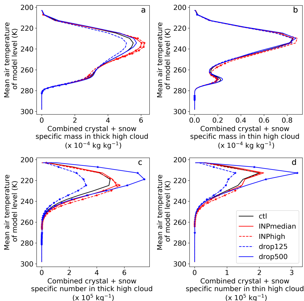
Figure 8. Combined ice crystal and snow mean in-cloud profiles for thick and thin cloud. Panels a and b are specific mass in thick and thin cloud, respectively. Panels c and d are specific number in thick and thin cloud, respectively. Scatter points denote where the mean experiment value is significantly different from the control at the 5% level using a 2-tailed, paired t-test. Equivalent figures for separate crystal and snow profiles are given in Supplementary Figures S9-10.
