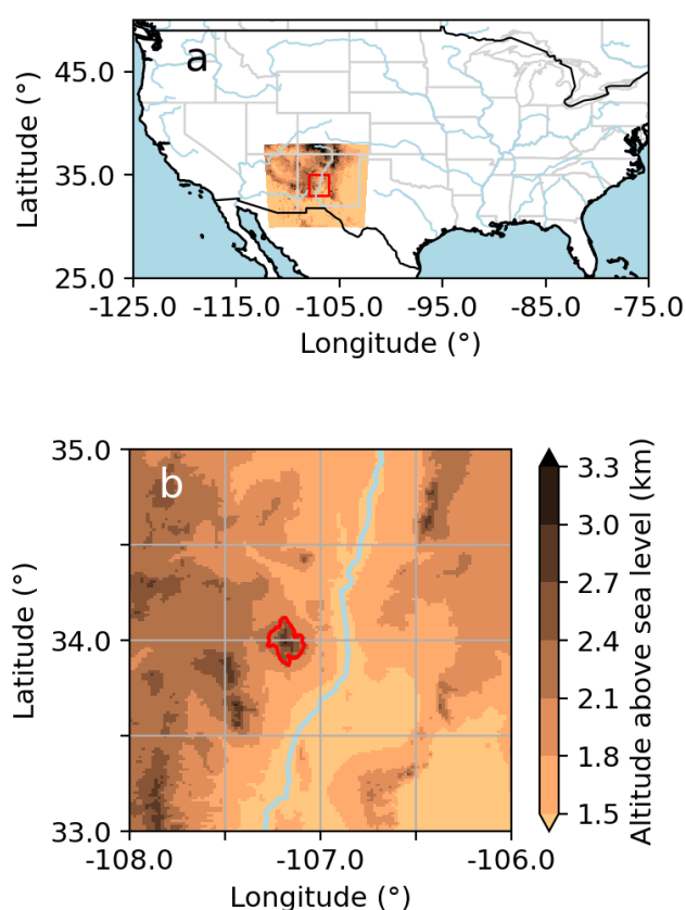
Figure 1. Model and analysis domains. Panel a shows, in the context of North America, the full model domain as the region with model orography shaded in copper colours. State and country borders are marked with grey and black lines, respectively. For analysis a 2^\circ \times 2^\circ sub-domain is used (red box in panel a), and a zoomed-in view of this domain is shown in panel b. In panel b, the 2250 m orography red contour around the Magdalena mountains is included to highlight where the DCMEX field campaign was focused. Rivers are marked in light blue, with the Rio Grande apparent running north to south through panel b.
