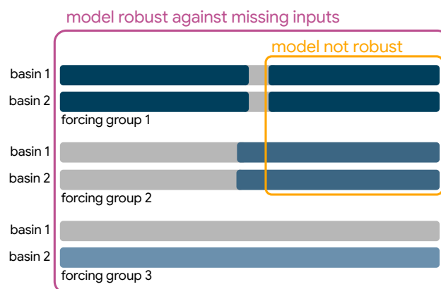
Figure 1. Different scenarios for missing input data: outages at individual time steps (top), data products starting at different points in time (middle), and local data products that are not available for all basins (bottom). All of these scenarios reduce the number of training samples for models that cannot cope with missing data (yellow, small box), while the models presented in this paper can be trained on all samples with valid targets (purple, large box).
