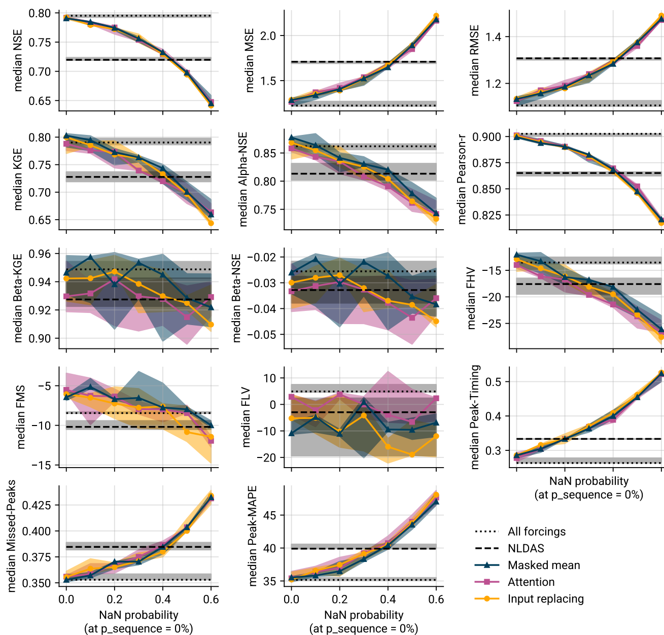
Figure C1. Extended version of Fig. 6, showing additional metrics.
