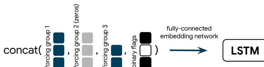
Figure 2. Illustration of the input replacing strategy. NaNs in the input data for a given time step are replaced by zeros, all forcings are concatenated, together with one binary flag for each forcing group which indicates whether that group was NaN or not. The resulting vector is passed through an embedding network to the LSTM.
