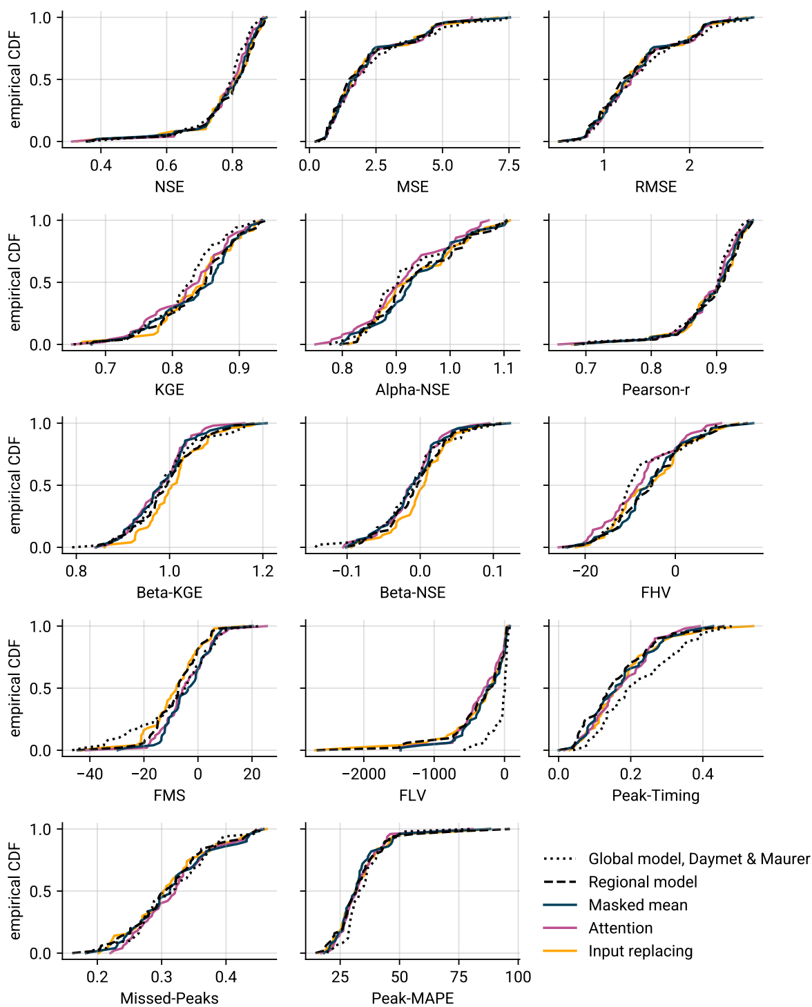
Figure C2. Extended version of Fig. 8, showing additional metrics.
