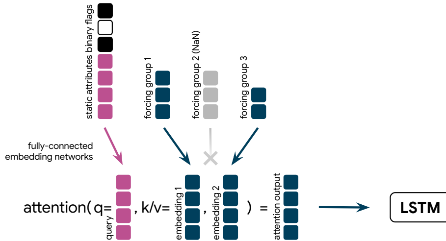
Figure 4. Illustration of the attention embedding strategy. Each forcing provider is projected to the same size through its own embedding network. The resulting embedding vectors become the keys and values. The static attributes, together with a binary flag for each provider, serve as the query. The attention-weighted average of embeddings is passed on to the LSTM.
