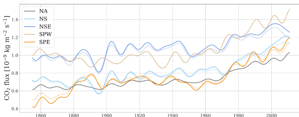
Figure 2: Decadal variability in the simulated \text{CO}_2 flux ( F , solid line) and calculated flux ( F_{\text{calc}} , dotted line) for ensemble member r4i1p1f1. Here the weighted mean is shown to compare the fluxes and variability across regions. F_{\text{calc}} only showed for NS, NSE, SPE
