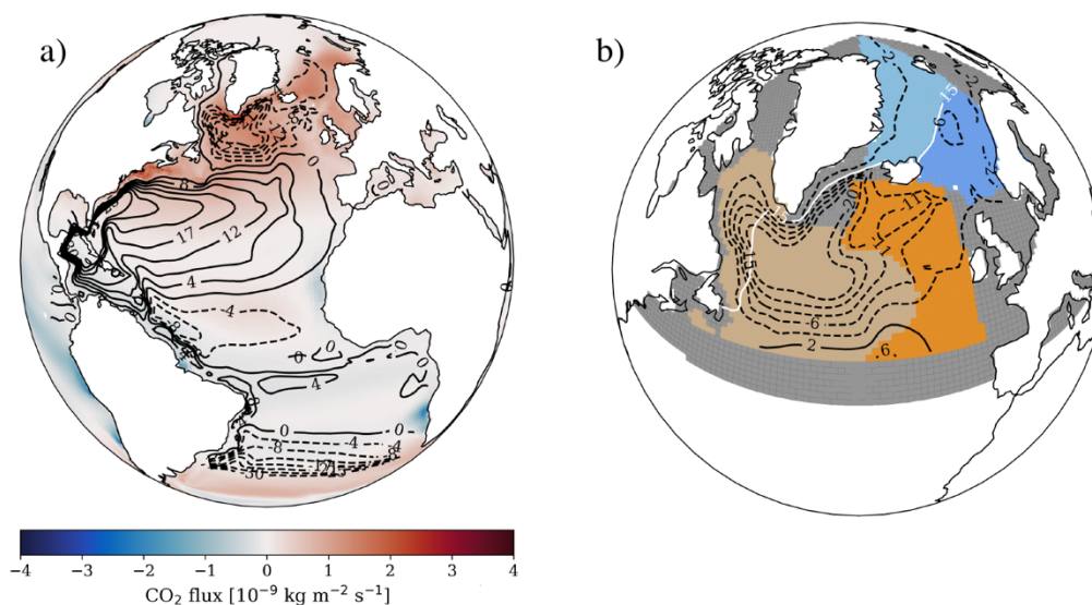
Figure 1: a) Atmosphere–ocean CO 2 flux averaged over the period 1982-2014 for EC-Earth3-CC. Black lines show the mean barotropic streamfunction of the SPG circulation of ten ensemble members in Sv. Full line indicating a positive values, dashed line indicating negative values. Closed dashed lines show the mean extent of the SPG. b) showing the study regions: NA covering all regions (dark grey) SPW (beige), SPE (orange), NSE (blue), NS covering NSE as well (light blue), global average 15% SIC line (white contour) indicating the boundary between sea ice covered regions and sea ice free areas.
