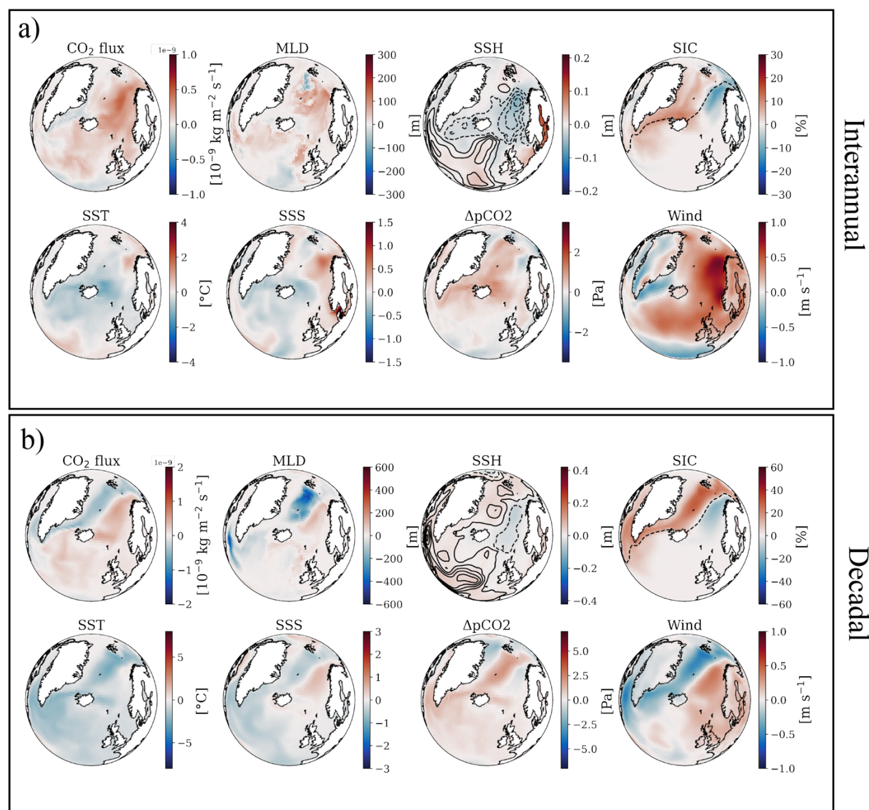
315 Figure 5 Anomalies of the high-low years of the dynamic parameters compared to the CO 2 flux anomaly in the NSE. a) showing interannual timescale and b) showing decadal timescale. Full and dashed lines on top of the SSH anomaly shows the barotropic mass streamfunction anomaly and dashed line on top of SIC anomaly shows the 15% SIC climatology (mean of ten ensemble members on both timescales).
