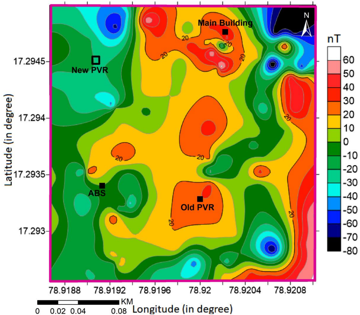
100 101 Figure 2: Magnetic anomaly plot of the survey region in 2012. Black box is the marked 102 location for the New PVR, built in 2019-2020. 103
