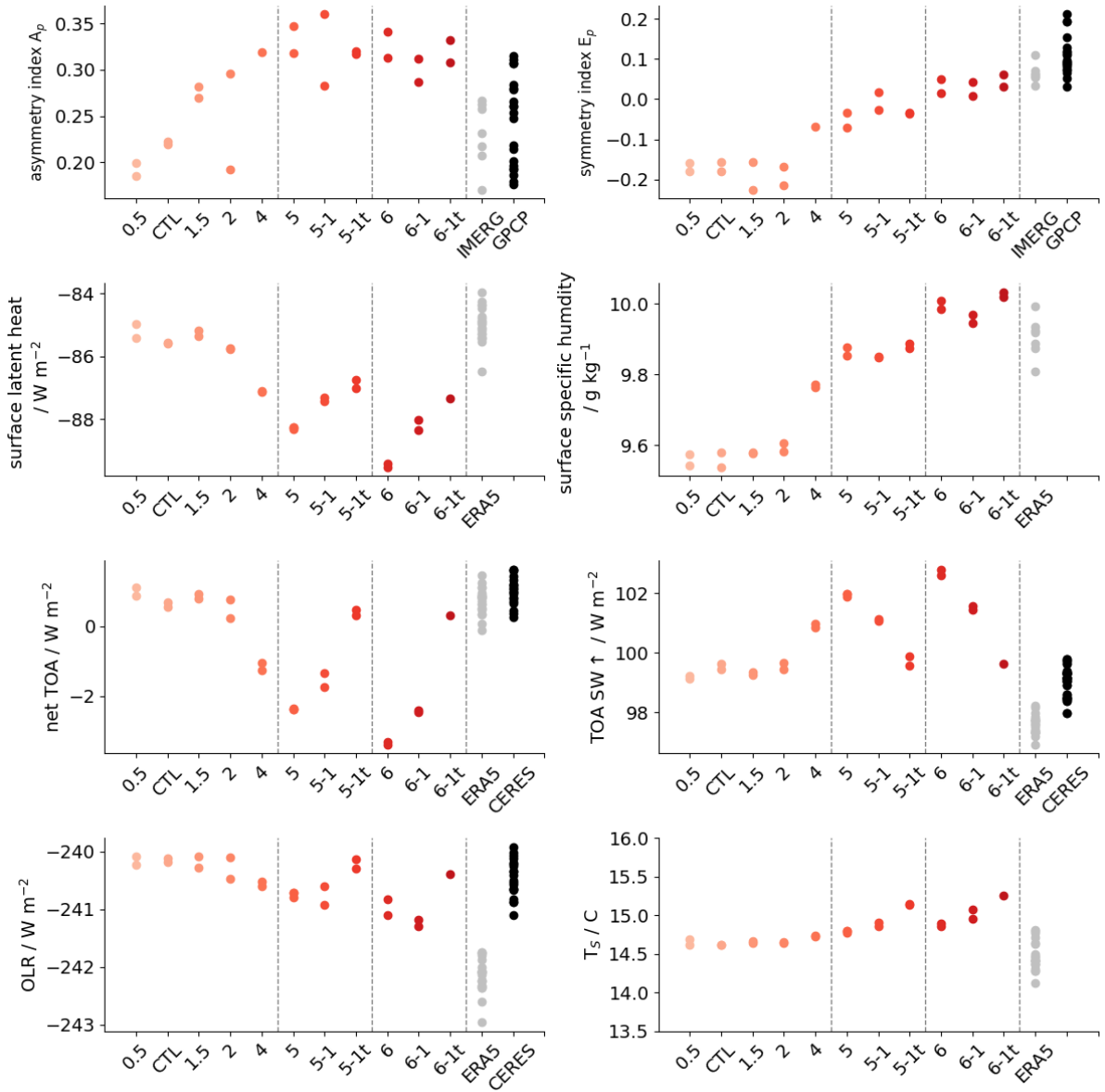
Figure 10. Simulation scores for all 40 km sensitivity experiments as a function of prescribed minimum surface wind speed. The values for a U_{min} of 1 \text{ m s}^{-1} were taken from the respective two years of the CTL simulation. Values for the asymmetric index A_p , symmetry index E_p as well as latent heat flux, near-surface specific humidity q_s , net top-of-the-atmosphere (TOA) imbalance, upwards radiative shortwave flux, outgoing long wave radiation (OLR) and global mean surface temperature T_s are shown. Each point depicts a one-year global average. For reference the corresponding values from IMERG, GPCP, ERA5 and CERES are depicted.
