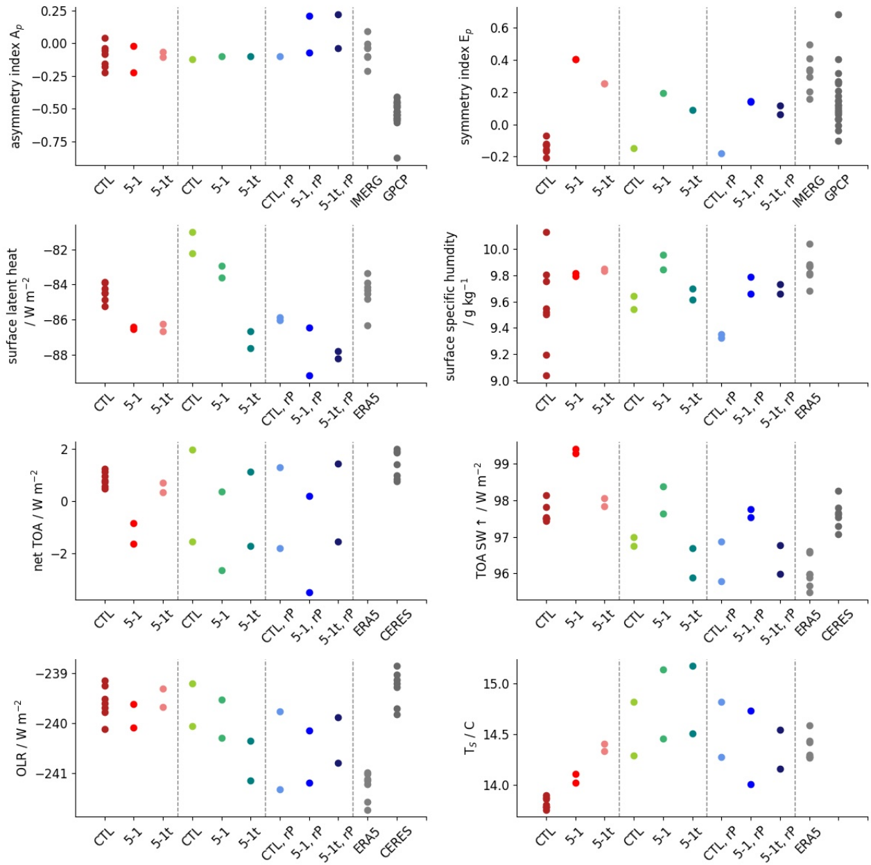
Figure 14. Simulation scores for two MAM seasons of CTL, PTB-5_1 and PTB-5_1t sensitivity experiments in the 40 km, 5 km and 5 km-rParam setup. The 40 km scores are shown in different shades of red, the 5 km setups in shades of green and the 5 km-rParam in different shades of blue. Values for the asymmetric index A_p , symmetry index E_p as well as latent heat flux, near-surface specific humidity q_s , net top-of-the-atmosphere (TOA) imbalance, upwards radiative shortwave flux, outgoing long wave radiation (OLR) and global mean near-surface temperature T_s are shown. Each point depicts a one season average. For reference the corresponding values from IMERG, GPCP, ERA5 and CERES are listed.
