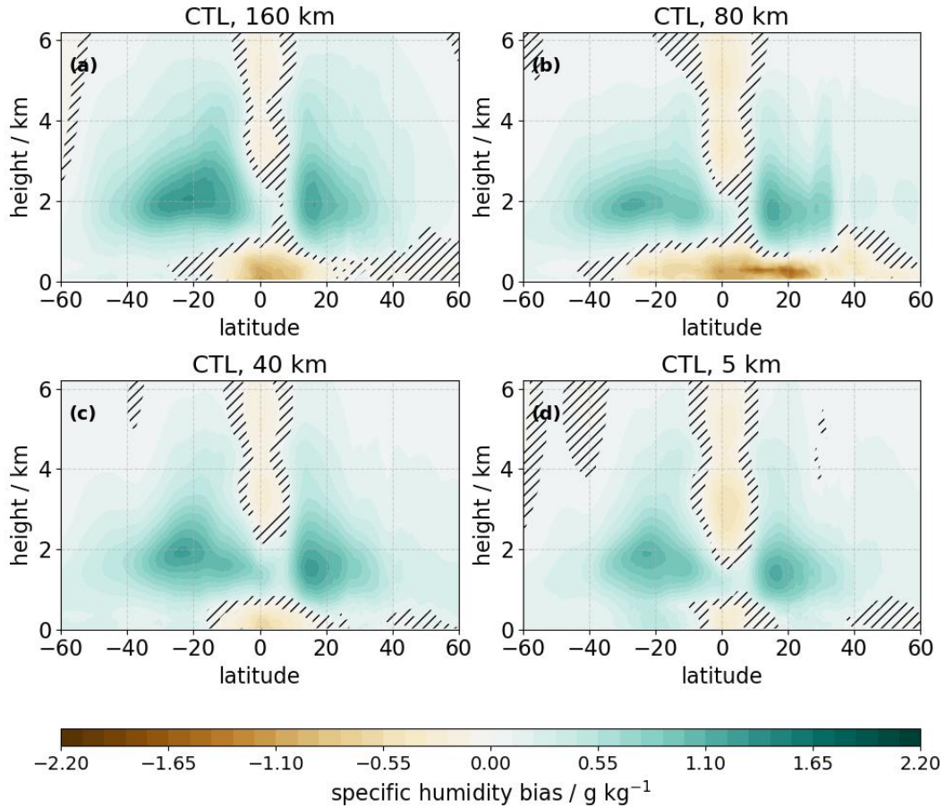
Figure 3. (a)-(d) Two-year atmospheric specific humidity bias with respect to ERA5 (2004-2010) for 160 km (a), 80 km (b), 40 km (c) and 5 km setups (d). Statistically significant differences between ERA5 and the model data are shown, and insignificant regions are dashed out.
