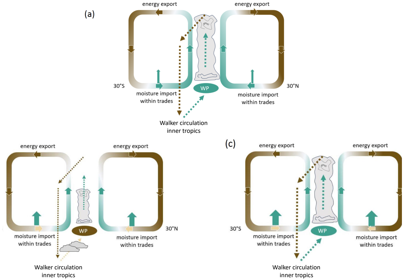
Figure 1. Conceptual depiction of the main zonal and meridional circulations exchanging moisture and energy between the subtropics and the tropics as a) observed, b) in default ICON simulations, and c) in U_{min} adjusted ICON simulations. Observations show that the moisture within the innermost tropics originates from evaporation in tropical and subtropical areas. The moisture is imported into the innermost tropics by the trade winds, with small losses to the free troposphere. In the innermost tropics it is then transported to the main convective regions, i.e., the Warm Pool (WP) within the zonally anomalous Walker circulation. Energy is exported to the subtropics within the outward branches of the Hadley circulation. In conventional ICON simulations (b), a large portion of the subtropical moisture is lost due to too much vertical transport of moisture from the boundary layer to the free troposphere. This leads to a moisture deficit in the tropics, specifically over the WP, reducing deep convection, slowing down the Walker circulation and leading to spurious additional convective centers over the Eastern Pacific as too little moisture is transported to the WP within the boundary layer. In the U_{min} adjusted ICON simulations (c) increased evaporation leads to an additional moisture source in the tropics, which resolves the dry bias over the WP. However, the adjustments increase the positive free-tropospheric moisture bias between 0^{\circ} to 30^{\circ} , reduce the trade wind strength and change the balance between innermost-tropical and subtropical sources of tropical moisture content. Green colors indicate high moisture content. Brown colors low moisture content.
