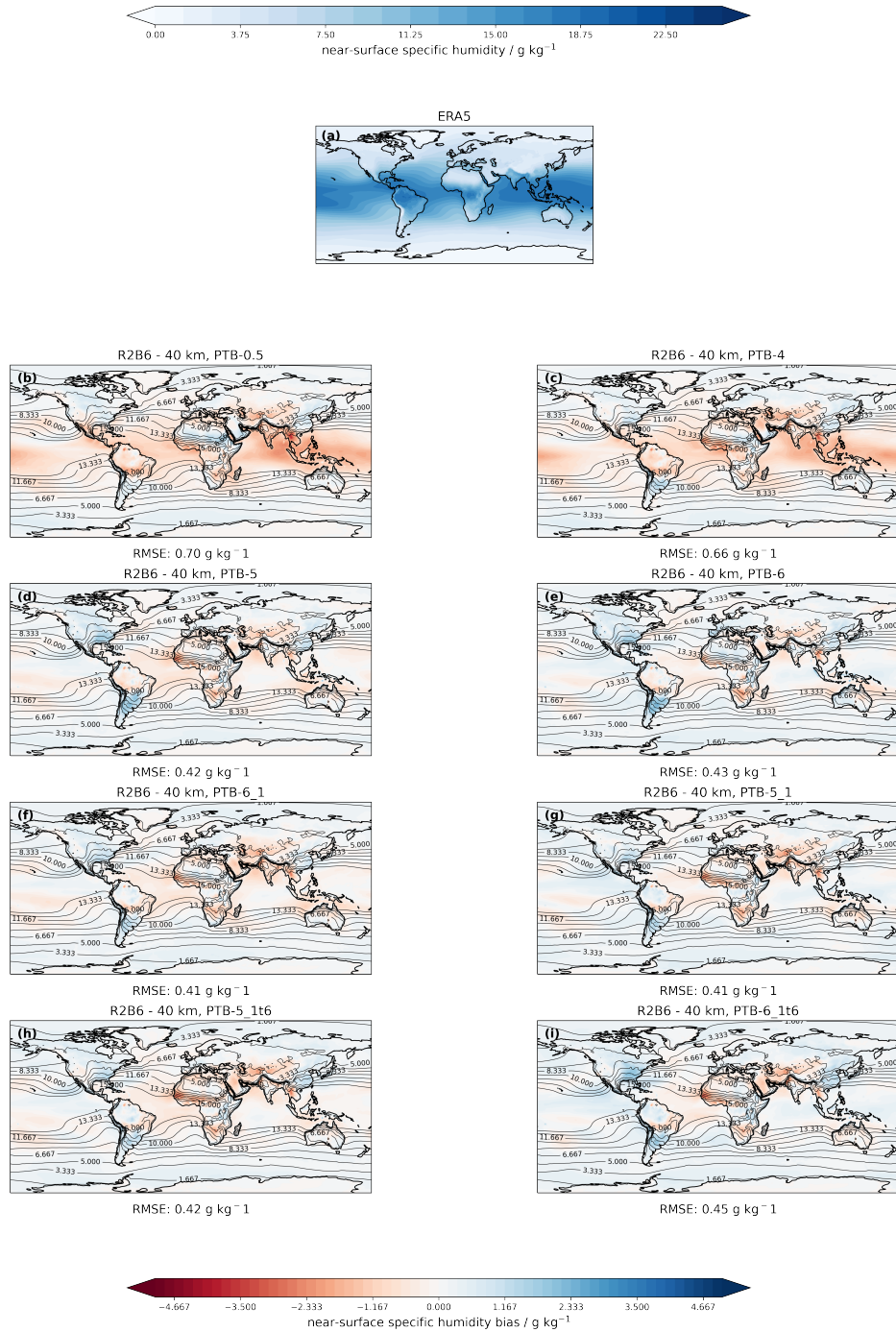
Figure C2. Two-year mean large-scale surface humidity bias with respect to ERA5 (2004-2010) for different settings of the surface wind in 40 km: : PTB-0.5, PTB-4, PTB-5, PTB-5_1, PTB-5_1t, PTB-6, PTB-6_1 and PTB-6_1t. Contours show the ERA5 climatology. The corresponding global RMSE is stated beneath the panel for each sensitivity experiment.
