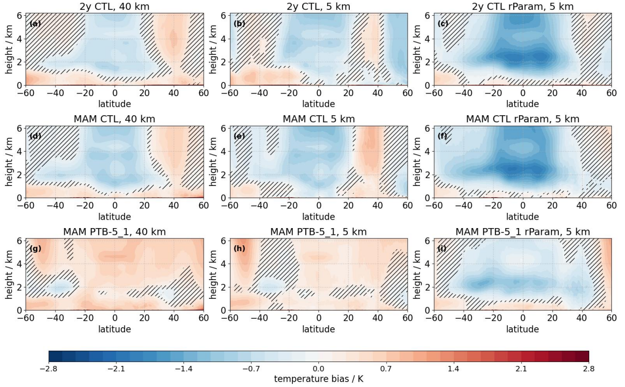
Figure 13. Zonal mean temperature bias with respect to ERA5: all CTL for a 2 year average (a-c), all CTL for an average over two MAM seasons (d-f) and all PTB-5_1 for an average over two MAM seasons (g-i) for 40 km, 5 km and 5 km-rParam. Statistically significant differences between ERA5 and the model data are shown, insignificant regions are hatched.
