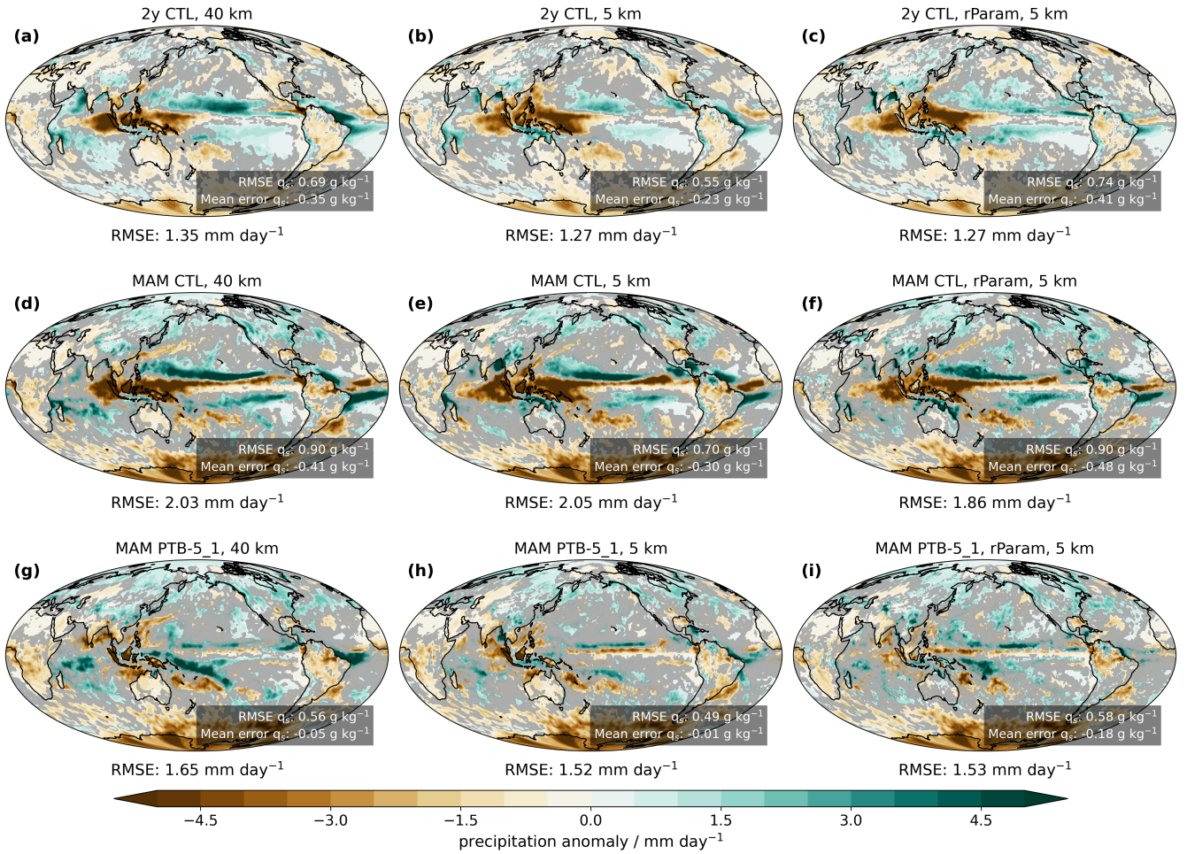
Figure 11. Large-scale precipitation bias with respect to IMERG in: 2-yr averages from CTL simulations (a-c), two-MAM averages from CTL simulations (d-f) and two-MAM averages from PTB-5_1 simulations (g-i) for 40 km, 5 km and 5 km-rParam. The corresponding global precipitation RMSE is indicated below the panel for each experiment. Statistically insignificant differences between IMERG and the experiments are shown based on a two-sided z-test at \alpha = 0.1 , and insignificant regions are grayed out. The global RMSE and mean error in the near-surface specific humidity, calculated with respect to the values derived from the ERA5 reanalysis, are shown in the inlays.
