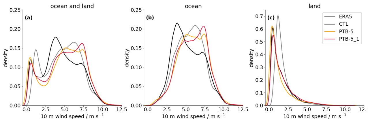
Figure 6. Normalized probability density functions of the monthly mean near-surface wind speed distributions between 10^\circ \text{ S} to 10^\circ \text{ N} in the experiments CTL, PTB-5 and PTB-5_1. A comparison with ERA5 data is given for (a) the entire region, (b) over ocean only, and (c) over land only.
