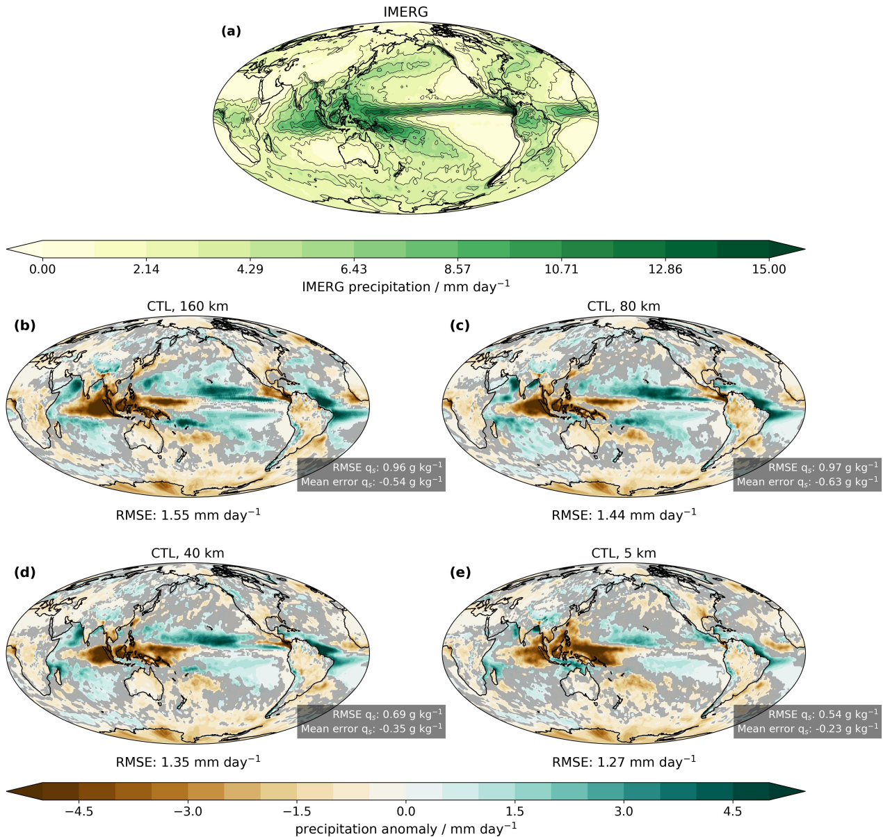
Figure 2. (a) Climatological IMERG precipitation distribution from 2004 to 2010 and (b)-(e) two-year mean precipitation bias with respect to IMERG for 160 km (b), 80 km (c), 40 km (d) and 5 km (e) setups. Statistically insignificant differences between IMERG and the experiments based on a two sided z-test at \alpha=0.1 are grayed out in (b)-(e). The corresponding global RMSE in precipitation is stated beneath the panel for each resolution experiment. The global RMSE and mean error in near-surface specific humidity, calculated with respect to values derived from ERA5 reanalysis, is depicted in the inlays.
