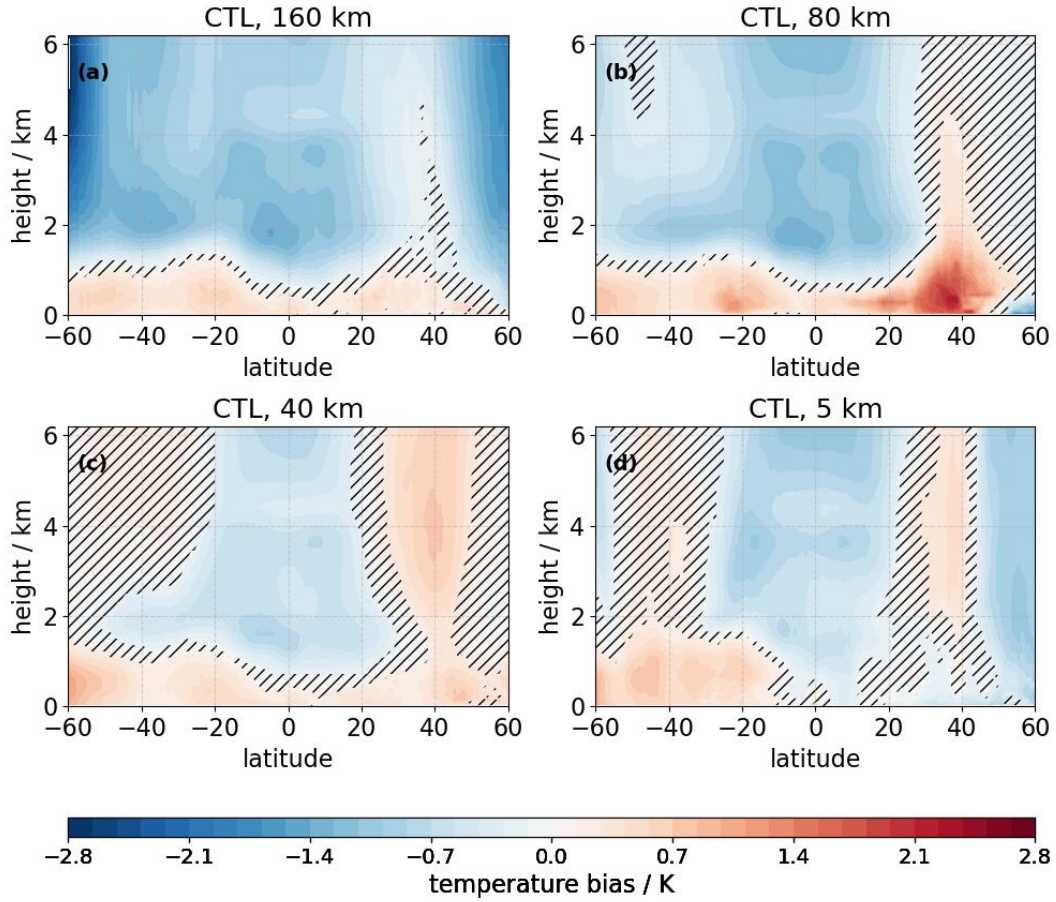
Figure 4. (a)-(d) Two-year atmospheric temperature bias with respect to ERA5 (2004 to 2010) for 160 km (a), 80 km (b), 40 km (c) and 5 km (d) setups. Statistically significant differences between ERA5 and the model data are shown, insignificant regions are dashed out.
