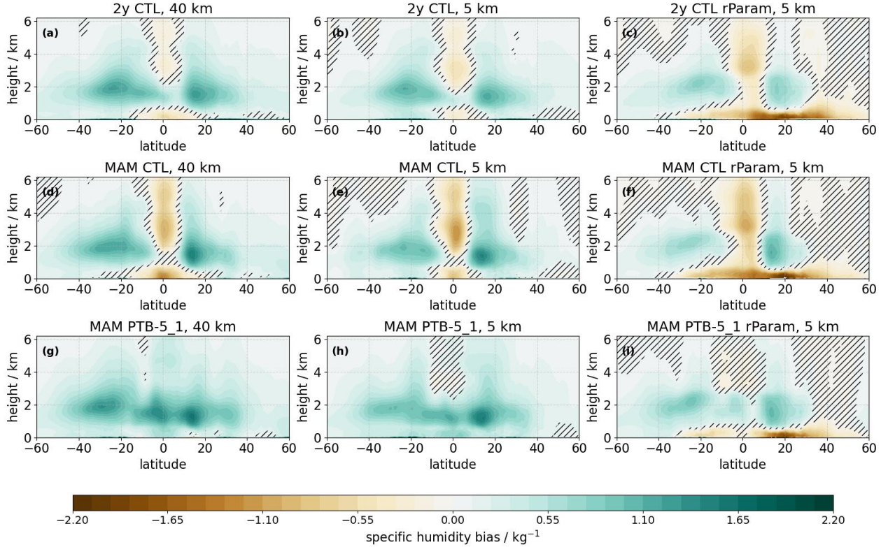
Figure 12. Atmospheric specific humidity bias with respect to ERA5: all CTL for a 2 year average (a-c), all CTL for an average over two MAM seasons (d-f) and all PTB-5_1 for an average over two MAM seasons (g-i) for 40 km, 5 km and 5 km-rParam. Statistically significant differences between ERA5 and the model data are shown, insignificant regions are hatched.
