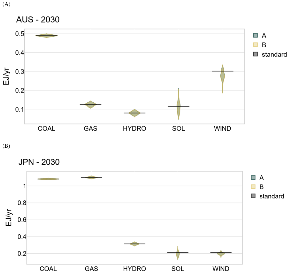
Figure 8 Electricity generation by fuel (distribution) in Australia (AUS) and Japan (JPN) in 2030, downscaled from the MESSAGE current policy scenario. We have run two simulations (A and B), each of them with completely independent ( n=500 ) randomly generated electricity criteria. The distribution of the results is depicted in light blue (A) and yellow (B) from the two sets of randomly
