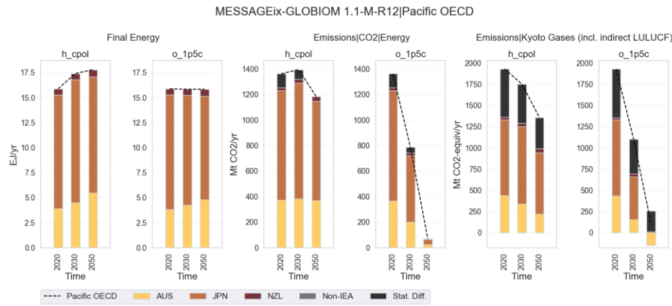
820 Figure 4 Downscaled results from the Sub-Saharan Africa (a), China (b), Western Europe (c) and Pacific OECD (d) regions of the MESSAGE model, under a Current policy and 1.5°C scenarios. Selected variables: Final Energy, Energy related CO 2 emissions and Kyoto Gases (including indirect LULUCF).
