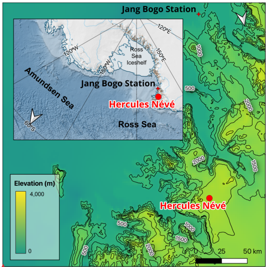
1240 Figure 1 (A) Map of the West and East Antarctica regions showing the Ross Ice Shelf, the Ross Sea, and Hercules N  v  . (B) Topographic map of Northern Victoria Land. The red circles indicate the location of the Hercules N  v   ice core. The maps were created using Quantarctica 3.2 on QGIS.
