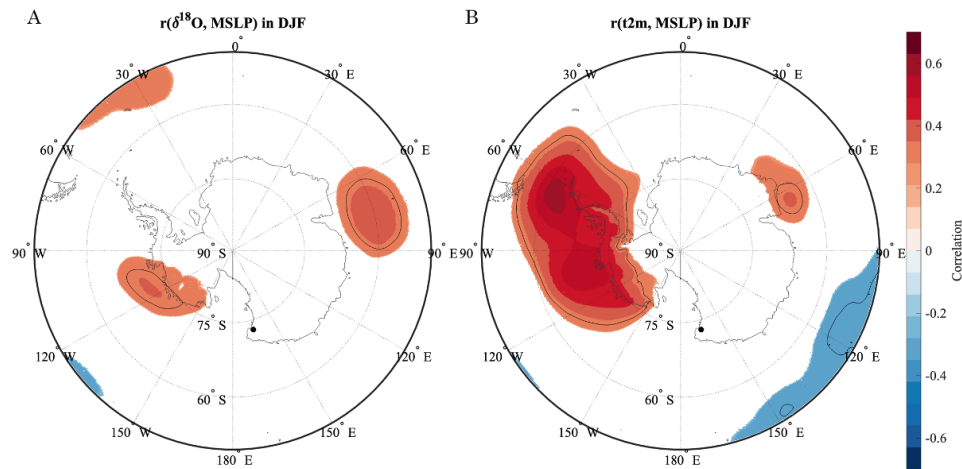
Figure 5: Spatial correlation analysis for (A) \delta^{18}\text{O} from the HN ice core (black symbol) and (B) the 2 m temperature (t2m) from ERA5 data with the mean sea level pressure (MSLP) from 1979 to 2015 in DJF. Contour plots are used for p < 0.05 and black lines for p < 0.01 .
