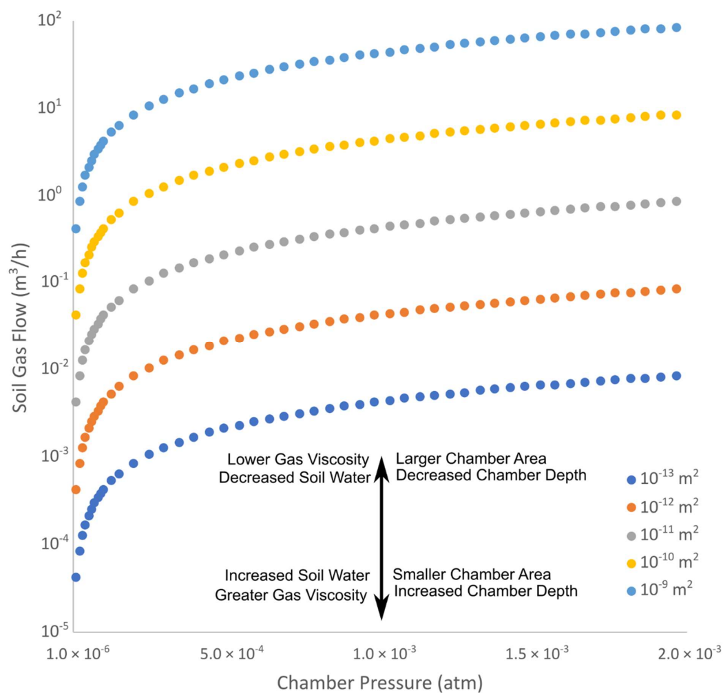
Figure 9: Gas flow through different soil permeabilities ( 10^{-9} to 10^{-13} \text{m}^2 ) as a function of chamber pressure. The arrows show how changes in conditions affect soil gas flow at a given chamber pressure.
