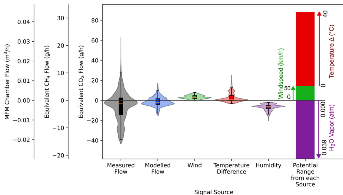
Figure 11: Violin and box plots showing the range and distribution of measured chamber flow (black) with modelled chamber flow from equation 4 (blue), and contributions to the modelled flow from wind (green), temperature difference between inside the chamber and outside (red), and humidity of the gas at the mass flow meter (MFM) vent (purple). On the right, the range of potential contributions for the different environmental components is shown as stacked bars with arrows showing the potential contribution from each environmental factor. Temperature differences and wind increase measured flow, while increasing water vapor in the chamber causes the signal in the MFM to decrease. The left axis is plotted both in terms of volumetric gas flow through the MFM (corrected to 25 °C and 1 atmosphere) as well as emission rates of methane and carbon dioxide.
