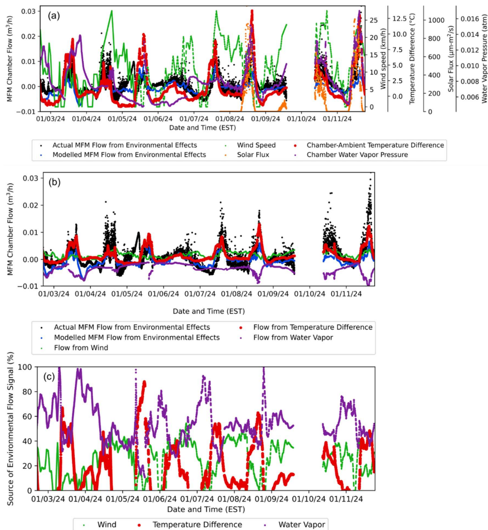
Figure 10: Analysis of the gas flow through the mass flow meter (MFM) chamber from environmental processes (a) Test chamber environmental flow measurements along with wind speed, temperature difference, solar flux, water vapor pressure, and modelled environmental flow. (b) The measured and predicted environmental flow along with the contribution to the MFM signal from wind, temperature difference, and water vapor pressure. (c) The relative proportion of the environmental flow from each factor (wind, temperature difference, and water vapor pressure) calculated at the time of each measurement. The collected on 1/10/2024 are omitted because the humidity sensor stopped working.
