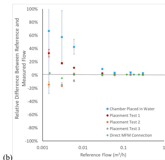
Figure 7: Comparison of the references gas flow rates into the chamber and the measured flow rates out of the chamber mass flow meter (MFM) under the direction connection, chamber in water, and replicate (3x) 18 cm placement scenarios. (a) Measurements and linear regression of the reference and measured flows (b) The difference between the reference flow (MFC) and the measured flow (MFM) as a function of reference flow rate, showing that the error in flow rates becomes much greater below 1 \times 10^{-2} \text{ m}^3/\text{h} .
