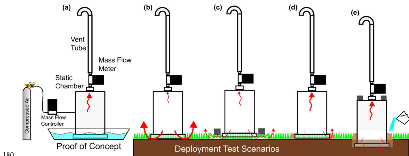
185 Figure 4: Diagram of flow test scenarios. (a) chamber in water bath to validate performance with perfect base seal and no leaks. (b) chamber on ground surface (c) chamber sealed to ground with weighted polyethylene skirt (d) chamber on ground surface sealed with dirt, (e) chamber buried at various depth and sealed with dirt and added water to improve soil compaction and ground seal formation. Grey squares are weights to hold the chamber down. Arrow widths denoted the relative amount of gas flows through different paths.
